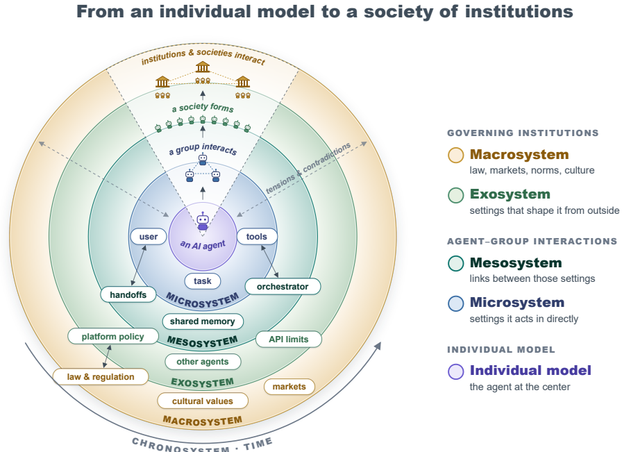
Fig. 1. Nested systems around interacting agents, after Bronfenbrenner [16]. An AI agent sits at the center, inside the settings it acts in (microsystem) and the links between them (mesosystem)—together, agent-group interactions—and inside the platform, market, and legal institutions that govern it from outside (exosystem and macrosystem). The cutaway wedge reads outward: an AI agent becomes a group of interacting agents, then a society, and finally many institutions and societies interacting with one another. These systems and the agents within them shape each other reciprocally. Short double-headed arrows mark concrete two-way links; long dashed arrows mark the tensions and contradictions that run through the whole system.
