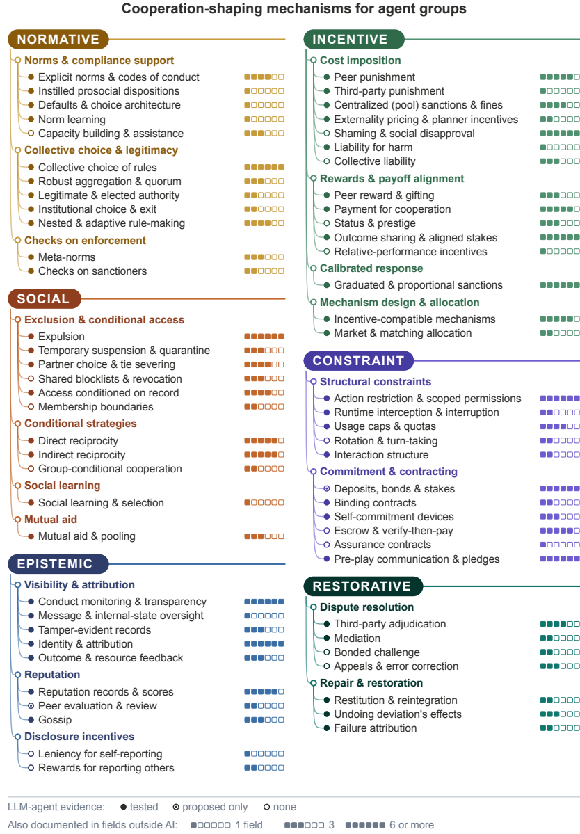
Fig. 5. Cooperation-shaping mechanisms for agent groups: 66 mechanisms in 18 themes, thematically coded from 645 instances across AI and 18 other disciplines (Section 3; Appendix A) and grouped by the six mechanism families. Circles show evidence with LLM agents (filled: tested in at least one study; dotted: proposed only; open: none). Squares count the fields outside AI in which a mechanism is also documented; six filled squares means six or more. An interactive version, with links to every source, is at https://van-truong.github.io/institutional-design-for-ai-agents/ .
