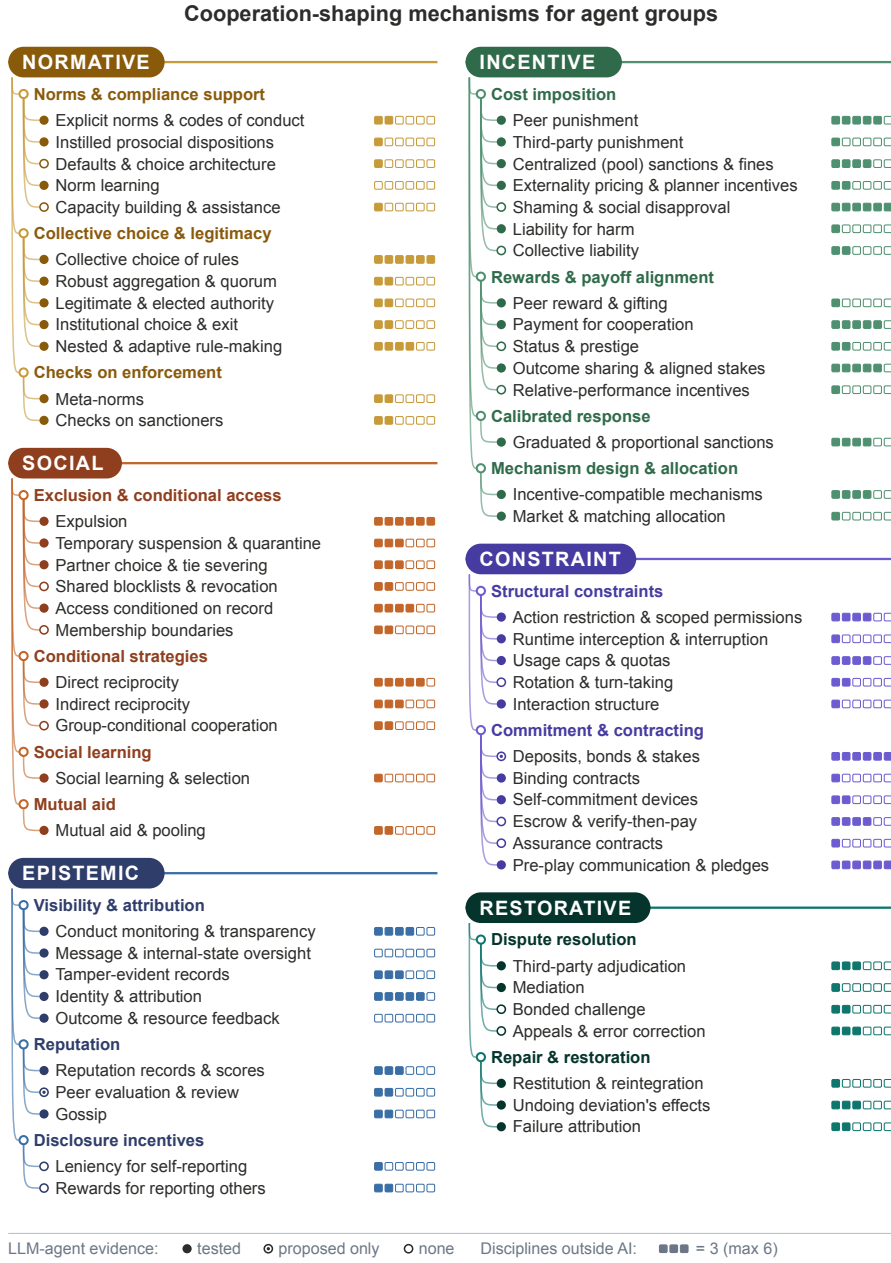
Fig. 4. Cooperation-shaping mechanisms for agent groups: 66 mechanisms in 18 themes, coded from 561 instances across AI and 18 other disciplines (Appendix A) and grouped by the six mechanism families. Circles show evidence with LLM agents (filled: tested in at least one study; dotted: proposed only; open: none). Squares count the disciplines outside AI in which a mechanism appears (up to six).
