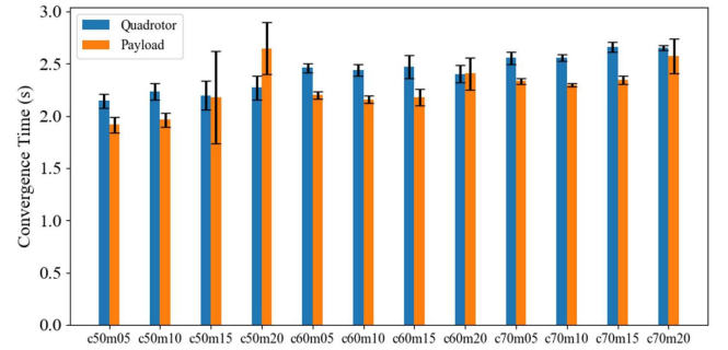
Fig. 13. Convergence time for stable hovering of different combinations of cable lengths and payload masses. In the figure, we visualize the convergence time for stable hovering at the target position across 12 combinations of three cable lengths and four payload masses. The blue bars represent the quadrotor's convergence time, while the orange bars represent the payload's convergence time. The x-axis corresponds to these different combinations, and the y-axis represents the convergence time in seconds.
