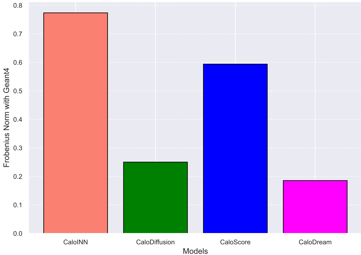
Frobenius Norm Comparison with Geant4 for group wise correlation
