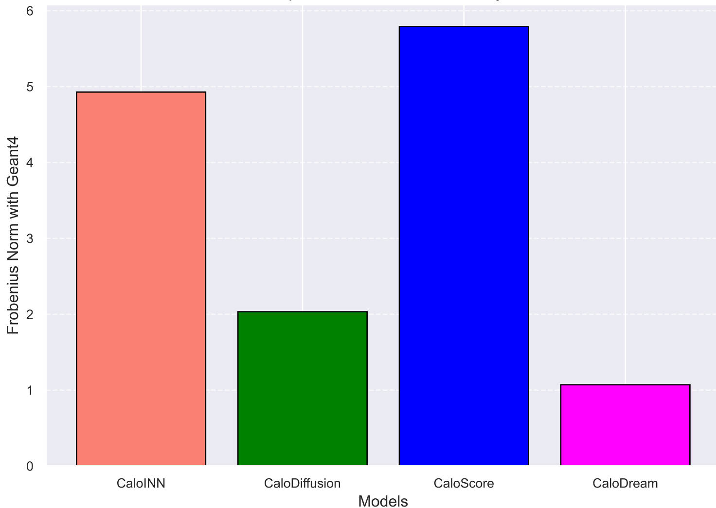
Frobenius Norm Comparison with Geant4 for layer wise correlation
