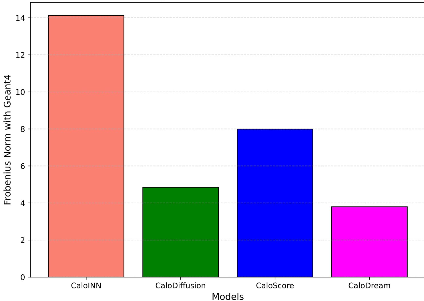
Frobenius Norm Comparison with Geant4 for voxel wise correlation
