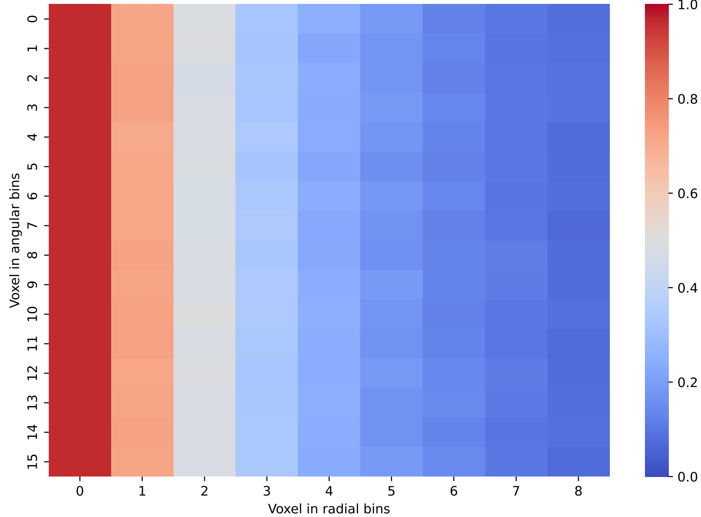
Geant4 Data: Layer 9 and 10
