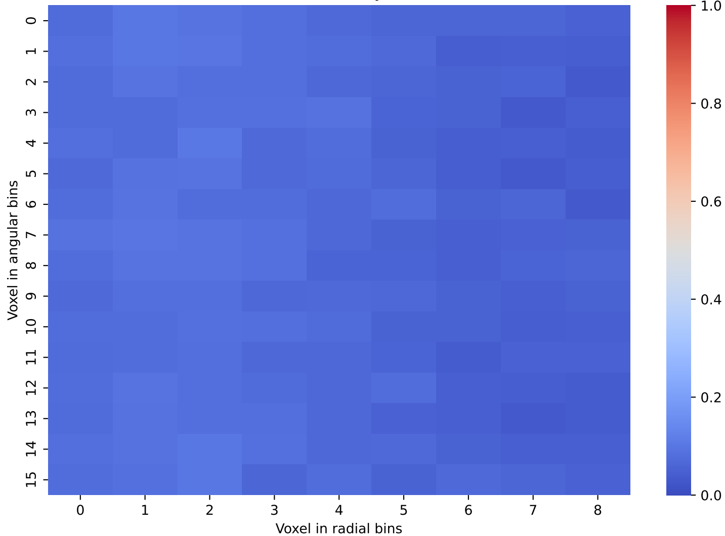
CaloDREAM Data: Layer 1 and 2
