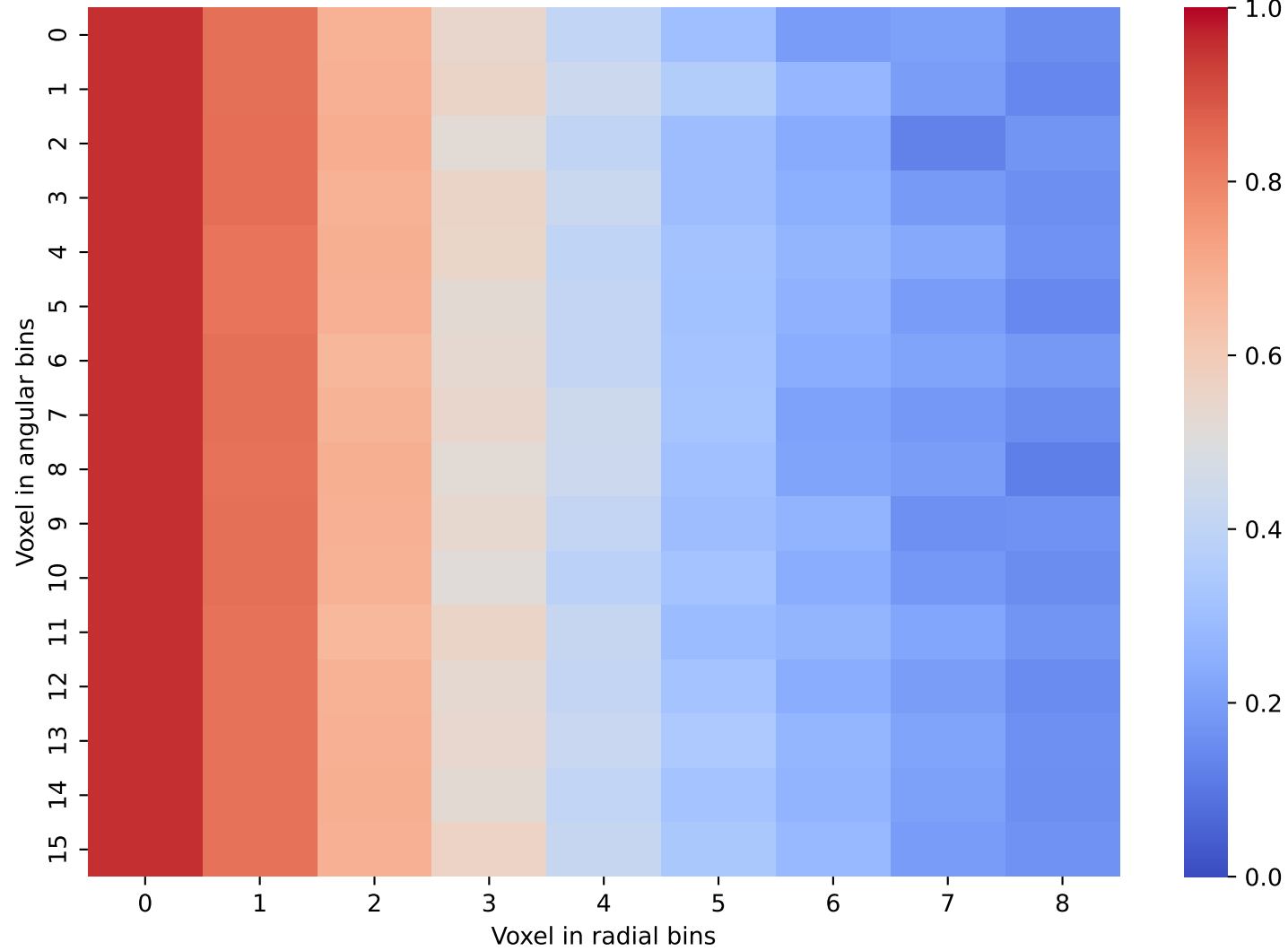
CaloDream Data: Layer 21 and 22
