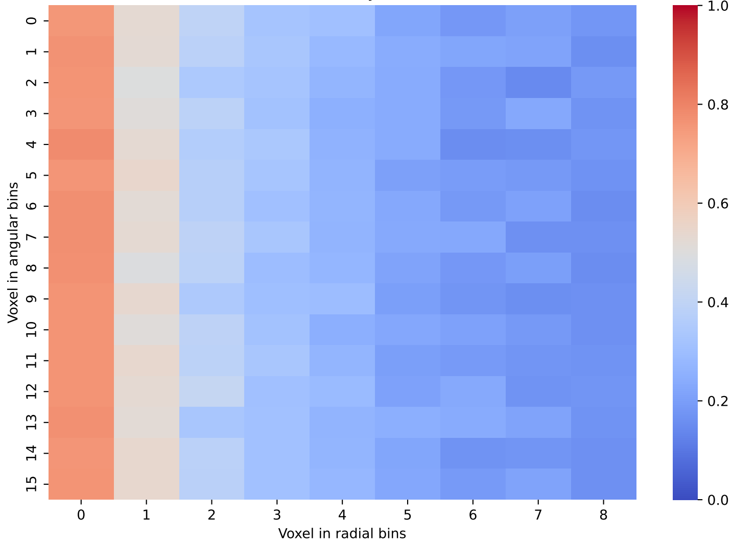
CaloDream Data: Layer 31 and 32
