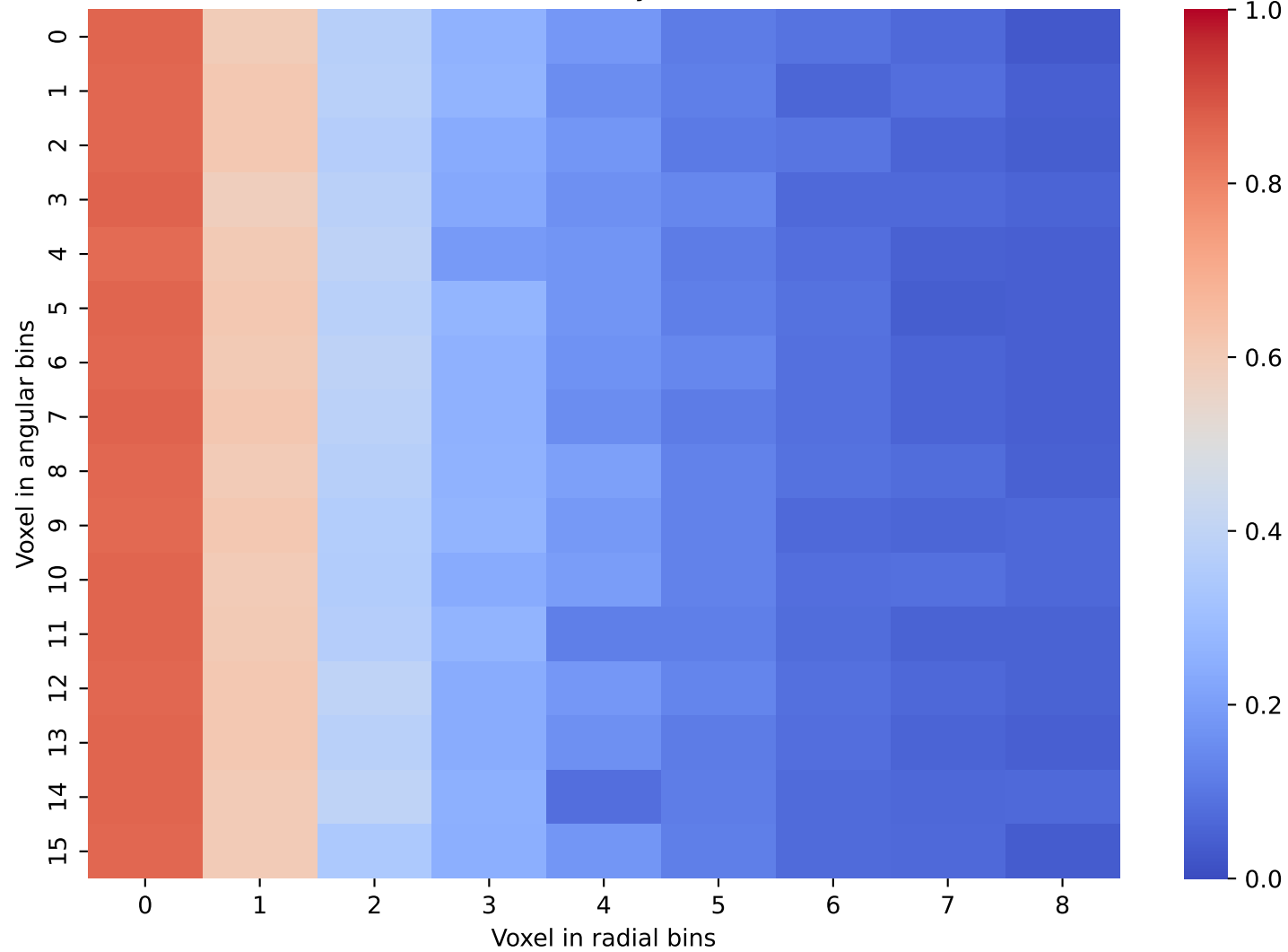
CaloINN Data: Layer 9 and 10
