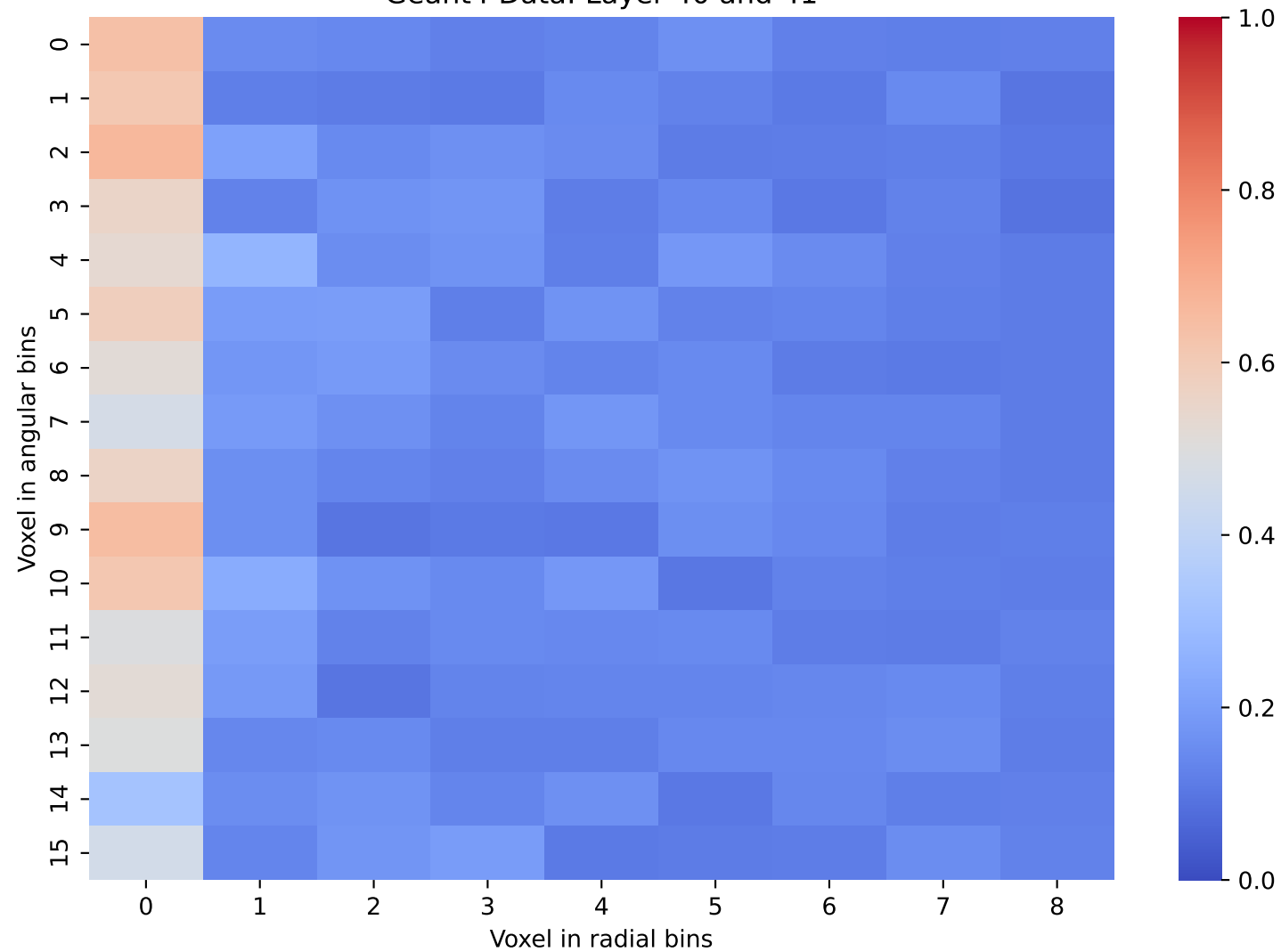
Geant4 Data: Layer 40 and 41
