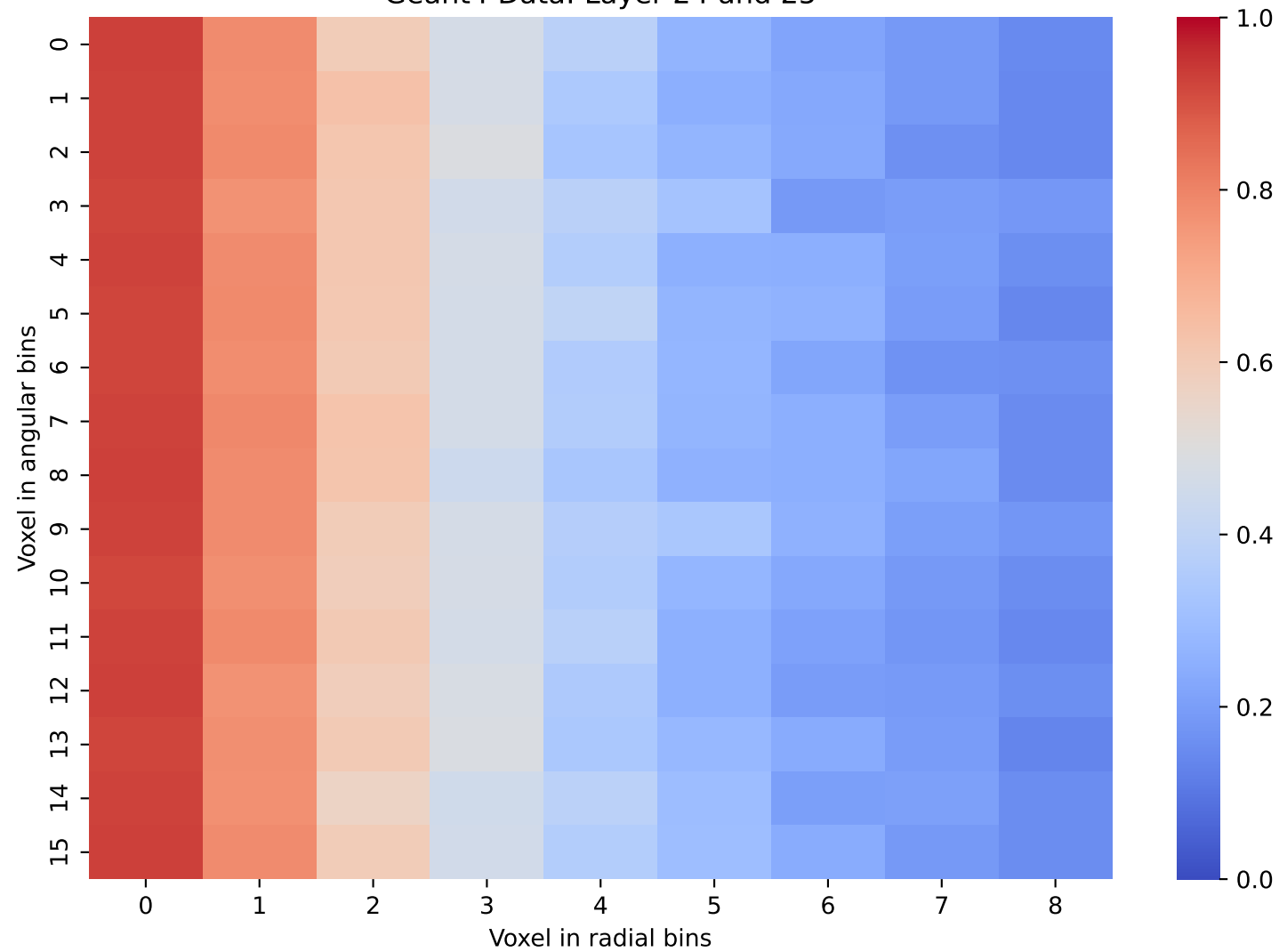
Geant4 Data: Layer 24 and 25
