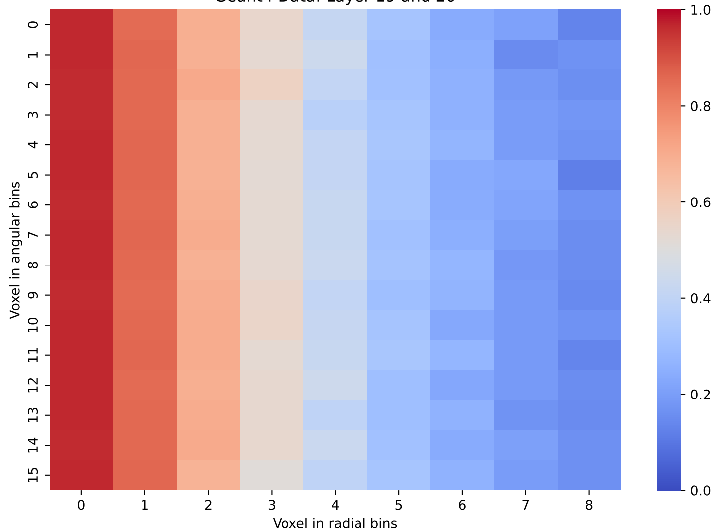
Geant4 Data: Layer 19 and 20
