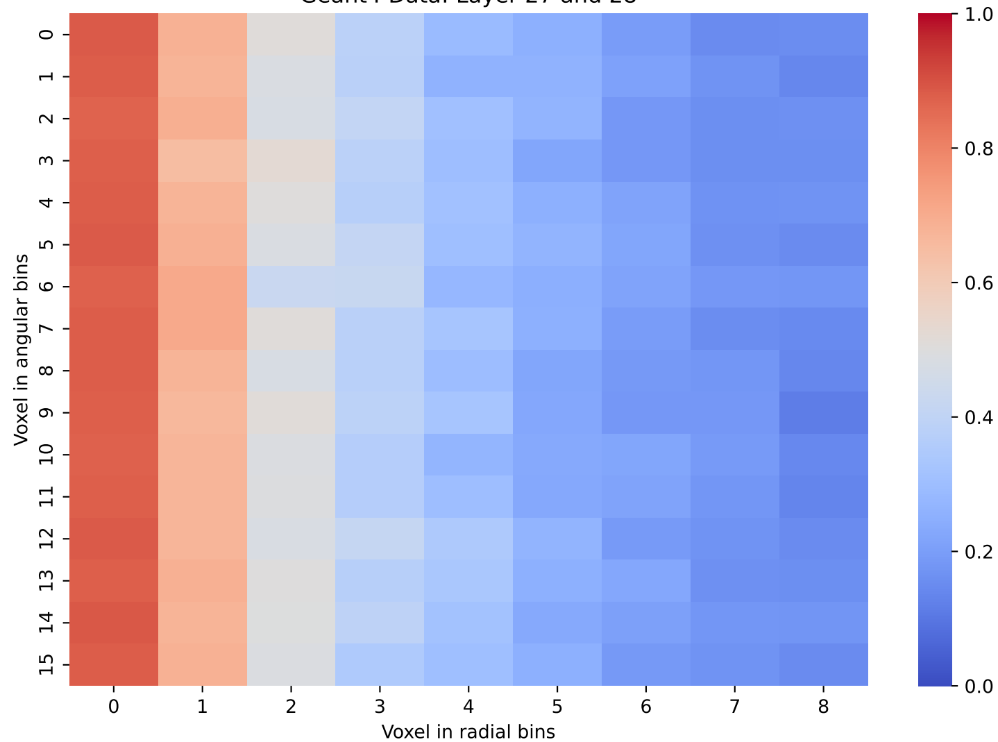
Geant4 Data: Layer 27 and 28
