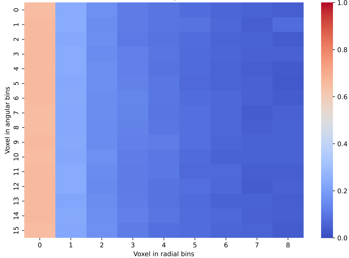
Geant4 Data: Layer 4 and 5
