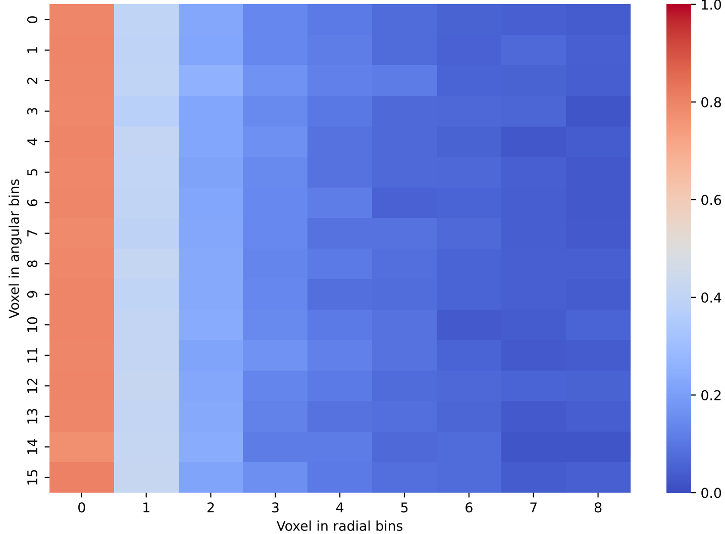
CaloINN Data: Layer 6 and 7
