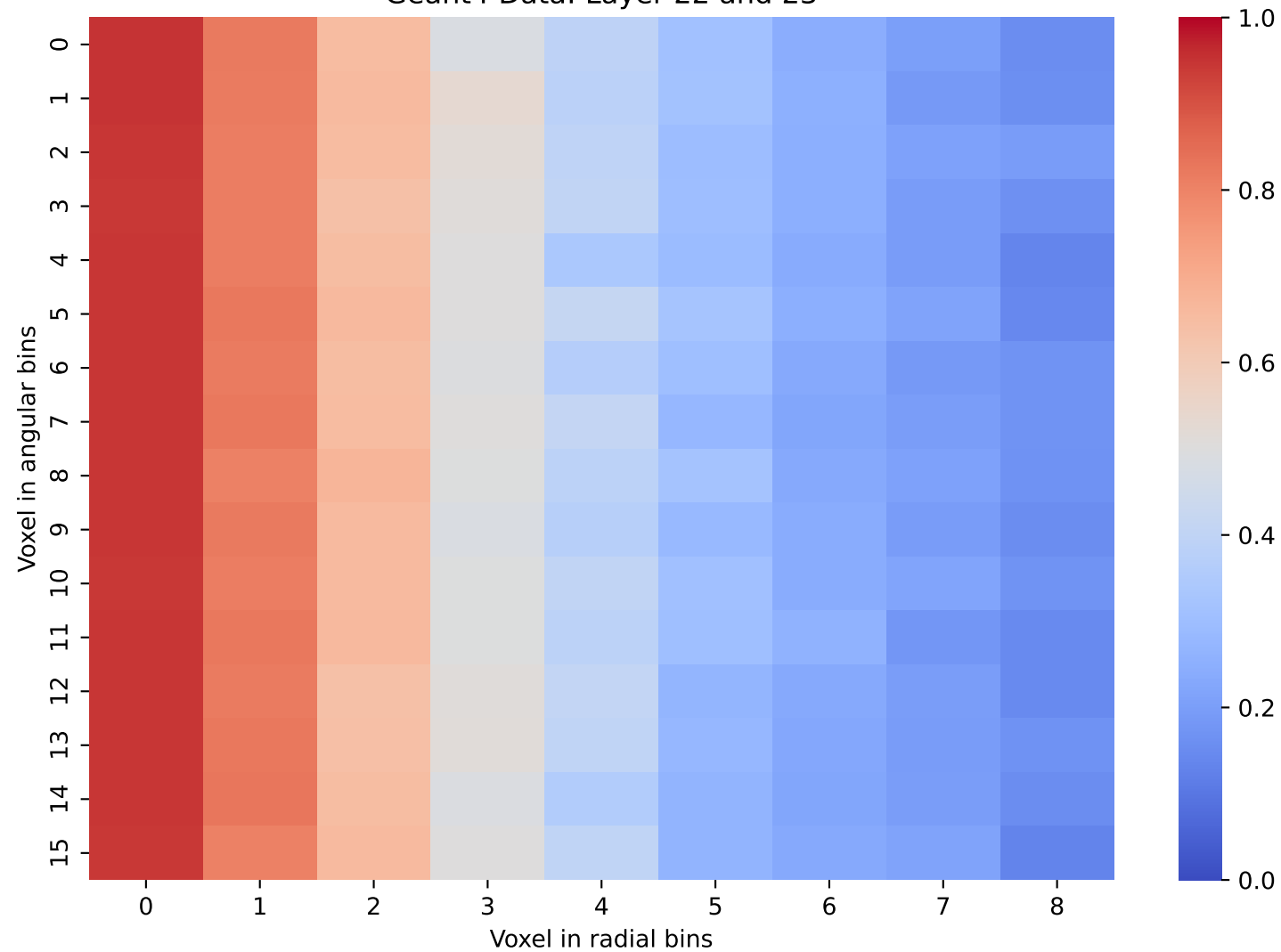
Geant4 Data: Layer 22 and 23
