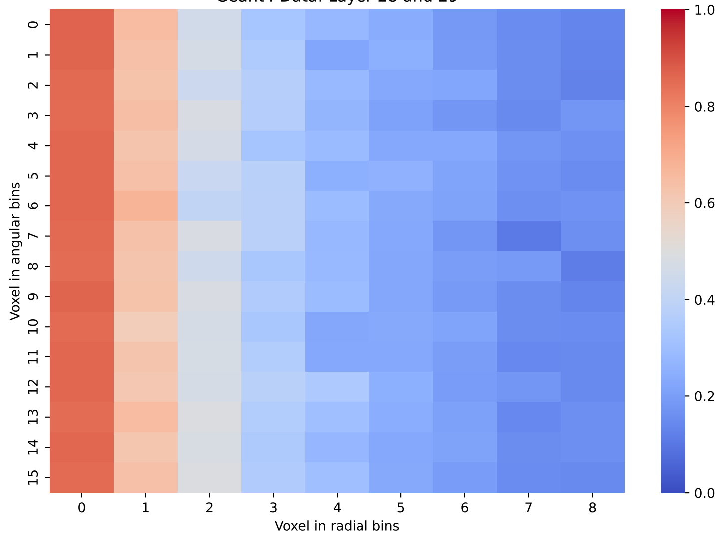
Geant4 Data: Layer 28 and 29
