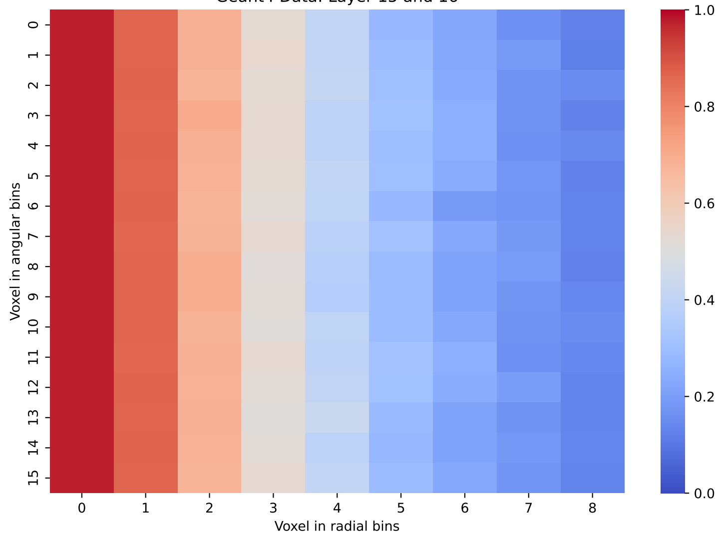
Geant4 Data: Layer 15 and 16
