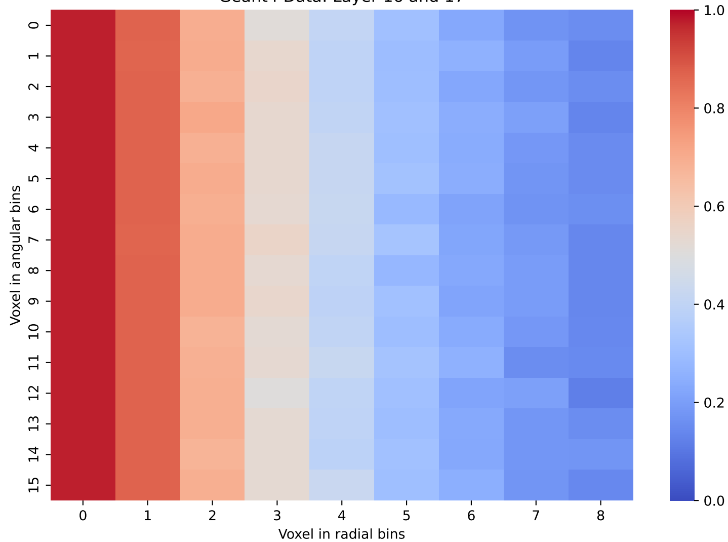
Geant4 Data: Layer 16 and 17
