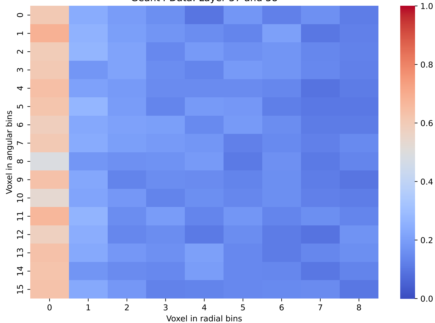
Geant4 Data: Layer 37 and 38
