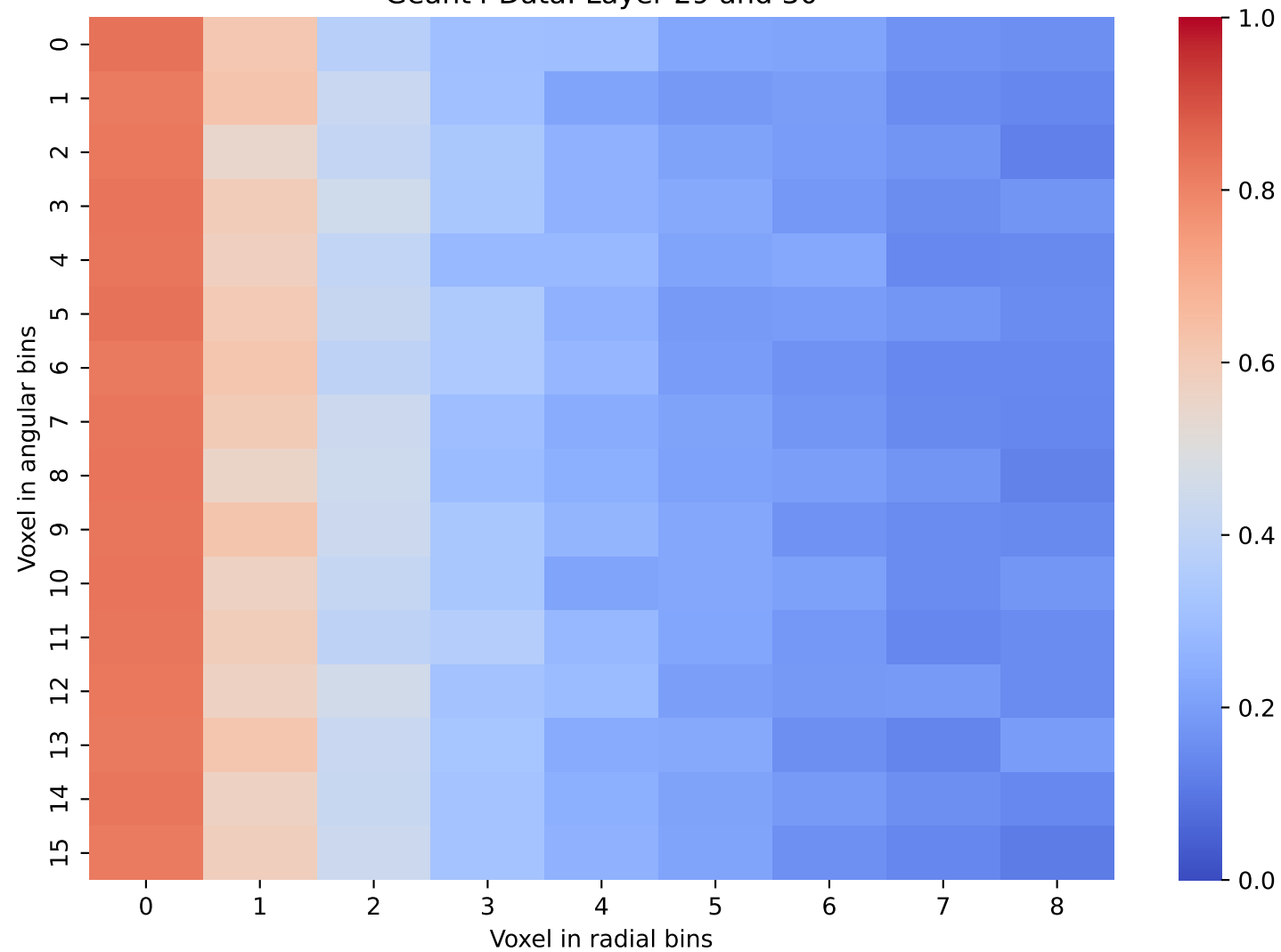
Geant4 Data: Layer 29 and 30
