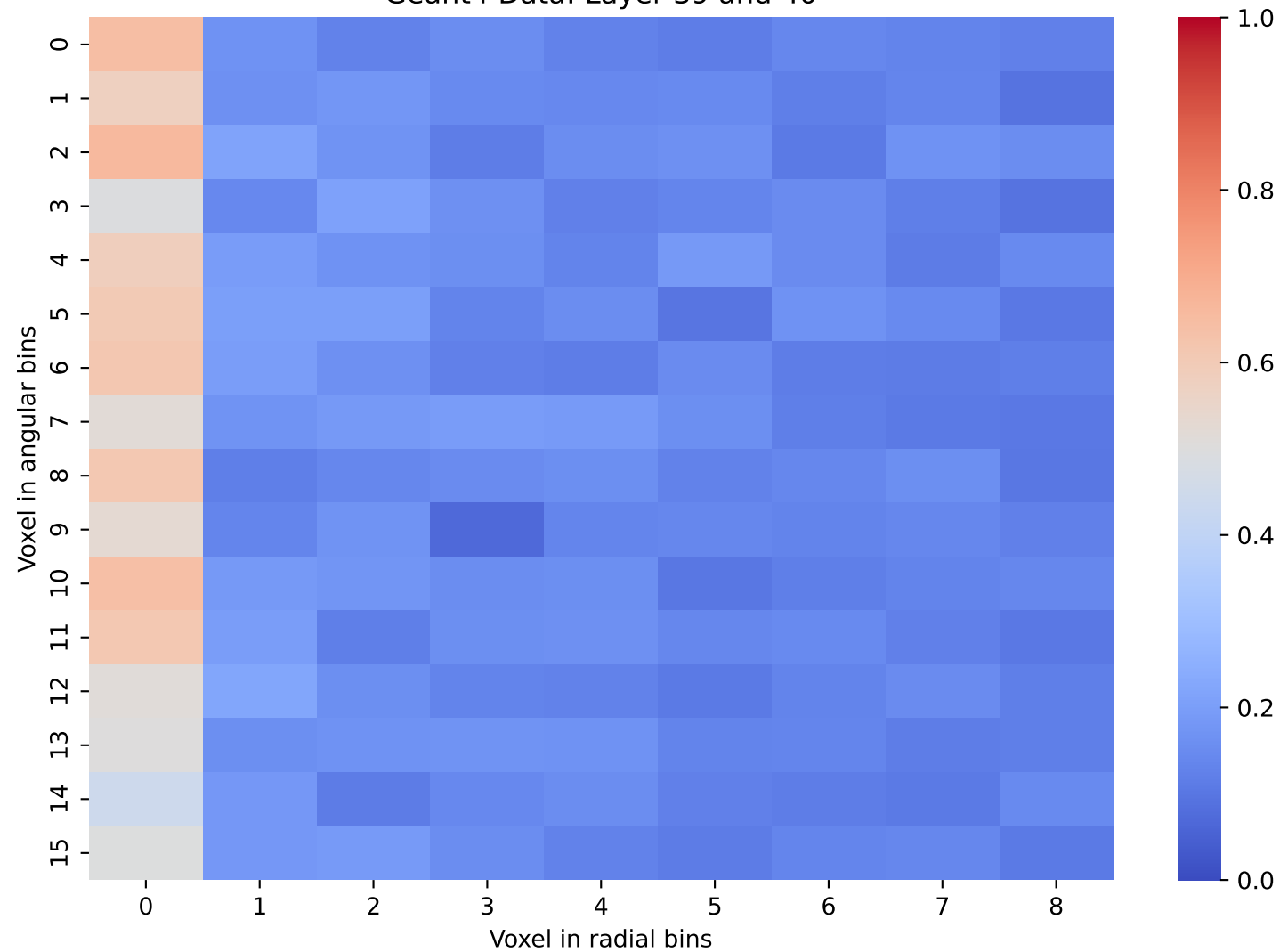
Geant4 Data: Layer 39 and 40
