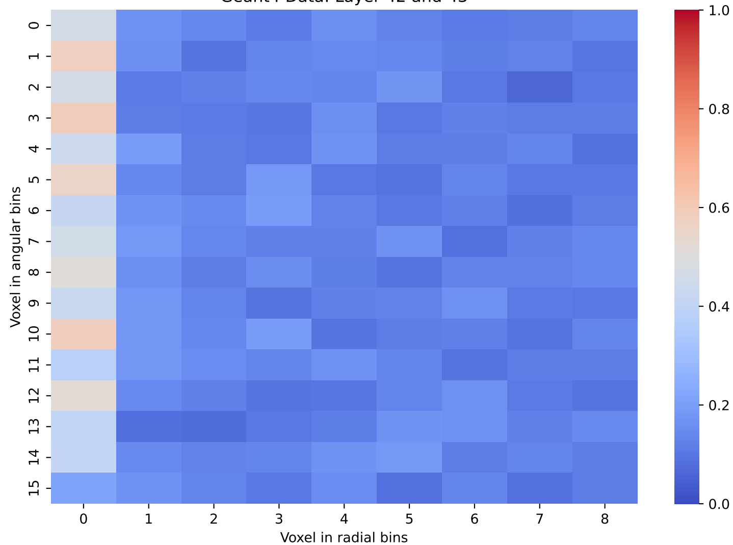
Geant4 Data: Layer 42 and 43
