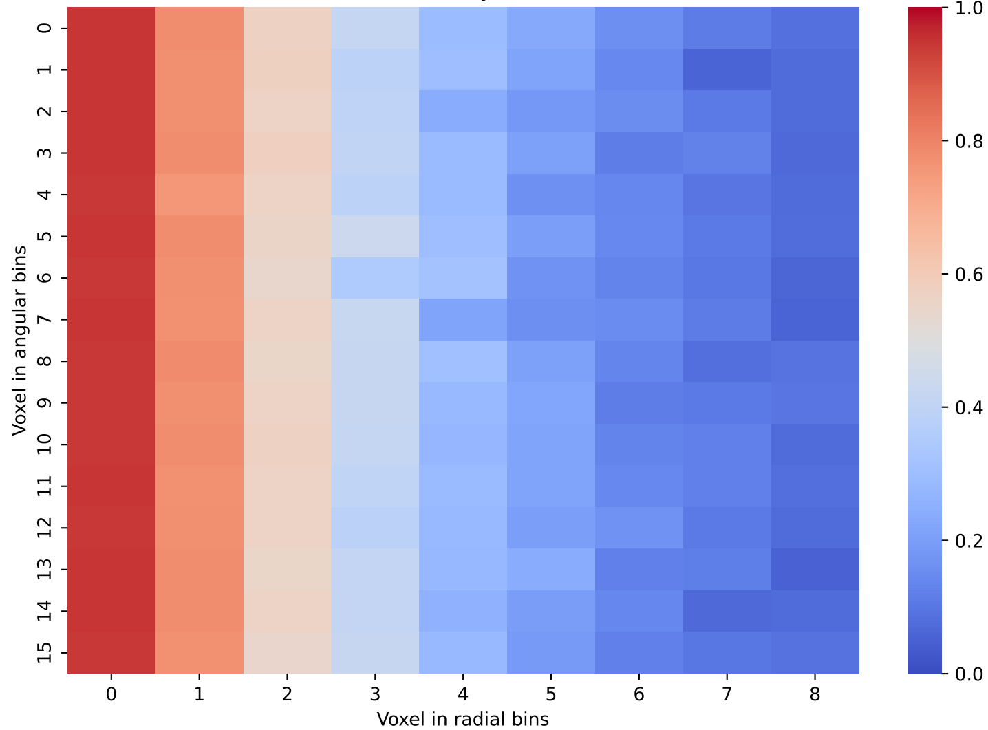
CaloINN Data: Layer 14 and 15
