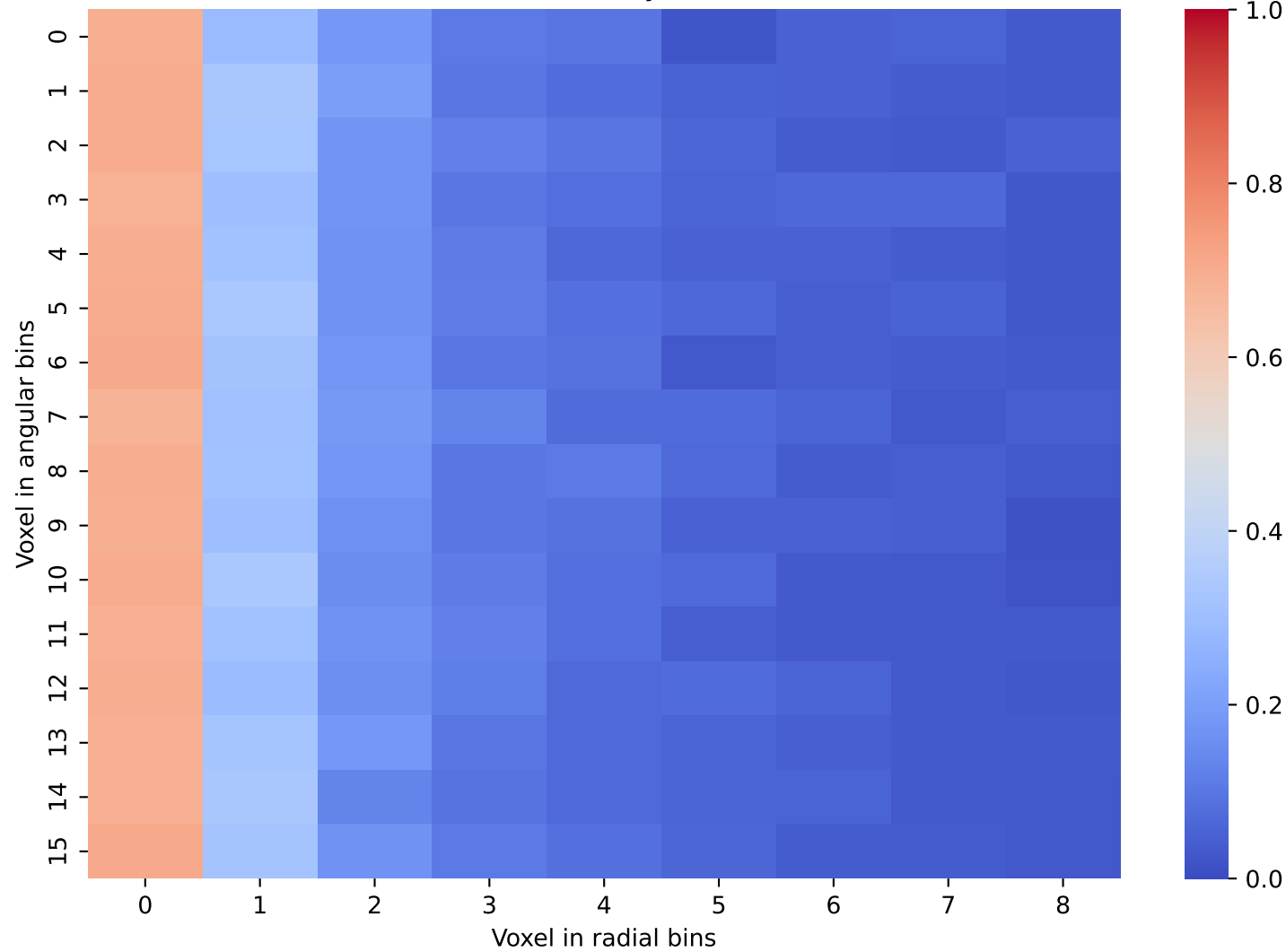
CaloINN Data: Layer 5 and 6
