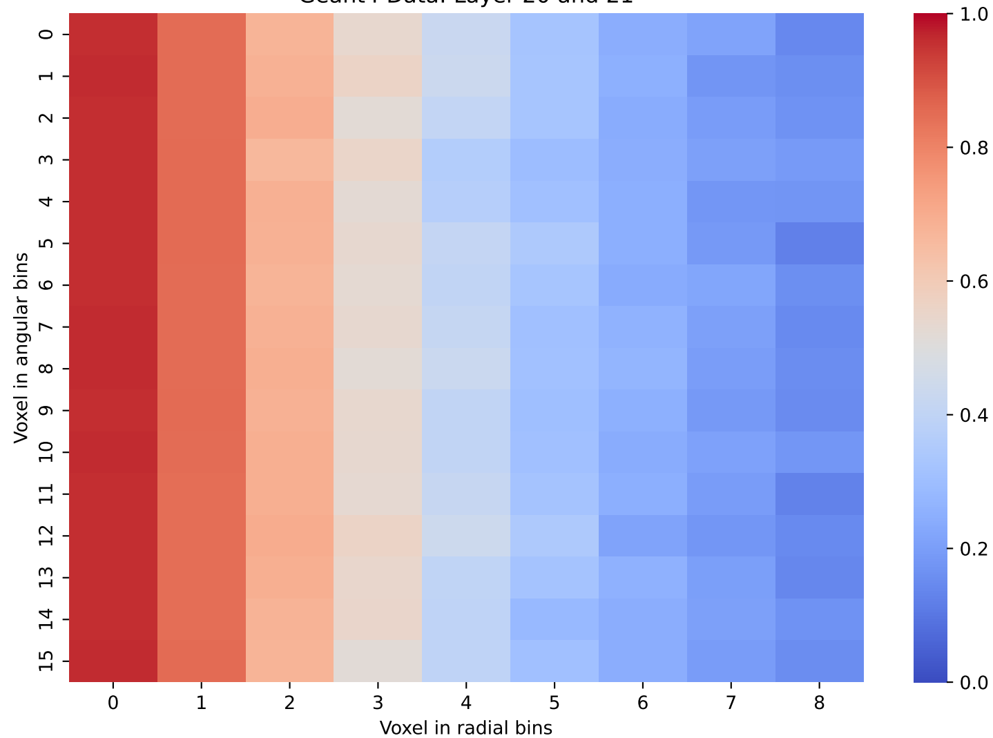
Geant4 Data: Layer 20 and 21
