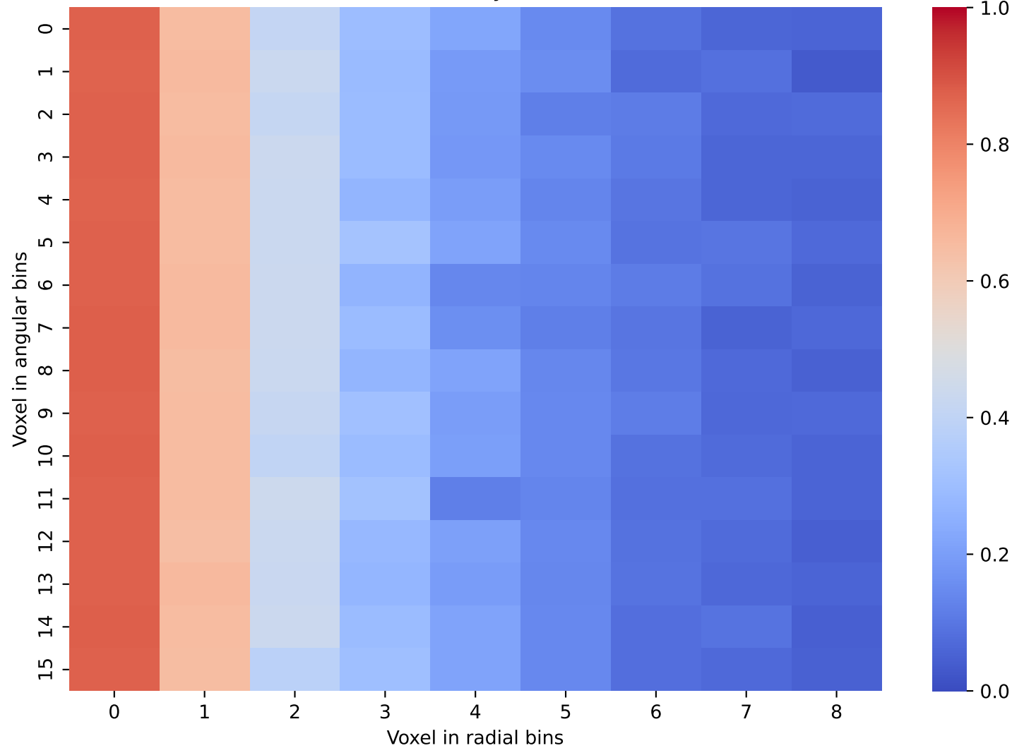
CaloINN Data: Layer 10 and 11
