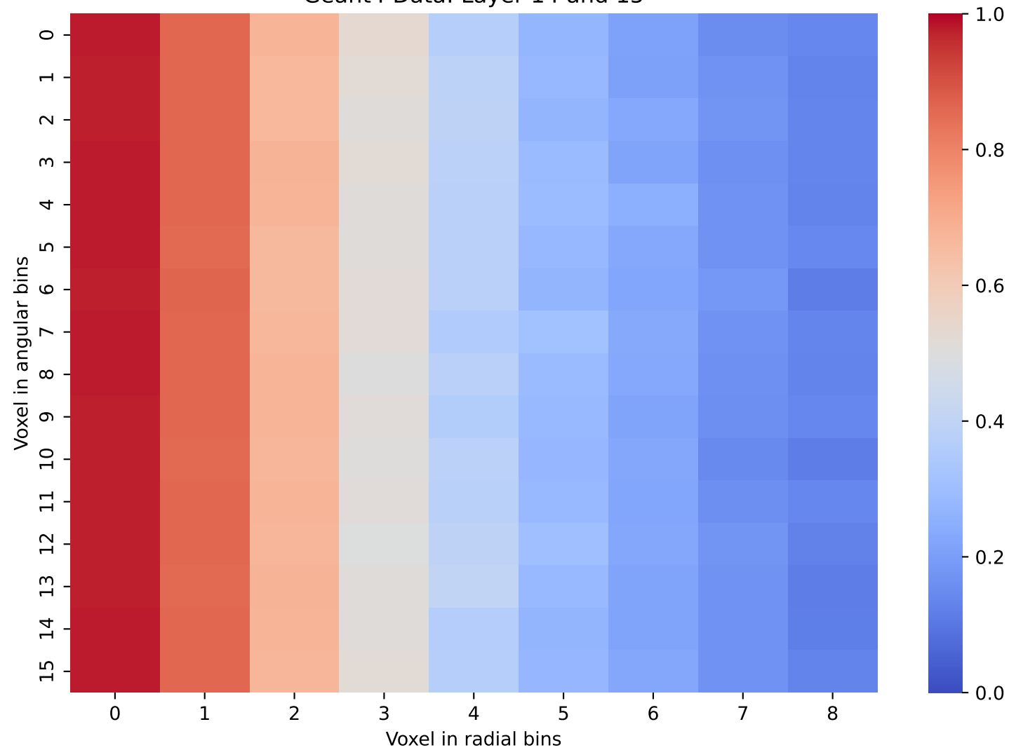
Geant4 Data: Layer 14 and 15
