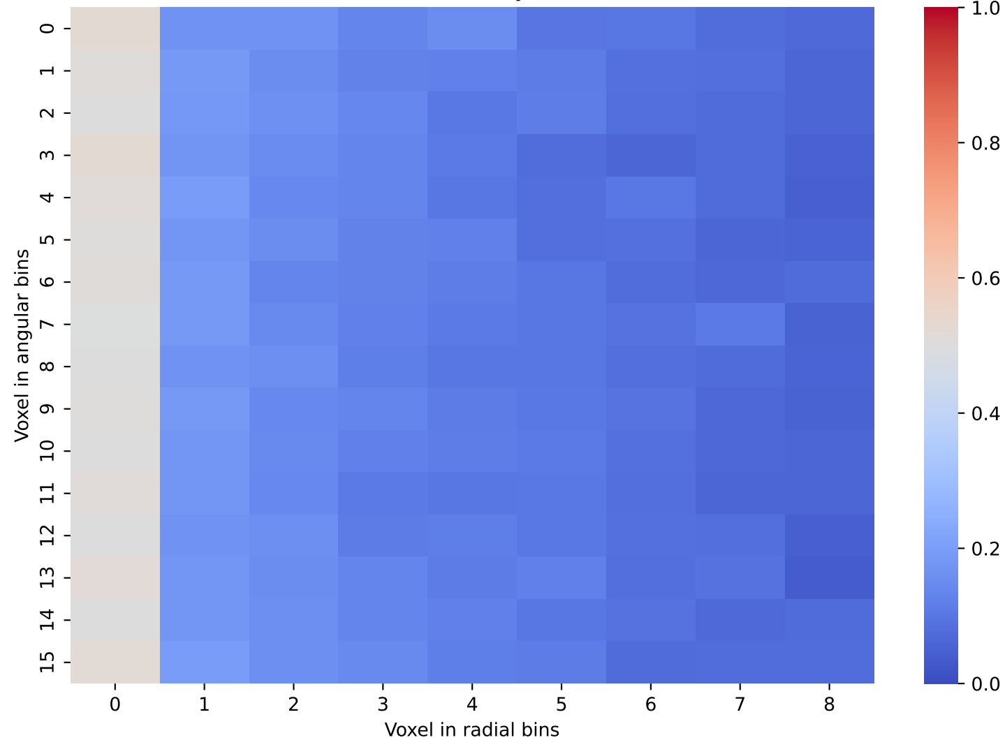
CaloScore Data: Layer 3 and 4
