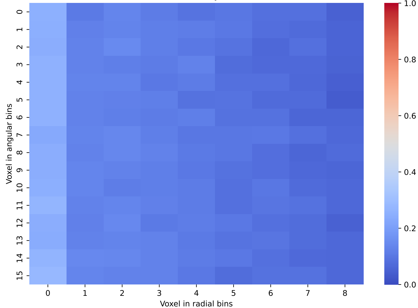
CaloScore Data: Layer 2 and 3
