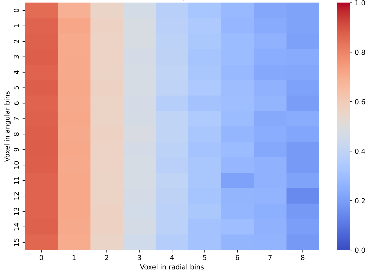
CaloScore Data: Layer 27 and 28
