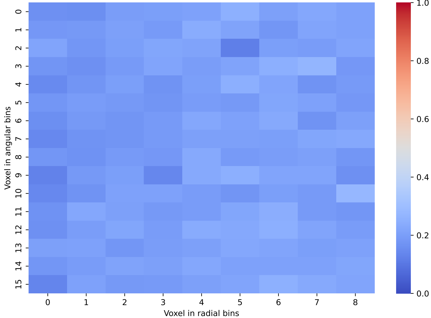
CaloScore Data: Layer 42 and 43
