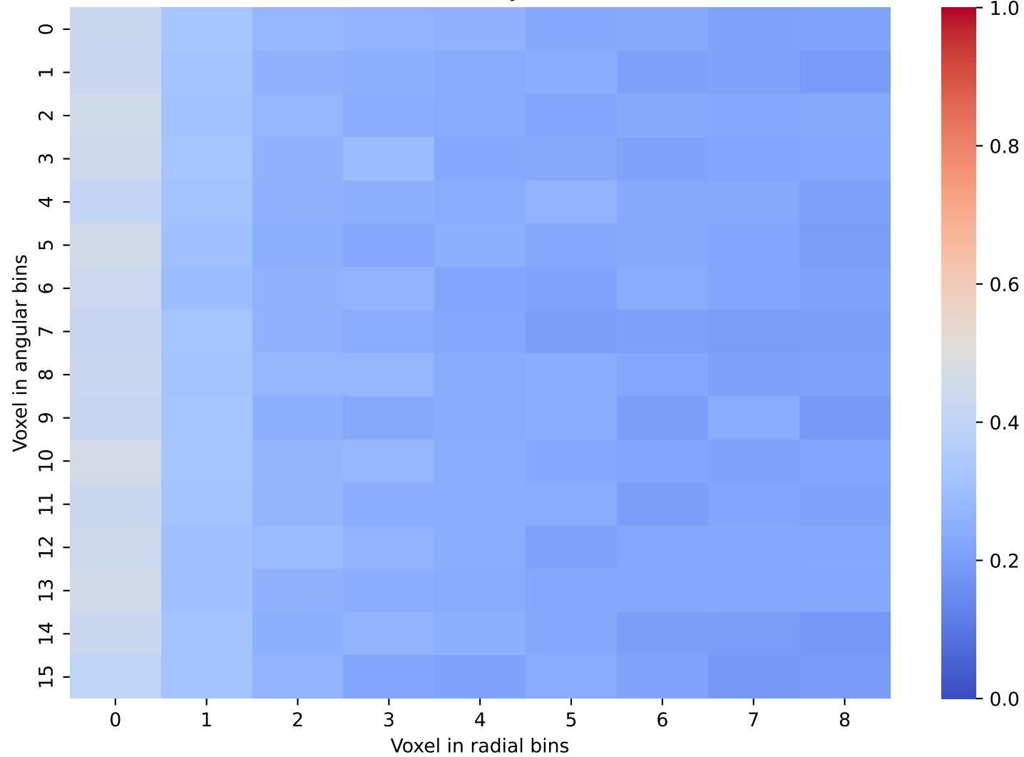
CaloScore Data: Layer 36 and 37
