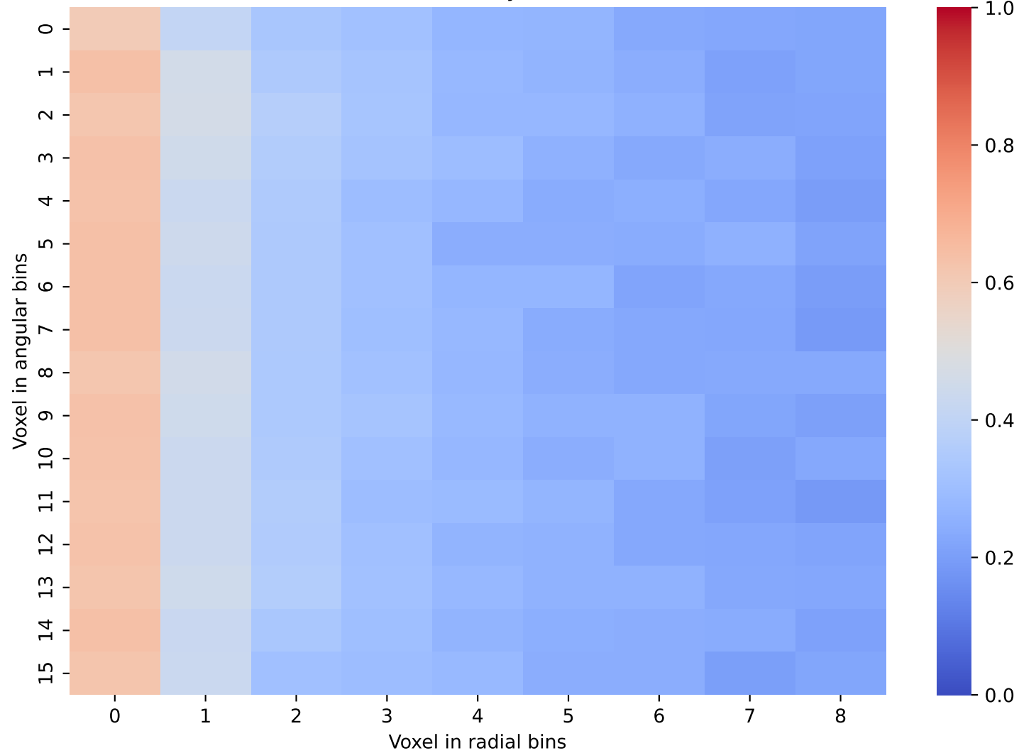
CaloScore Data: Layer 33 and 34
