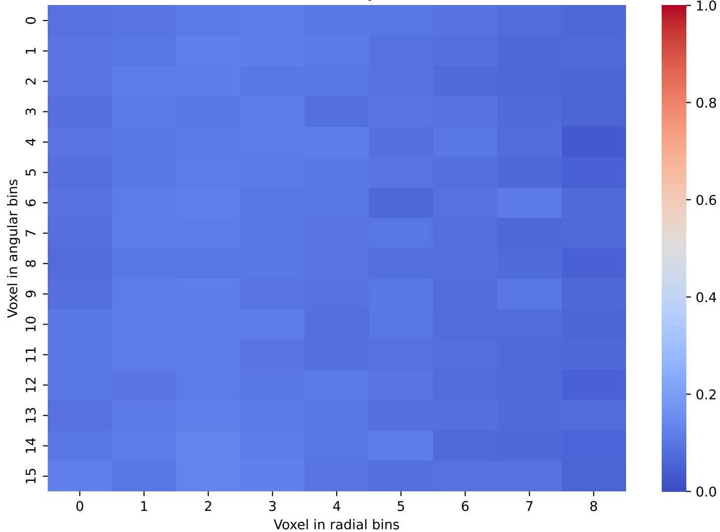
CaloScore Data: Layer 1 and 2
