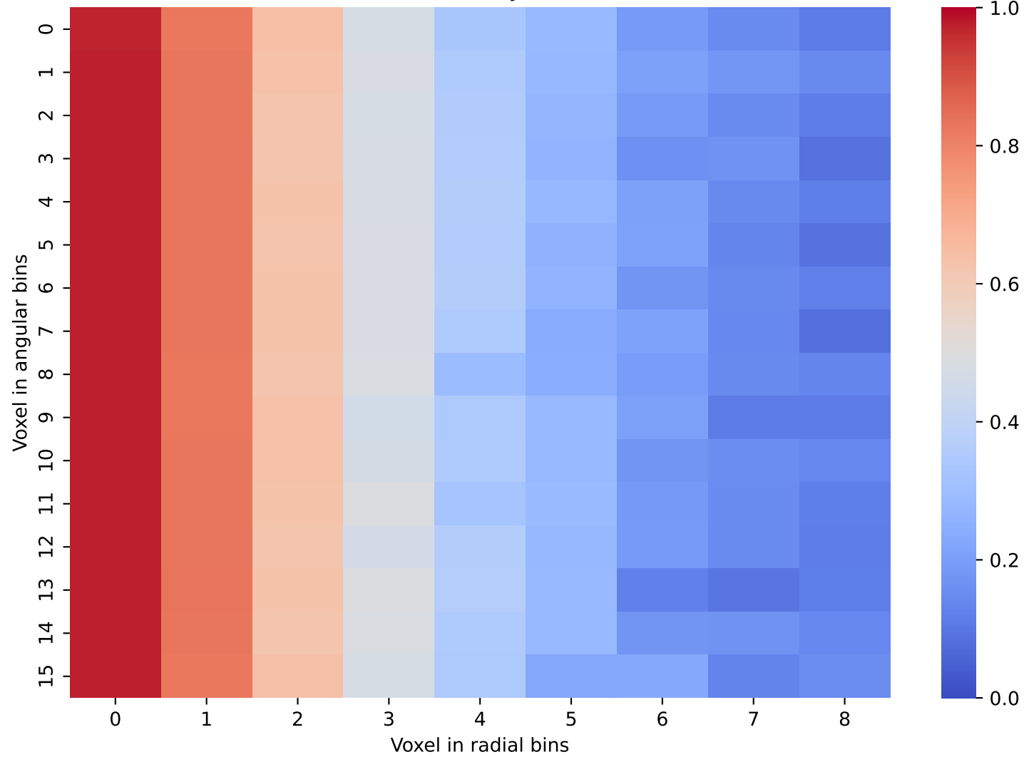
CaloScore Data: Layer 11 and 12
