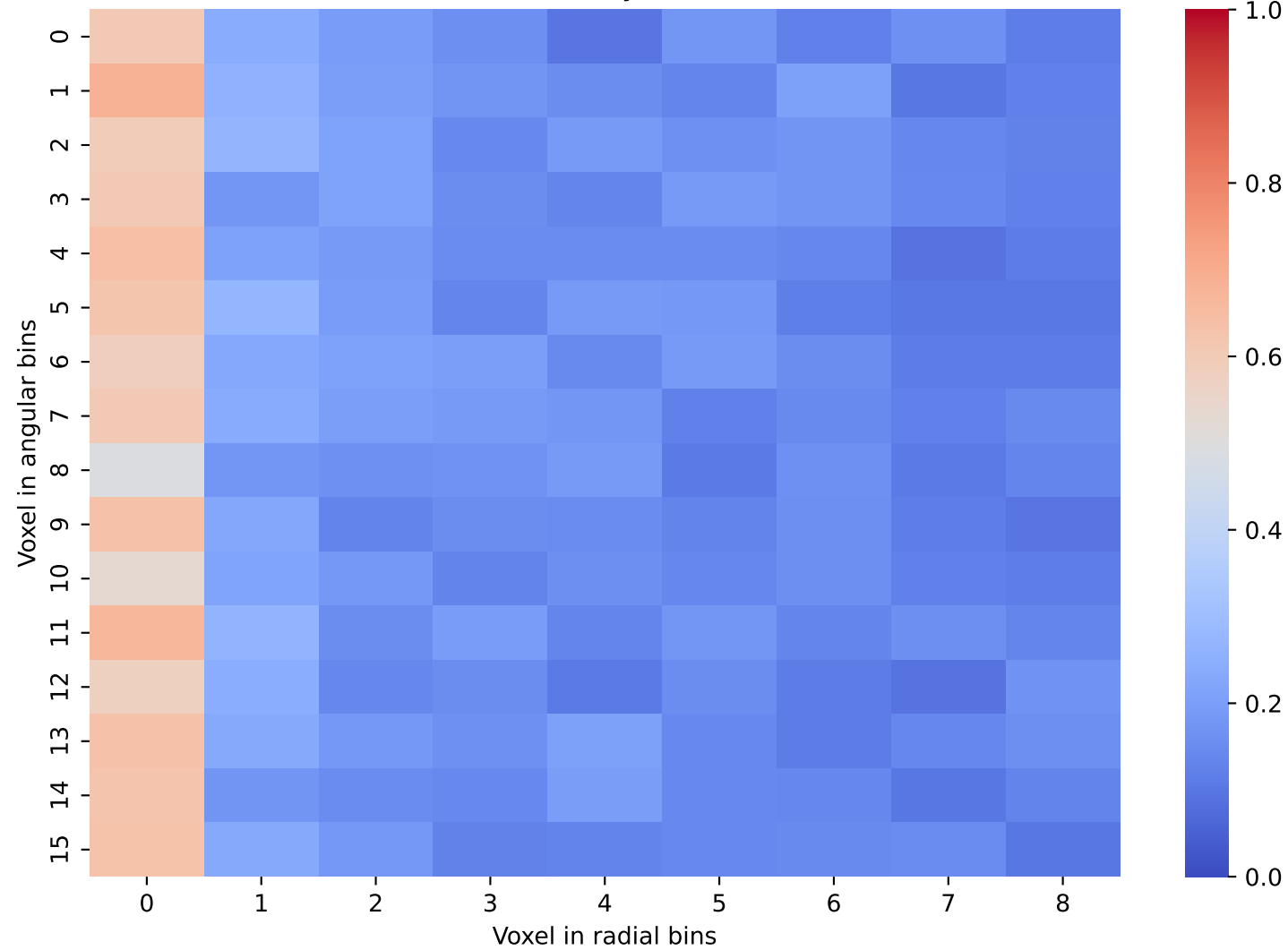
Geant4 Data: Layer 37 and 38
