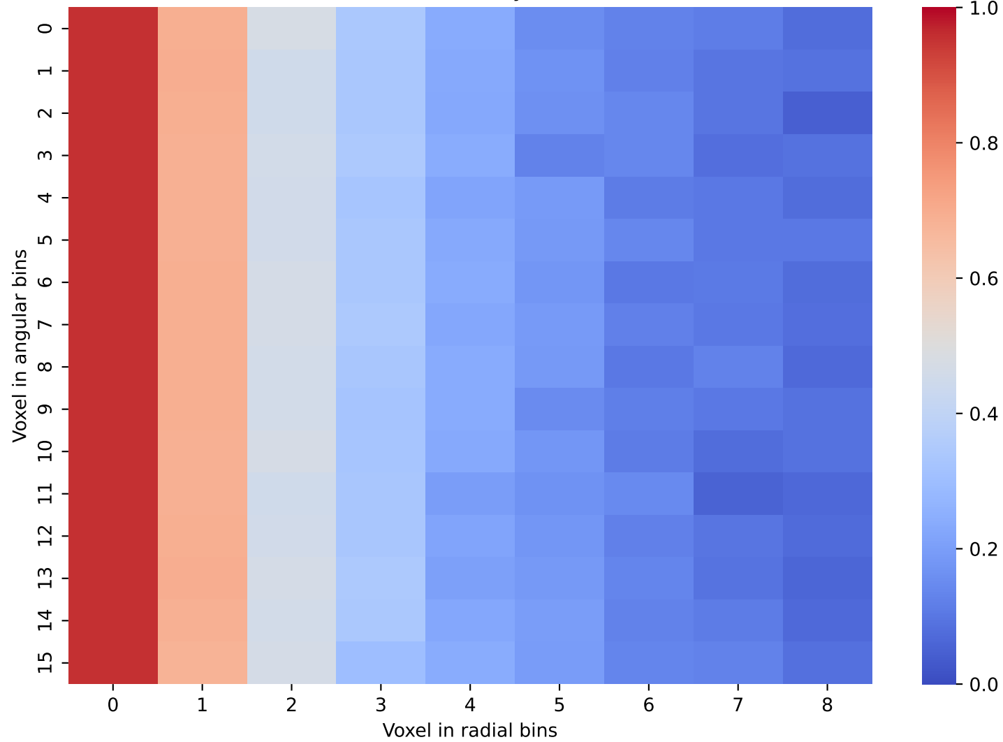
CaloScore Data: Layer 8 and 9
