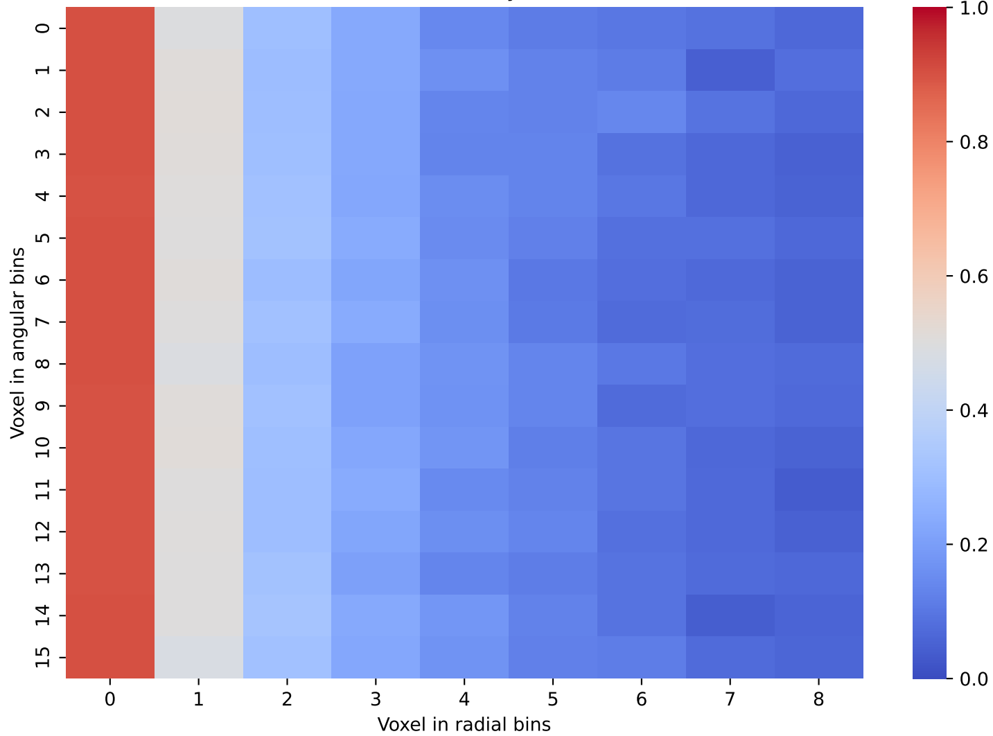
CaloScore Data: Layer 6 and 7
