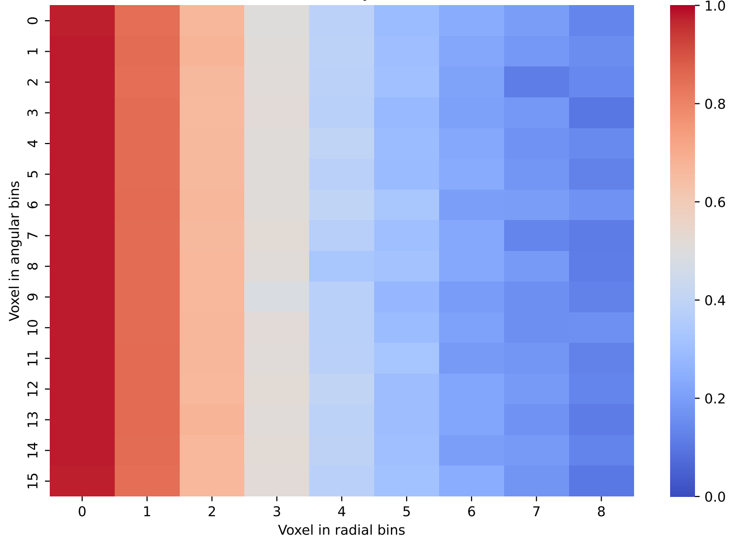
CaloScore Data: Layer 12 and 13
