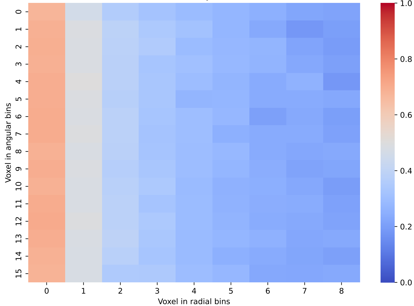
CaloScore Data: Layer 32 and 33
