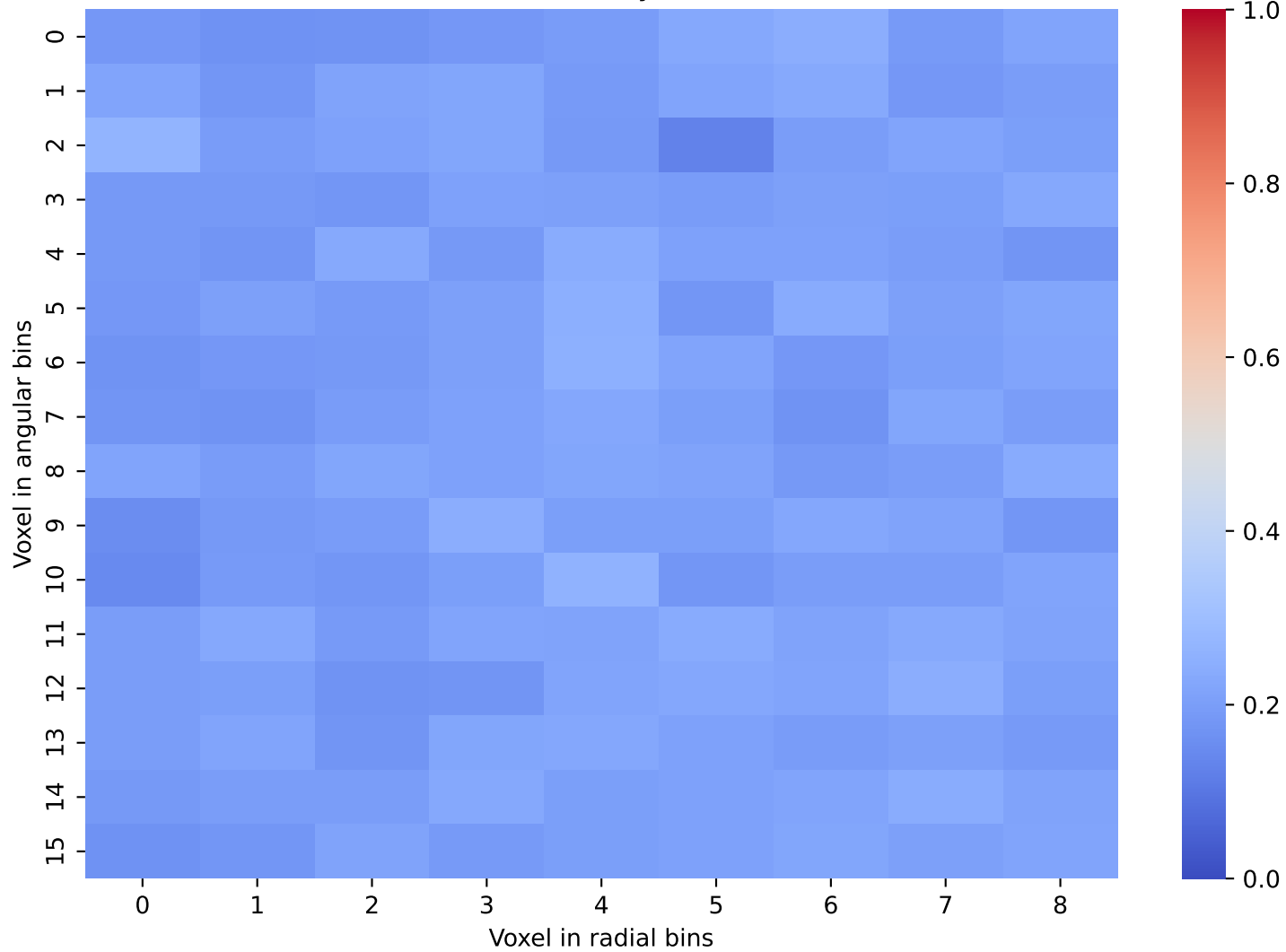
CaloScore Data: Layer 41 and 42
