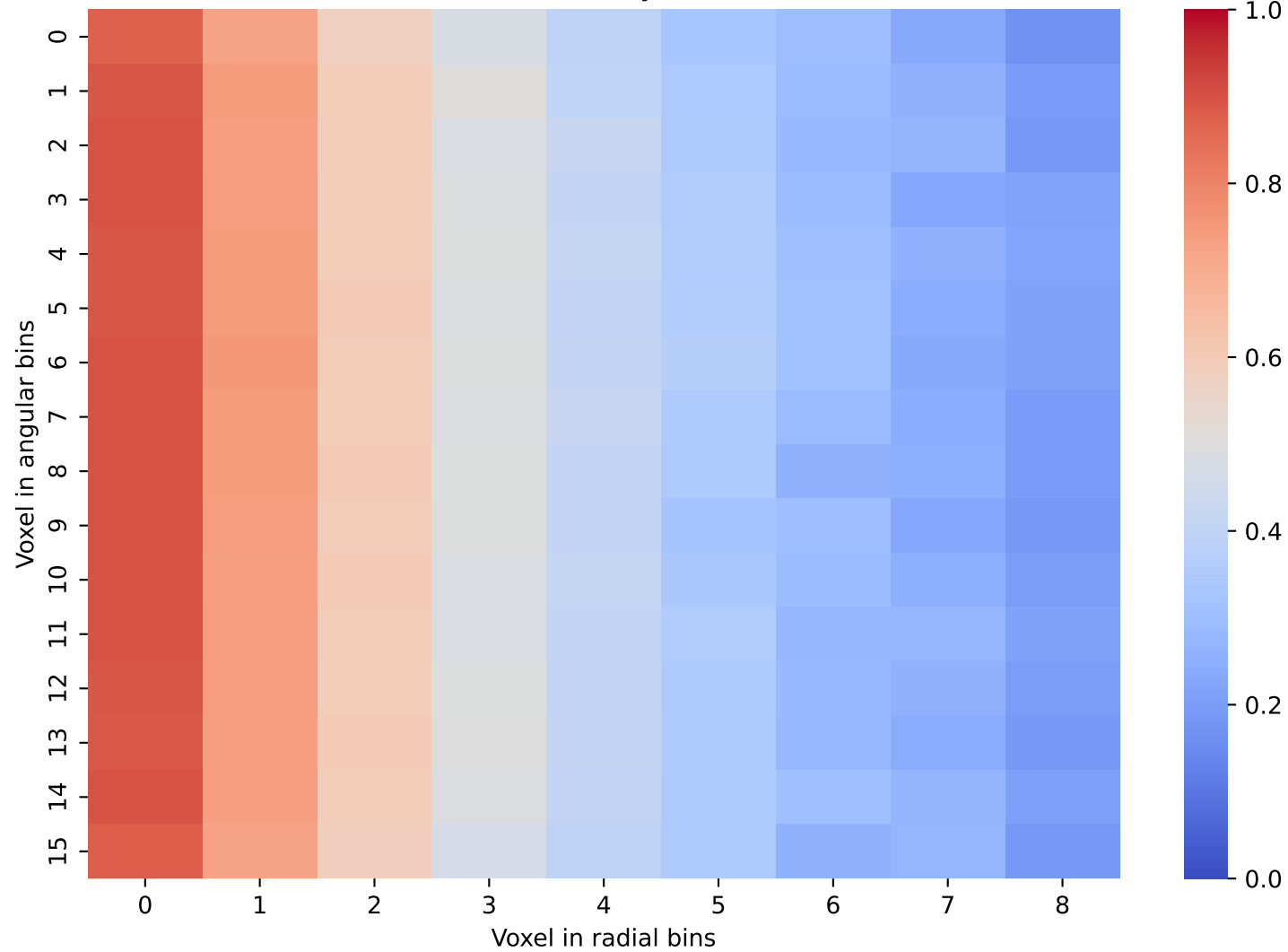
CaloScore Data: Layer 26 and 27
