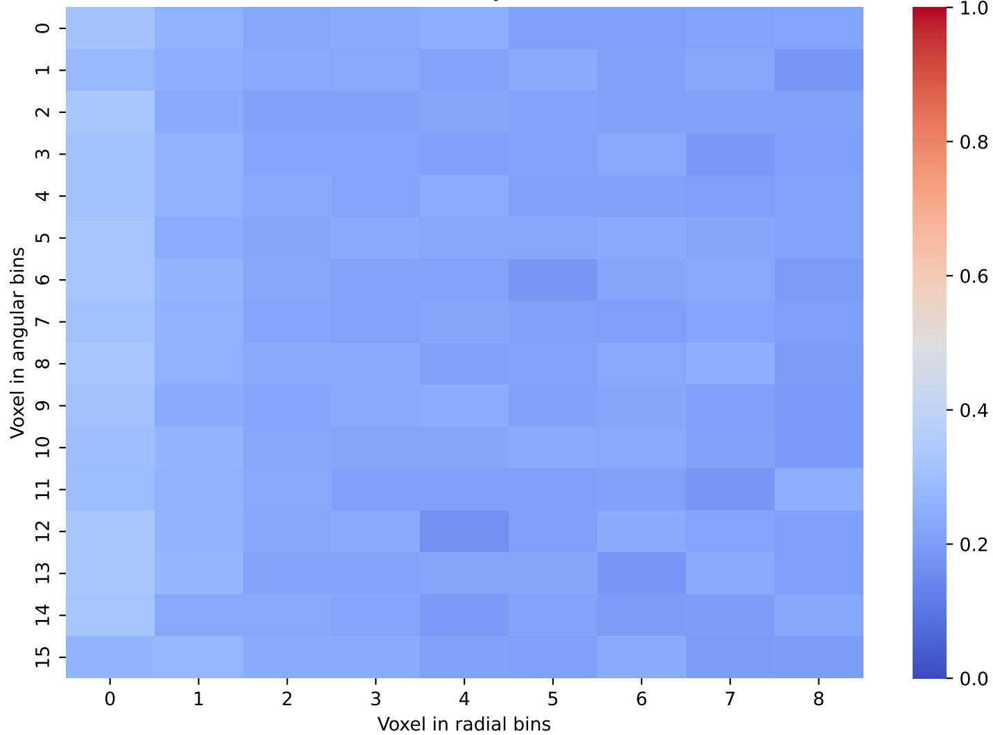
CaloScore Data: Layer 38 and 39
