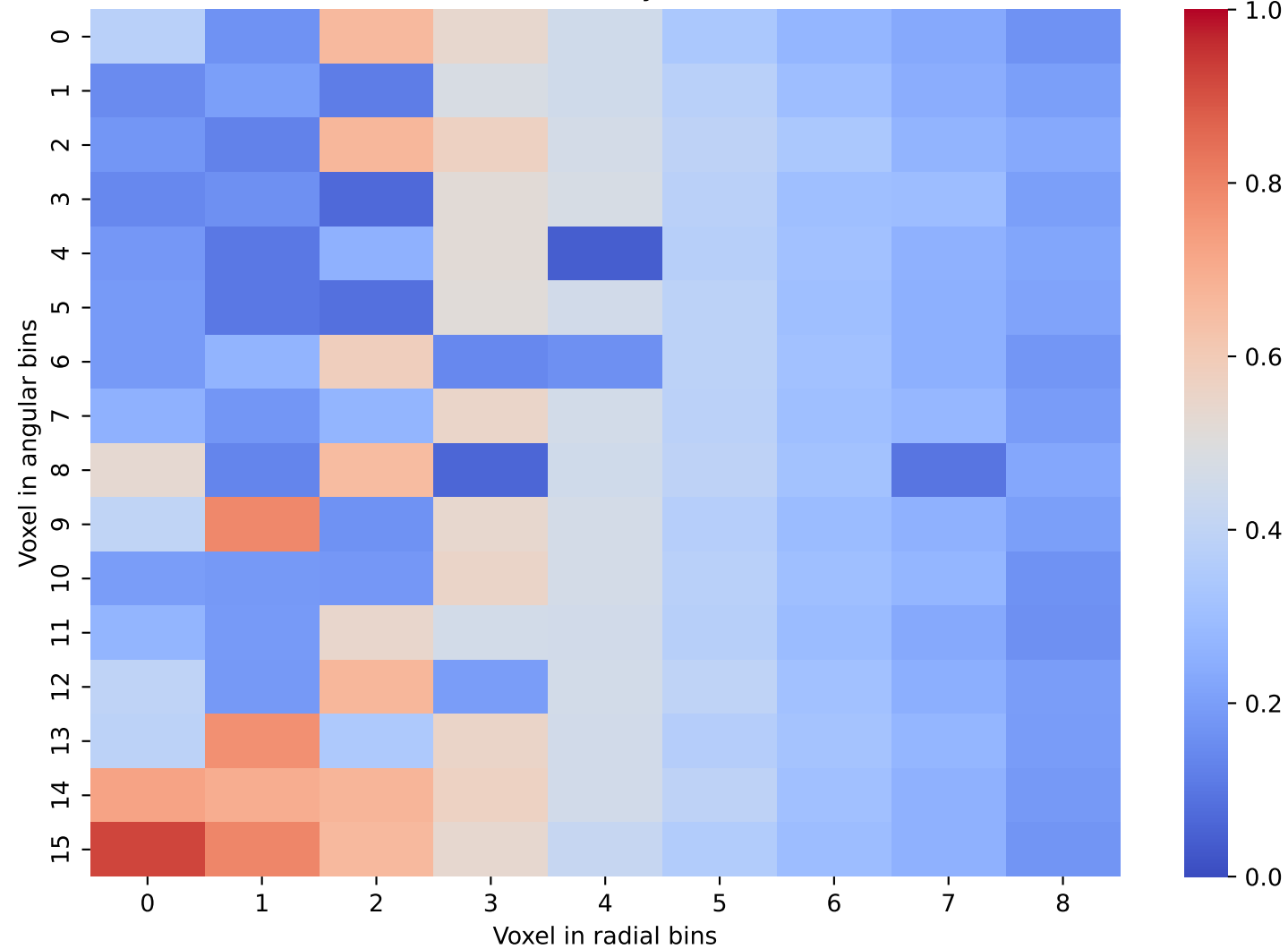
CaloScore Data: Layer 23 and 24
