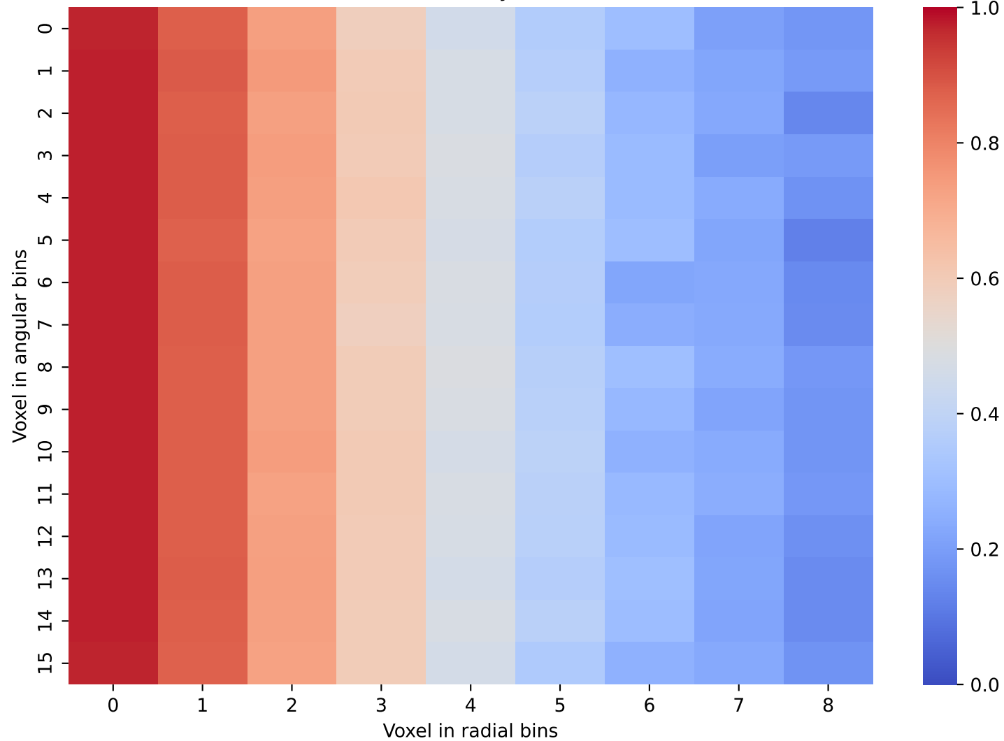
CaloScore Data: Layer 16 and 17
