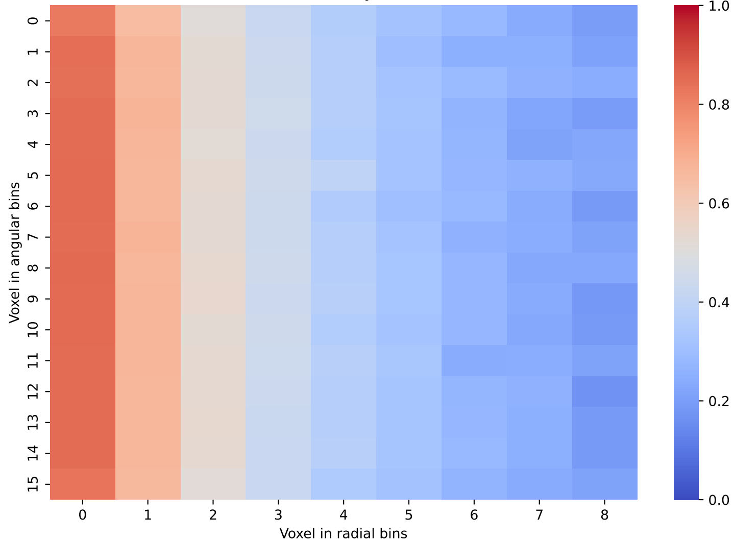
CaloScore Data: Layer 28 and 29
