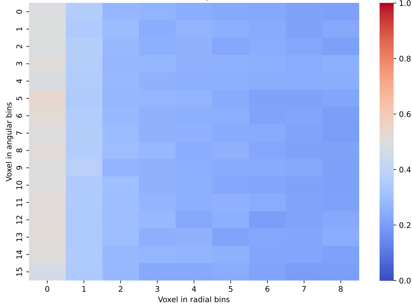
CaloScore Data: Layer 35 and 36
