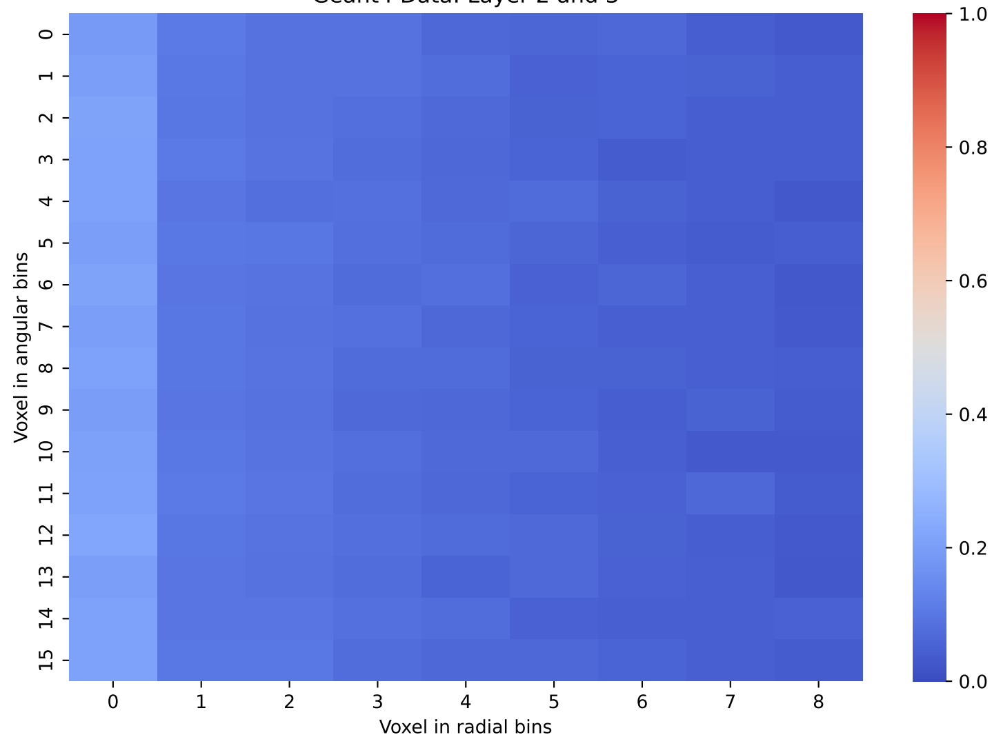
Geant4 Data: Layer 2 and 3
