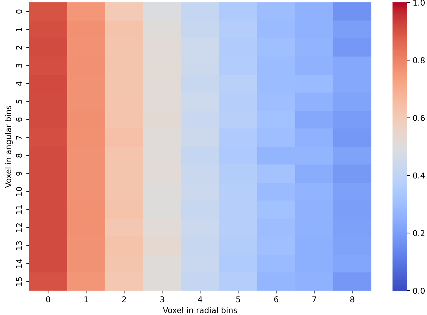
CaloScore Data: Layer 25 and 26
