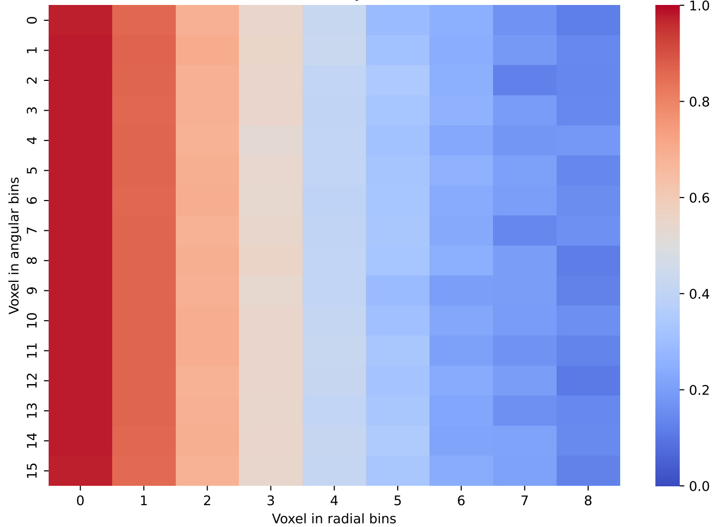
CaloScore Data: Layer 13 and 14
