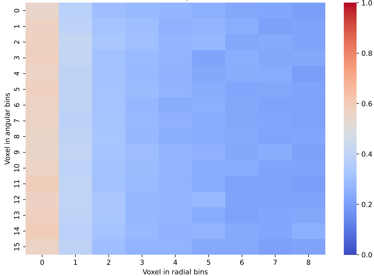
CaloScore Data: Layer 34 and 35
