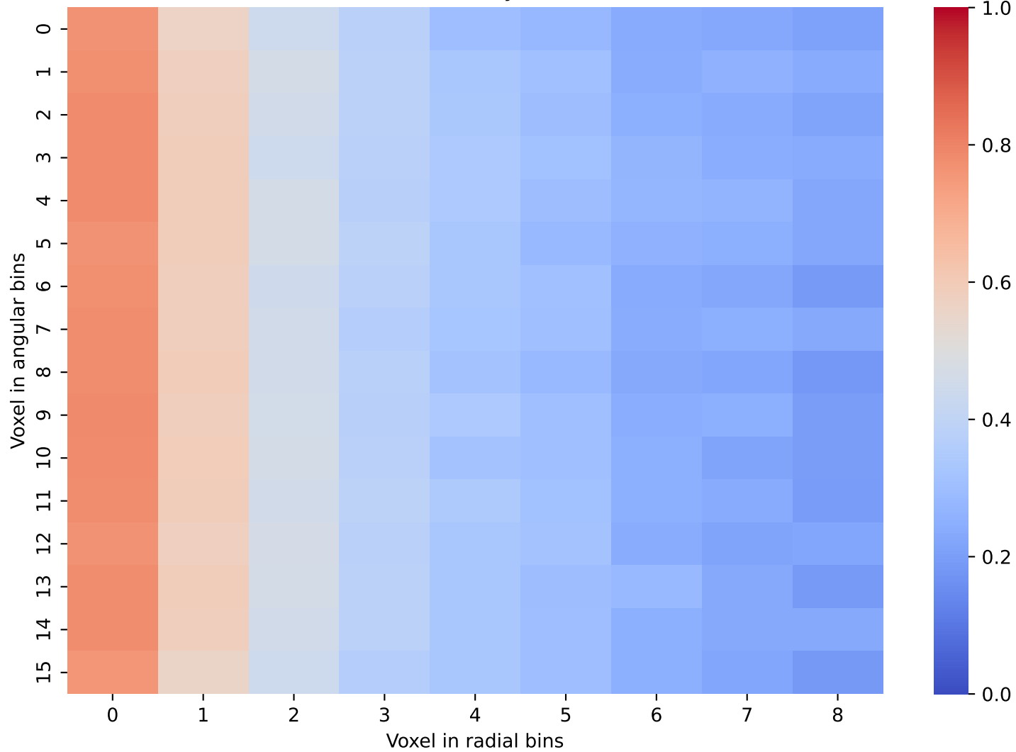
CaloScore Data: Layer 30 and 31
