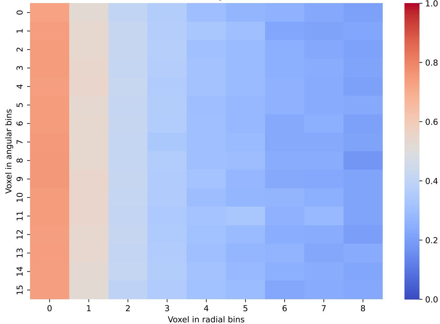
CaloScore Data: Layer 31 and 32
