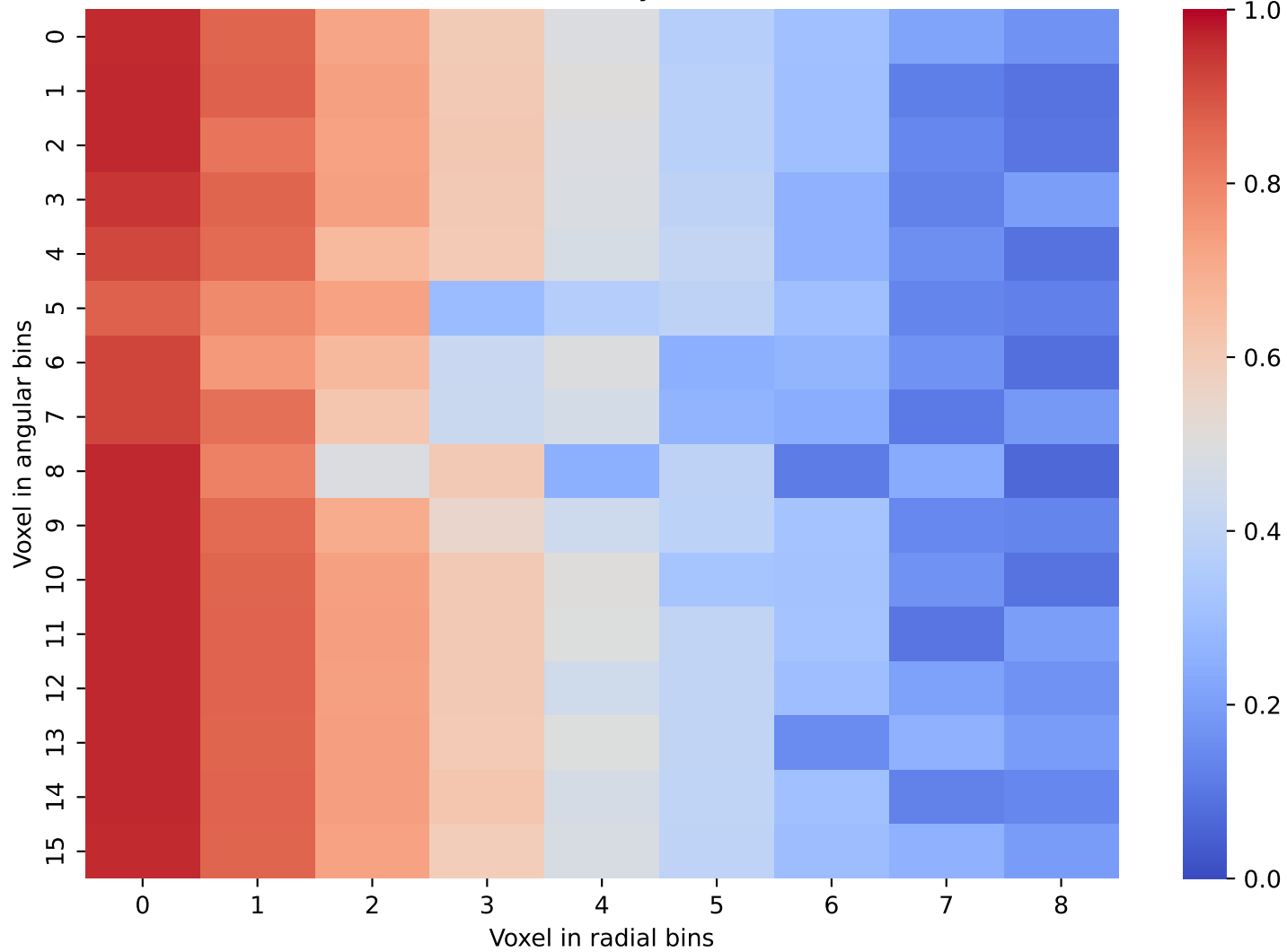
CaloScore Data: Layer 19 and 20
