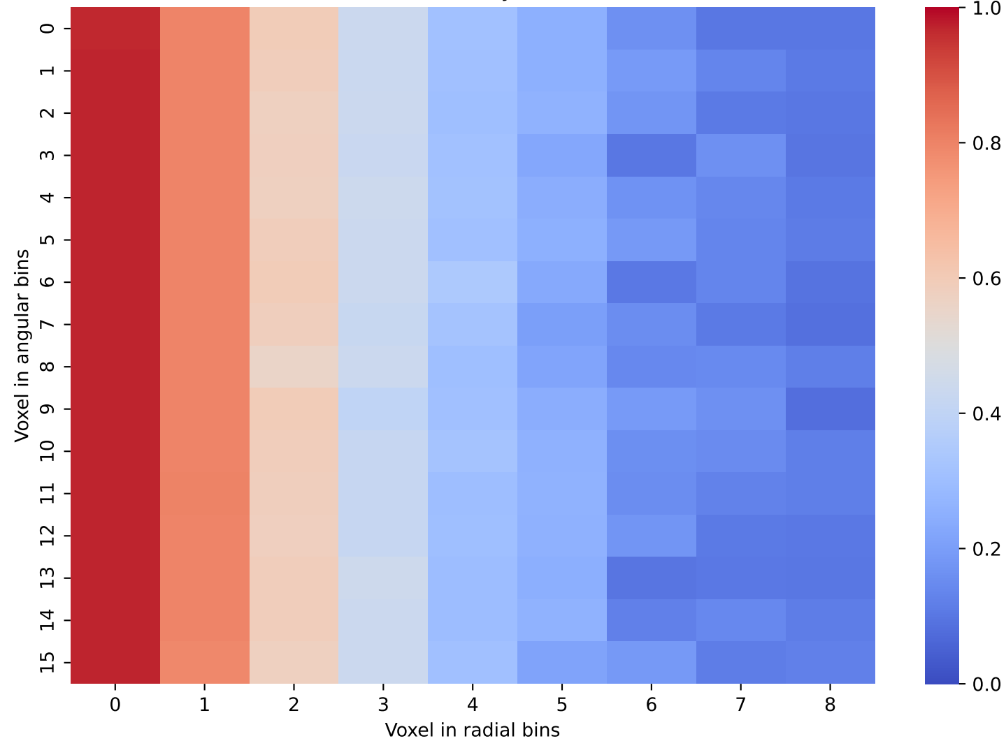
CaloScore Data: Layer 10 and 11
