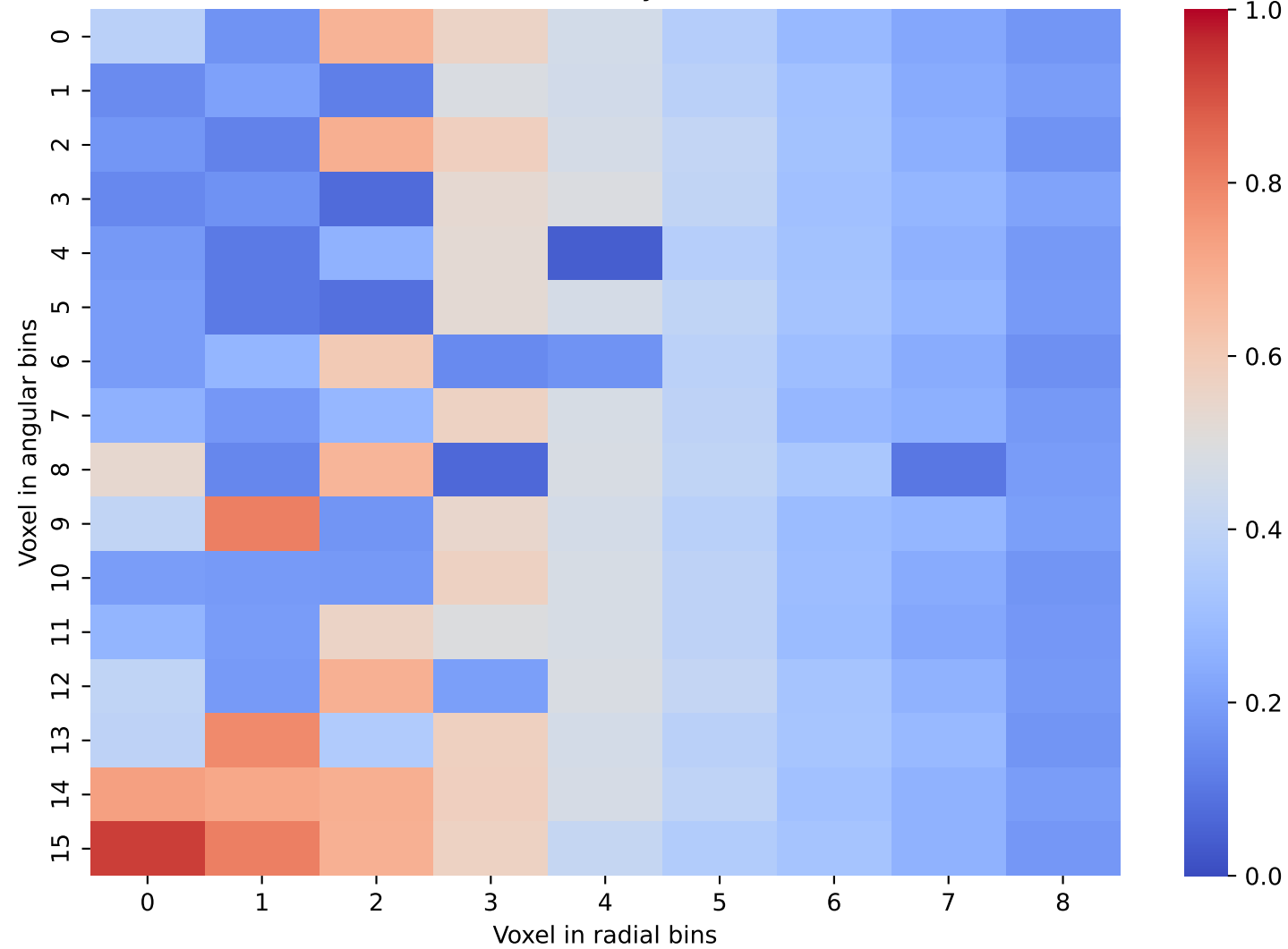
CaloScore Data: Layer 22 and 23
