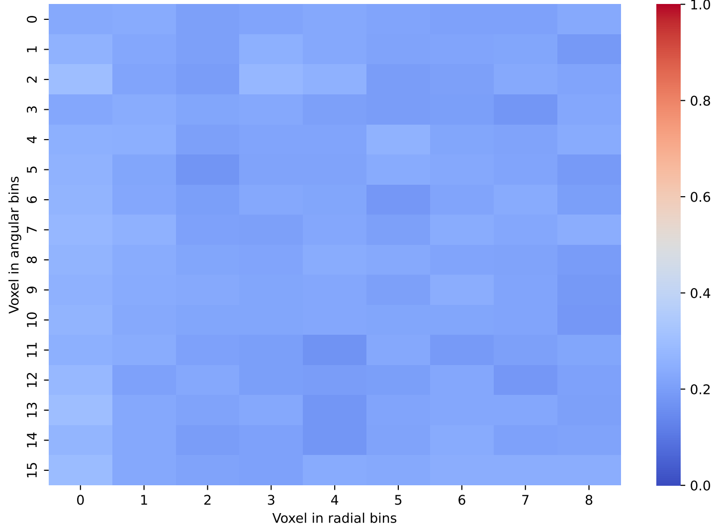
CaloScore Data: Layer 39 and 40
