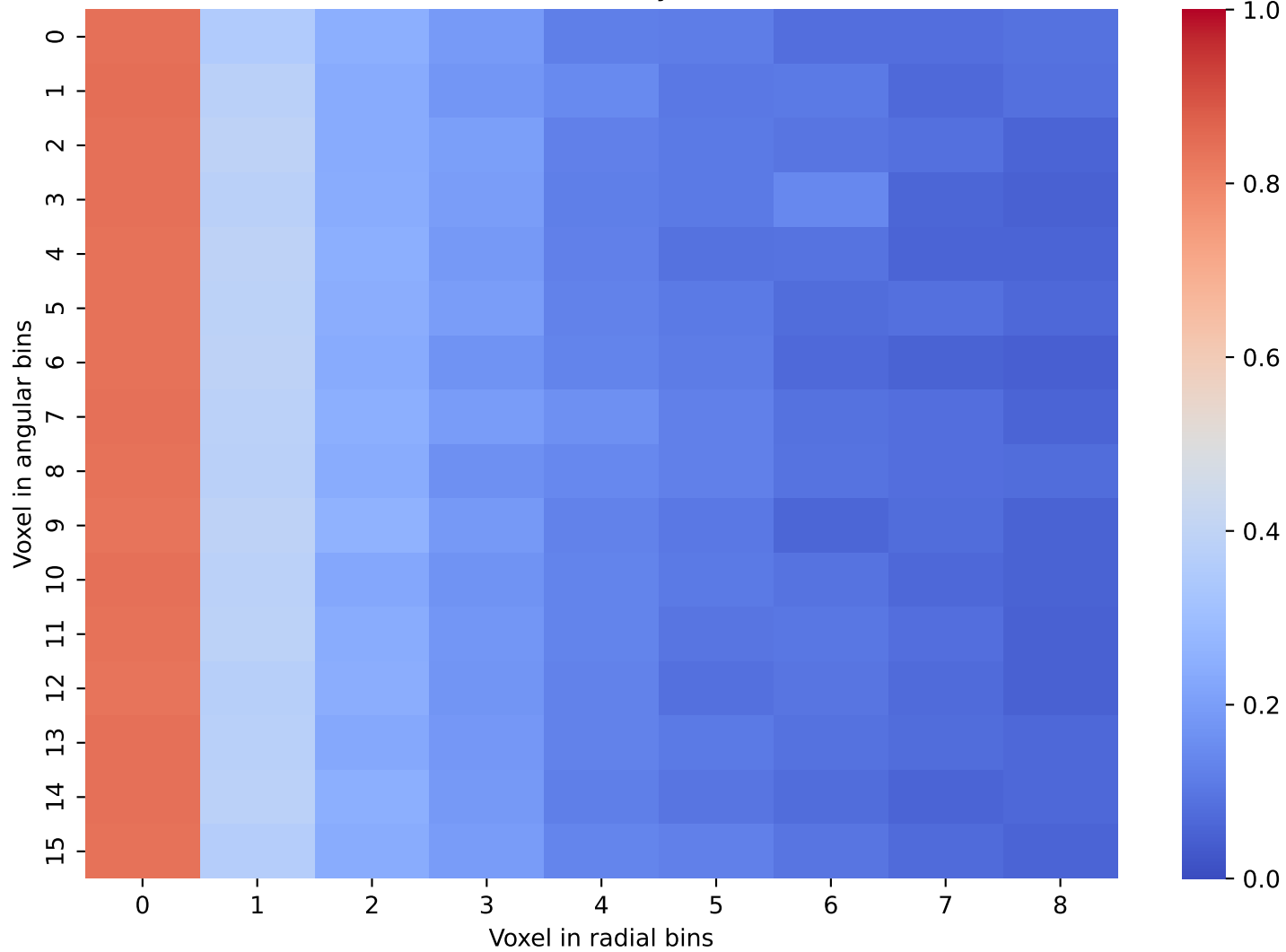
CaloScore Data: Layer 5 and 6
