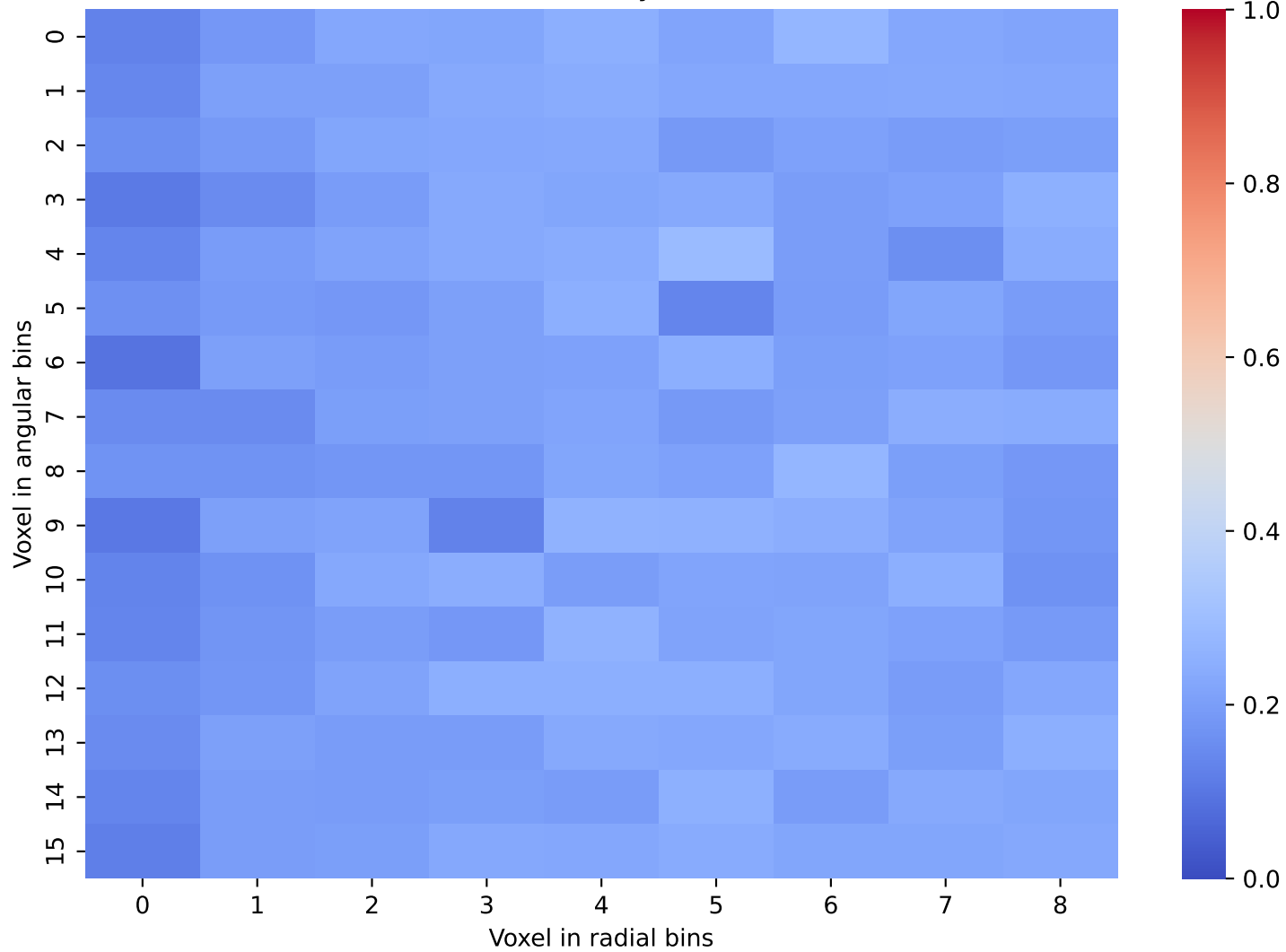
CaloScore Data: Layer 43 and 44
