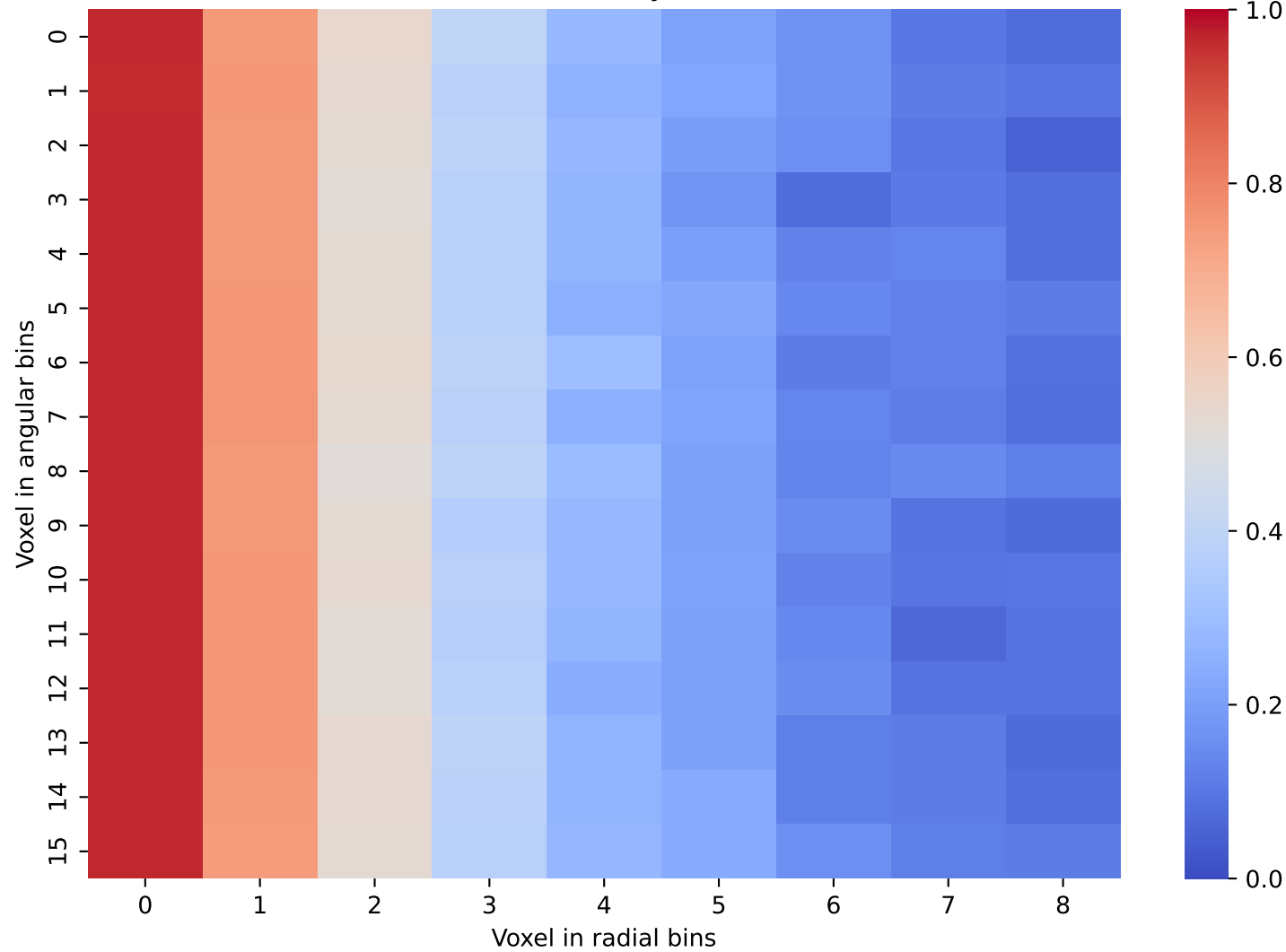
CaloScore Data: Layer 9 and 10
