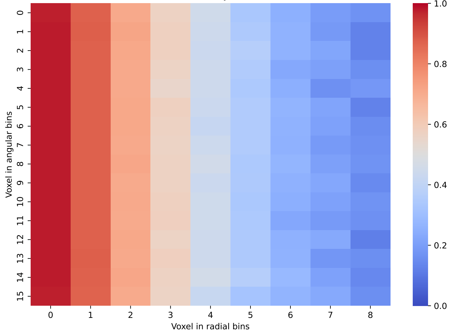
CaloScore Data: Layer 14 and 15
