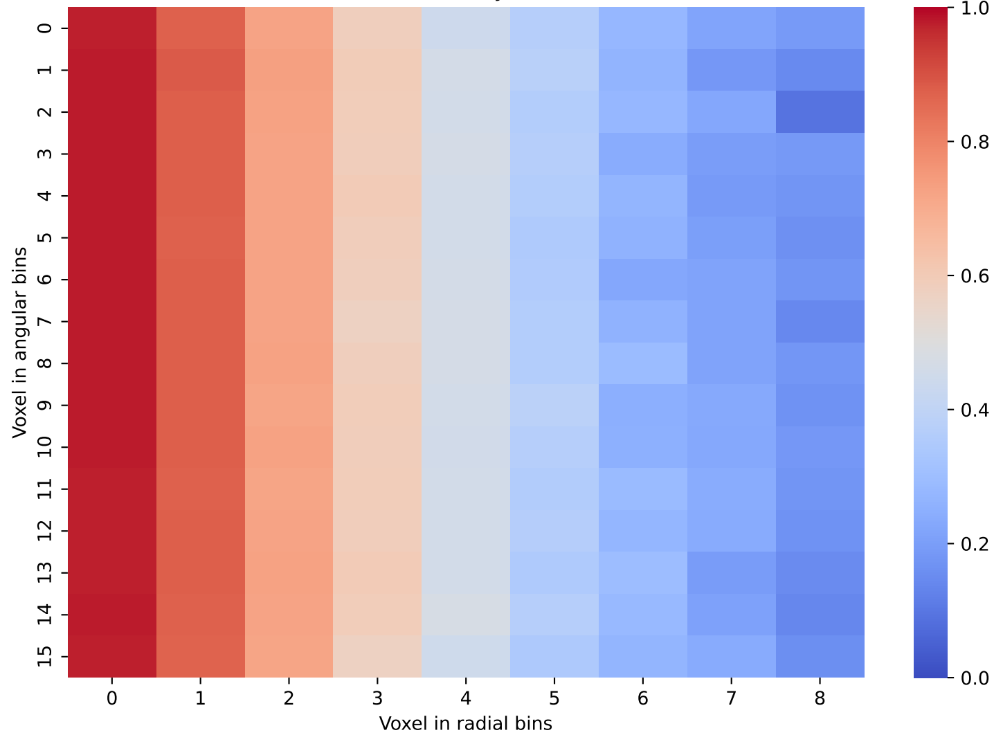
CaloScore Data: Layer 15 and 16
