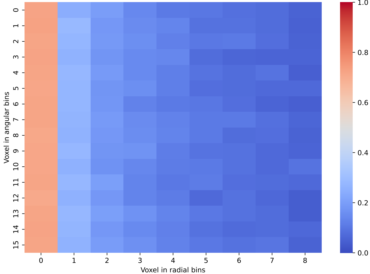
CaloScore Data: Layer 4 and 5
