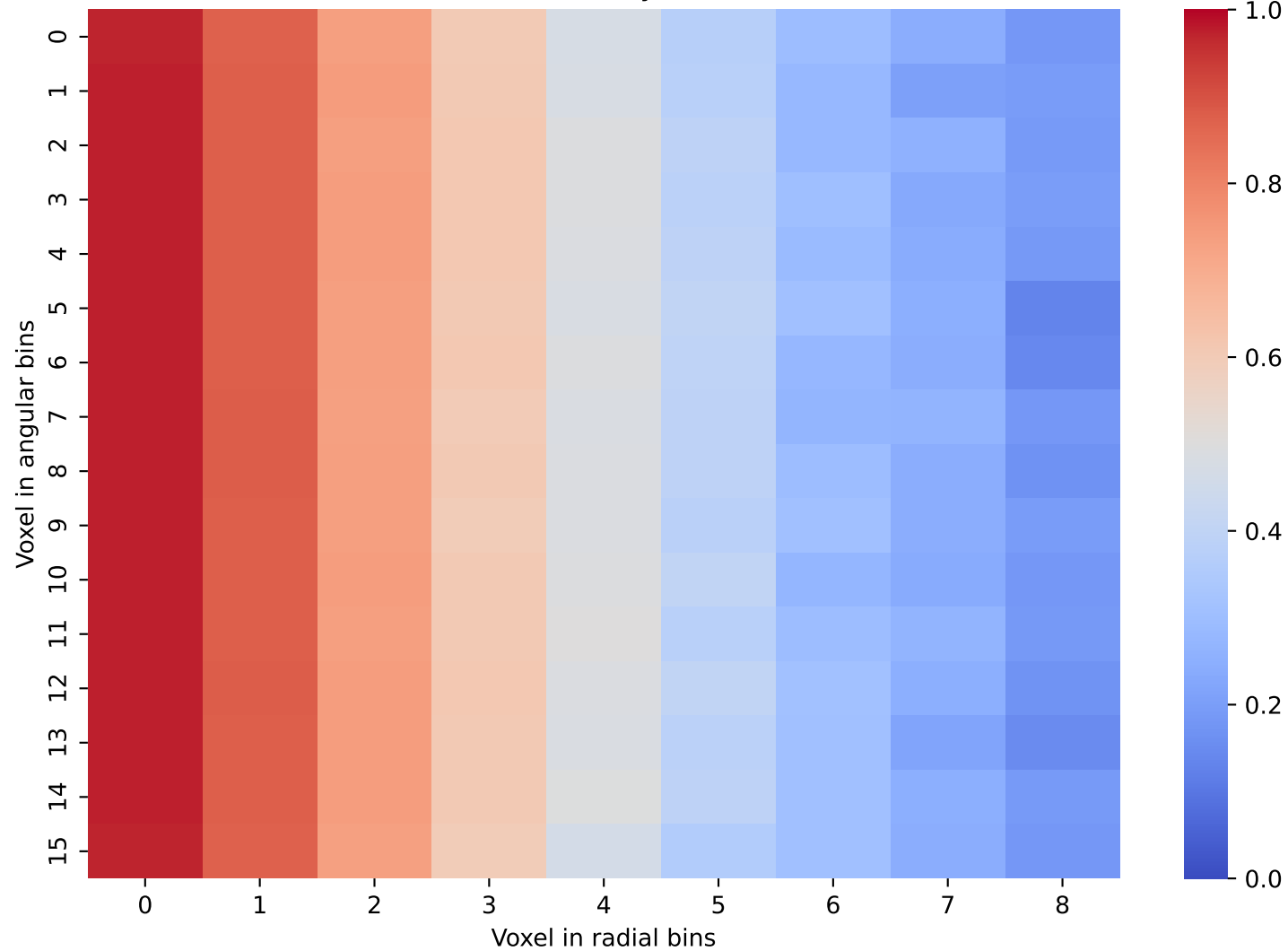
CaloScore Data: Layer 17 and 18
