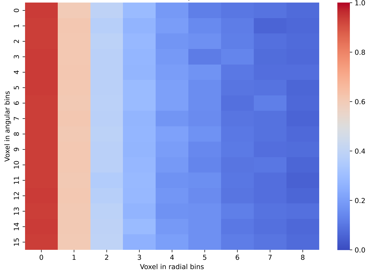
CaloScore Data: Layer 7 and 8
