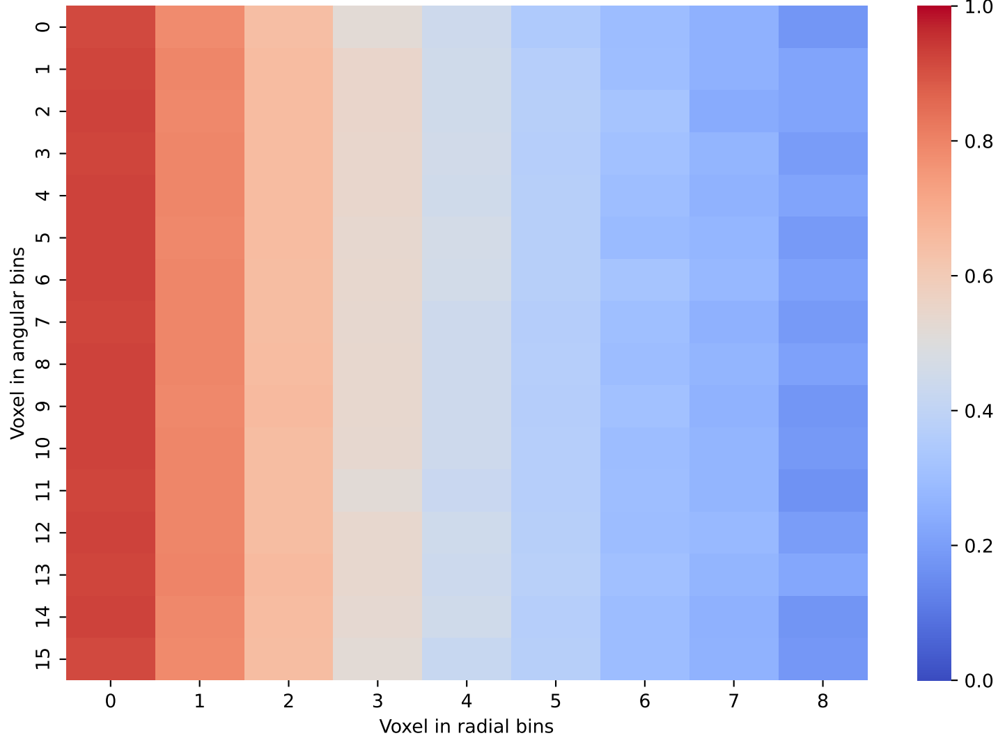
CaloScore Data: Layer 24 and 25
