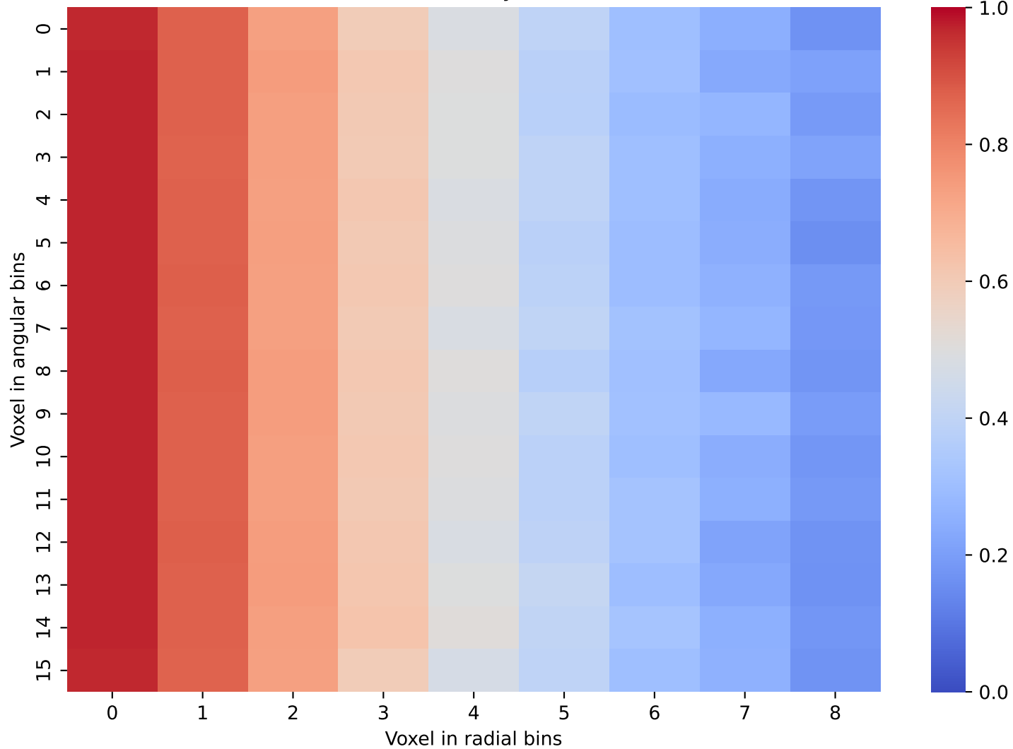
CaloScore Data: Layer 18 and 19
