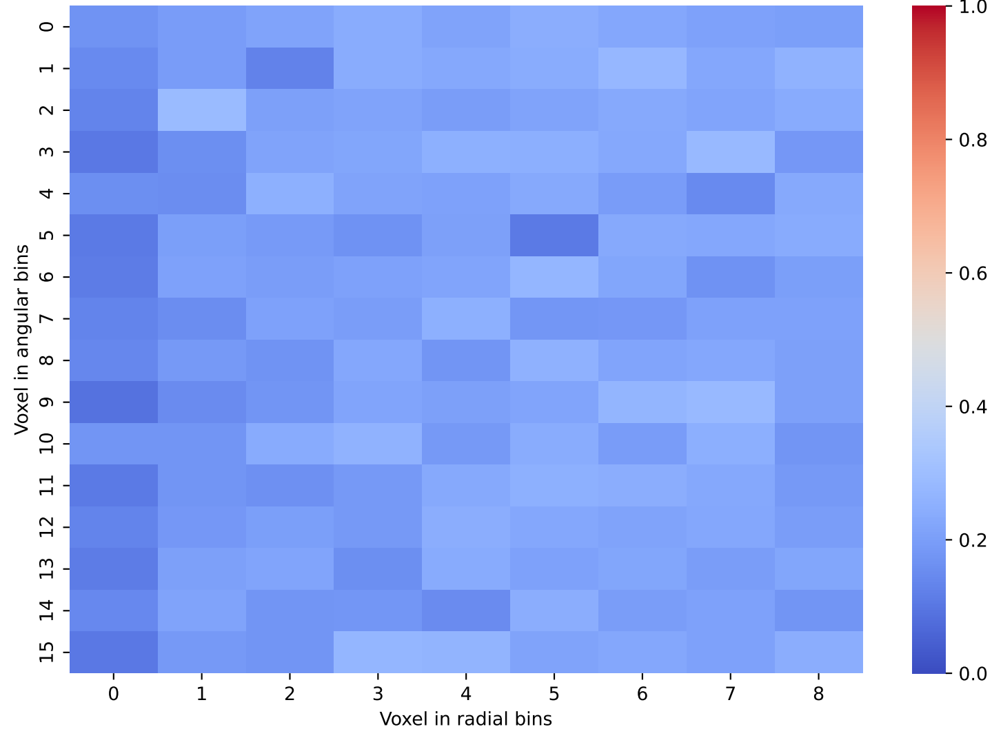
CaloScore Data: Layer 44 and 45
