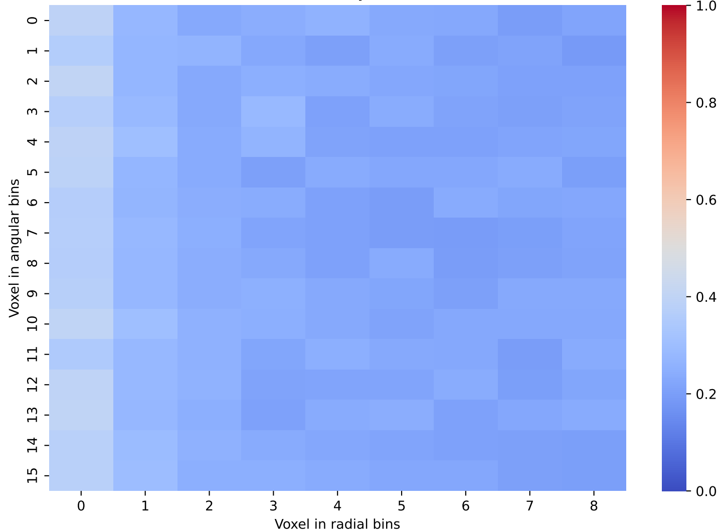
CaloScore Data: Layer 37 and 38
