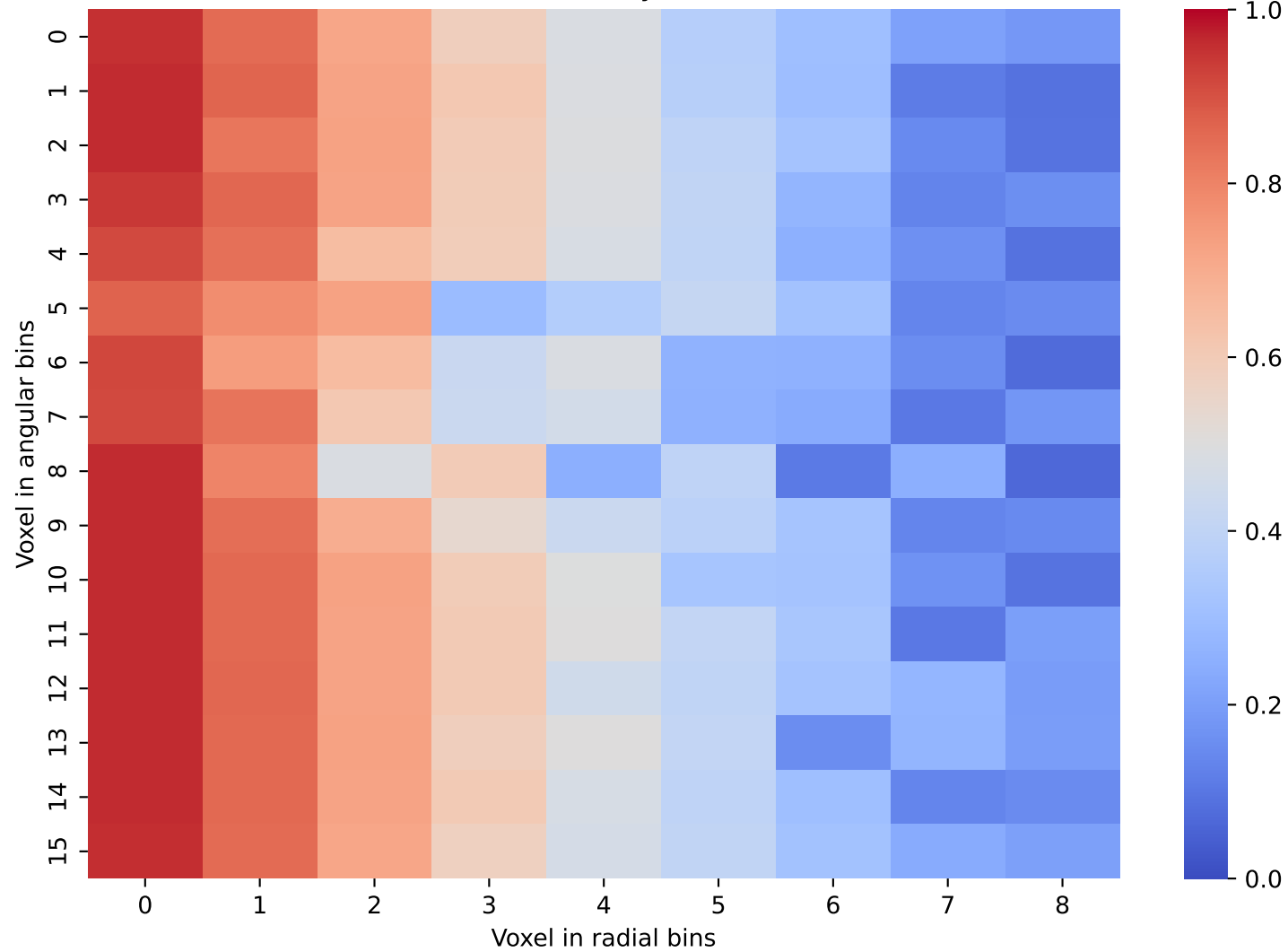
CaloScore Data: Layer 20 and 21
