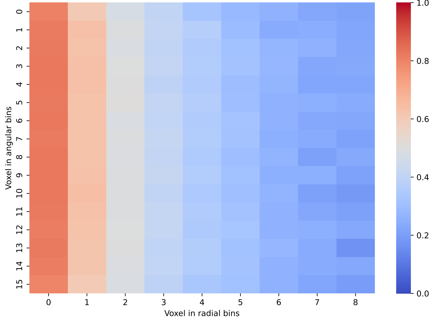
CaloScore Data: Layer 29 and 30
