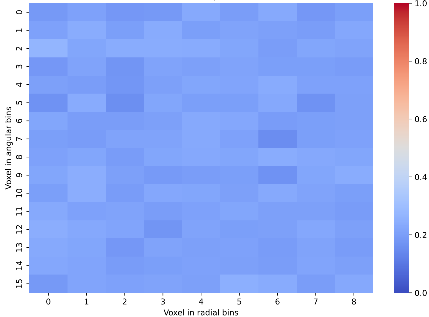
CaloScore Data: Layer 40 and 41
