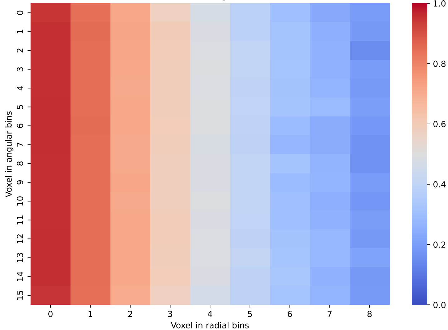
CaloScore Data: Layer 21 and 22
