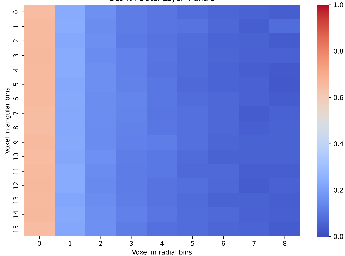
Geant4 Data: Layer 4 and 5
