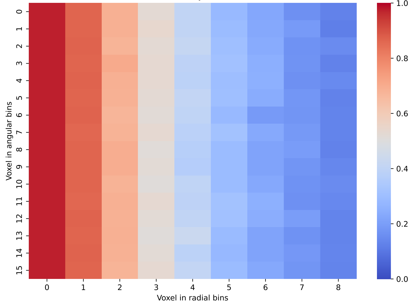
Geant4 Data: Layer 15 and 16
