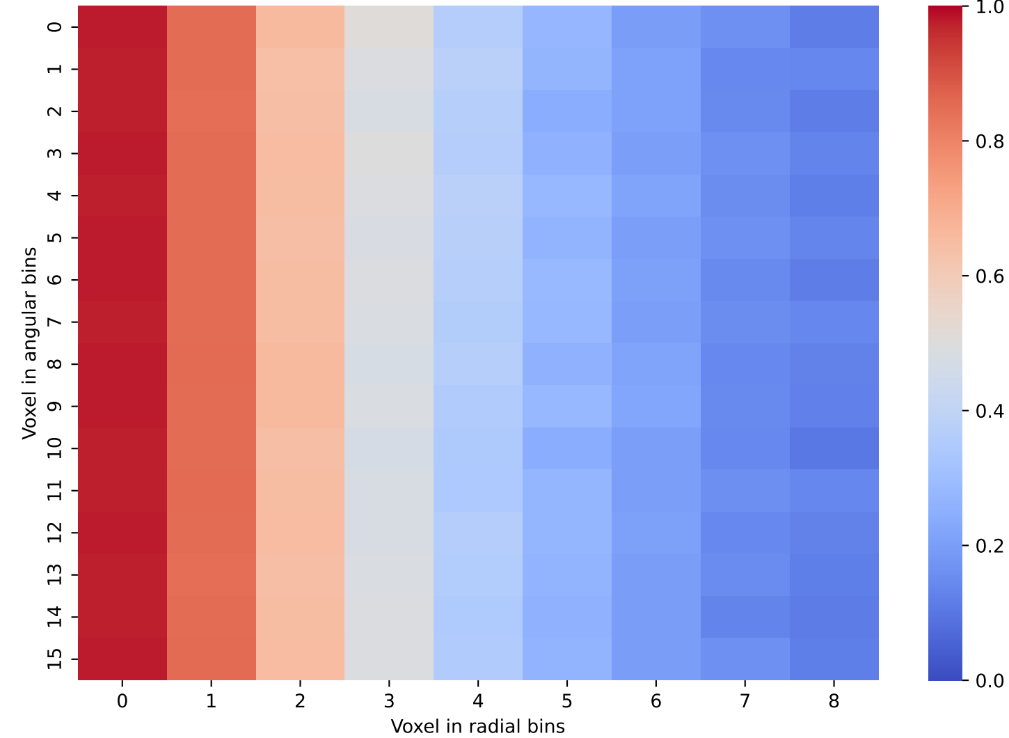
Geant4 Data: Layer 13 and 14
