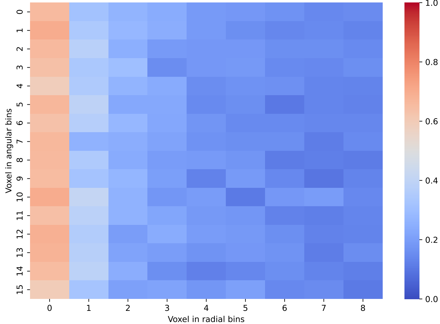
Geant4 Data: Layer 34 and 35
