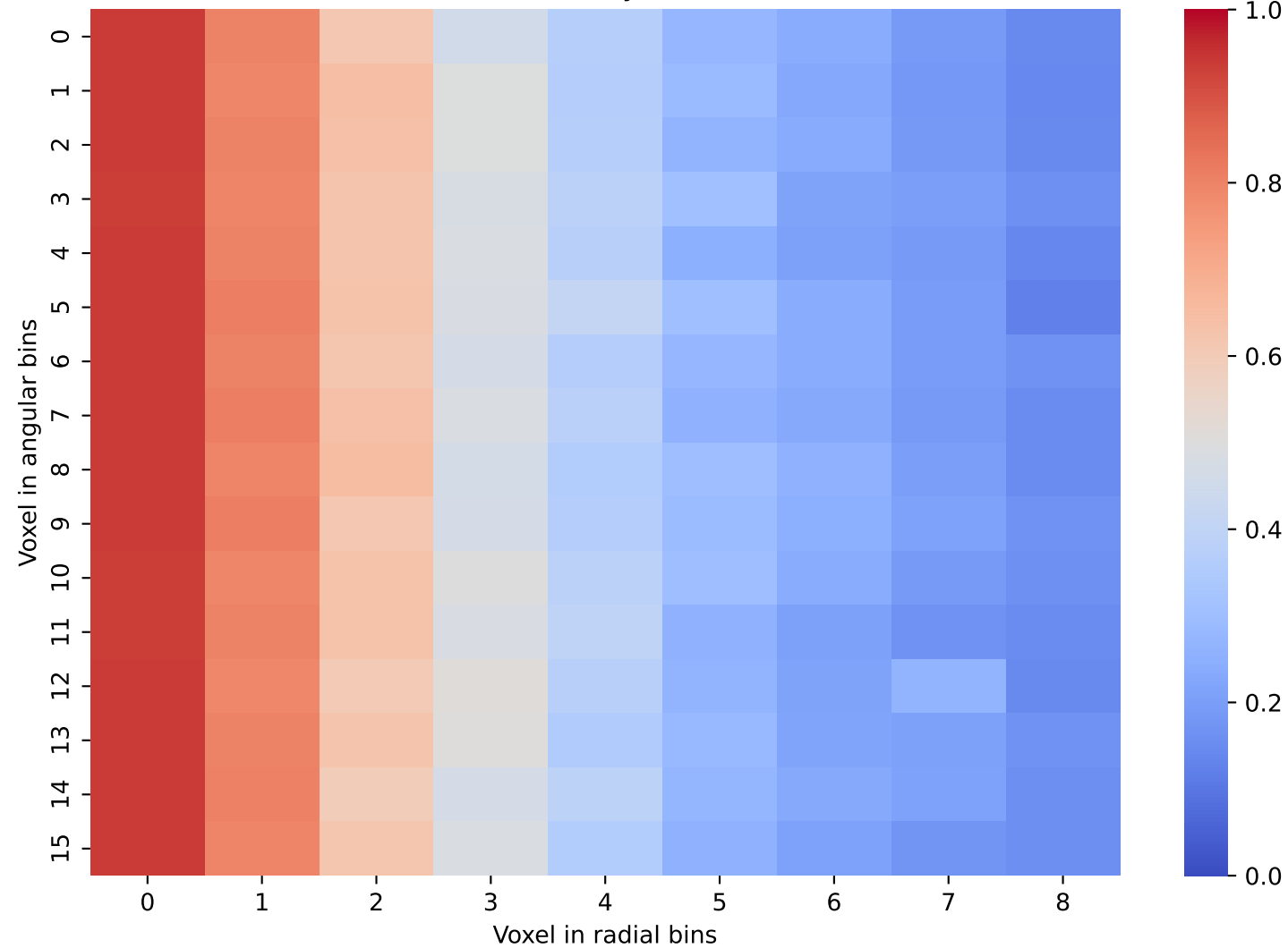
Geant4 Data: Layer 23 and 24
