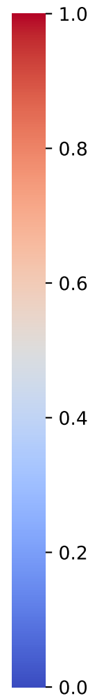
Geant4 Data: Layer 9 and 10 Voxel in angular bins Voxel in radial bins 0.0 0.2 0.4 0.6 0.8 1.0
