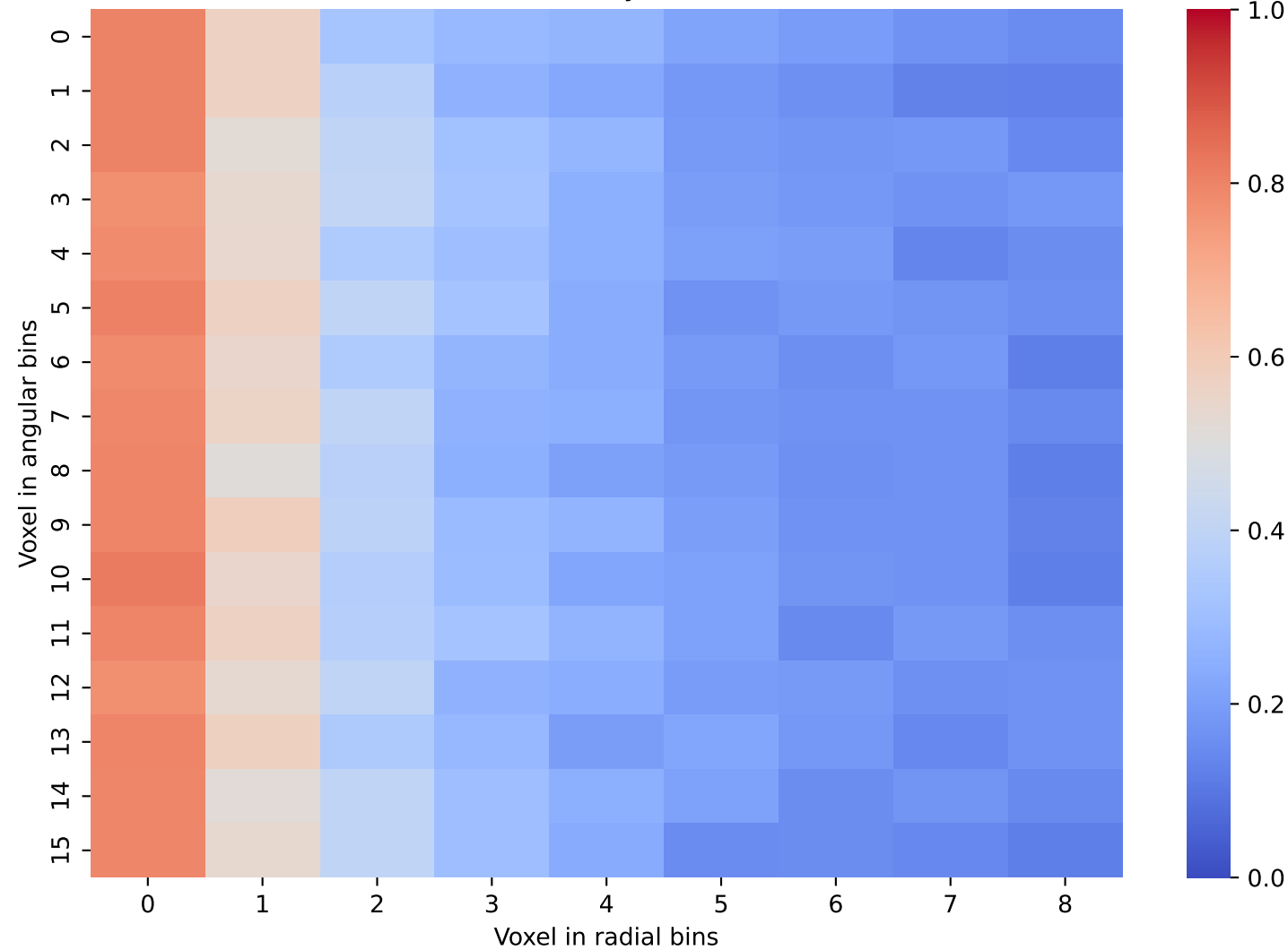
Geant4 Data: Layer 30 and 31
