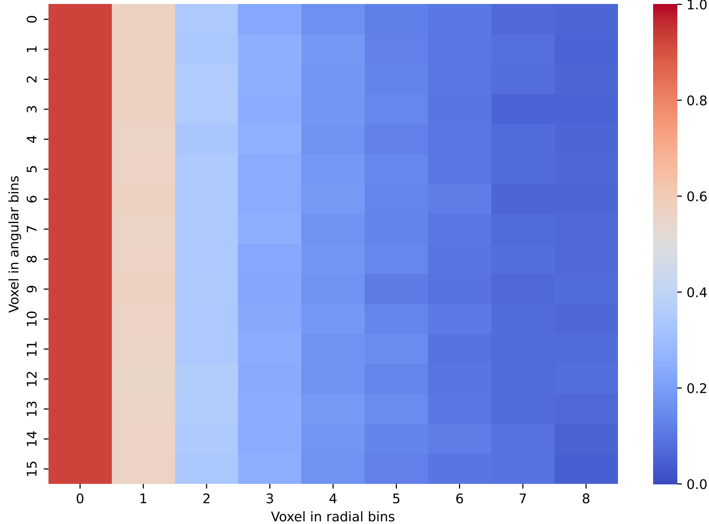
Geant4 Data: Layer 7 and 8
