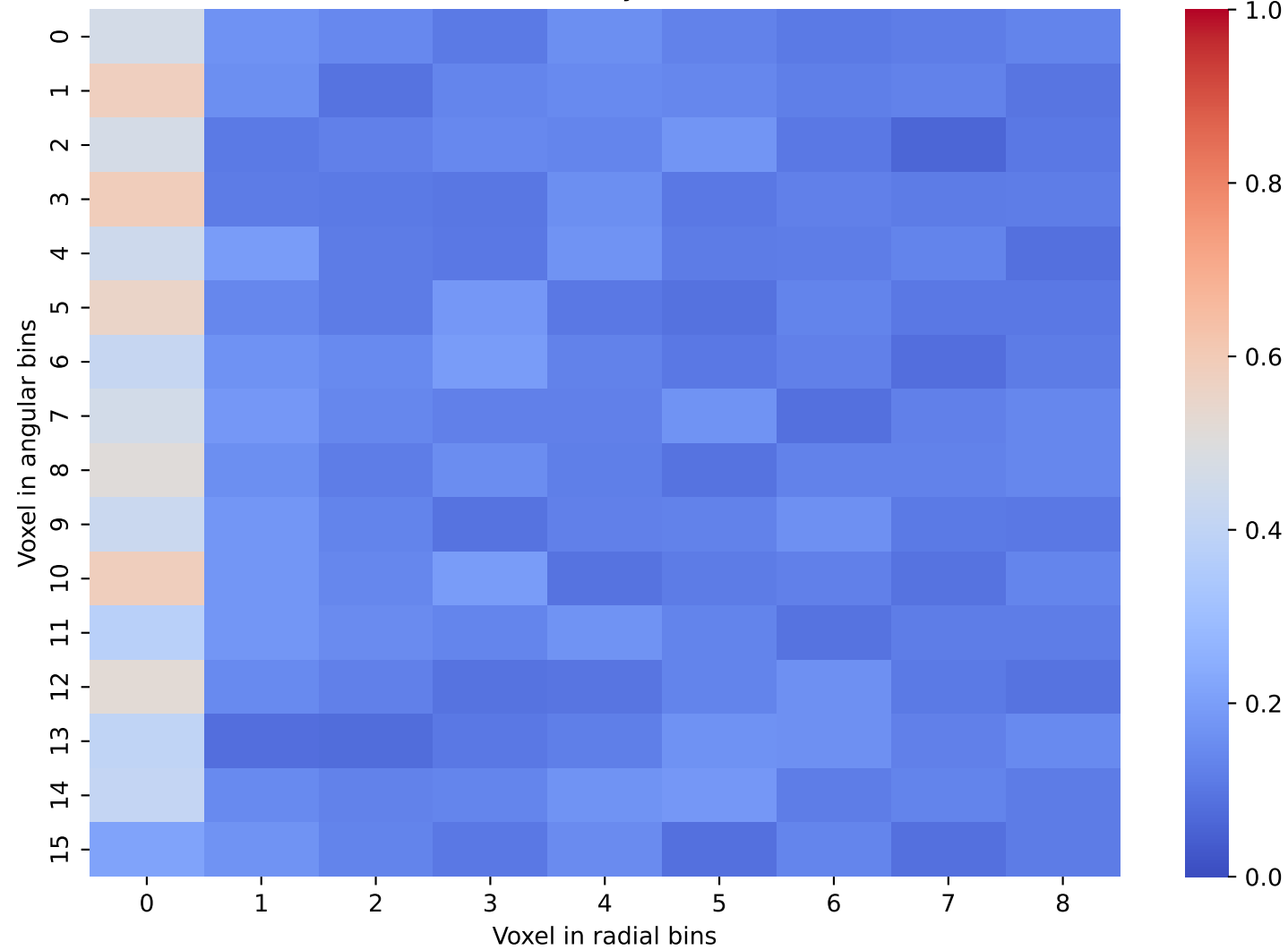
Geant4 Data: Layer 42 and 43
