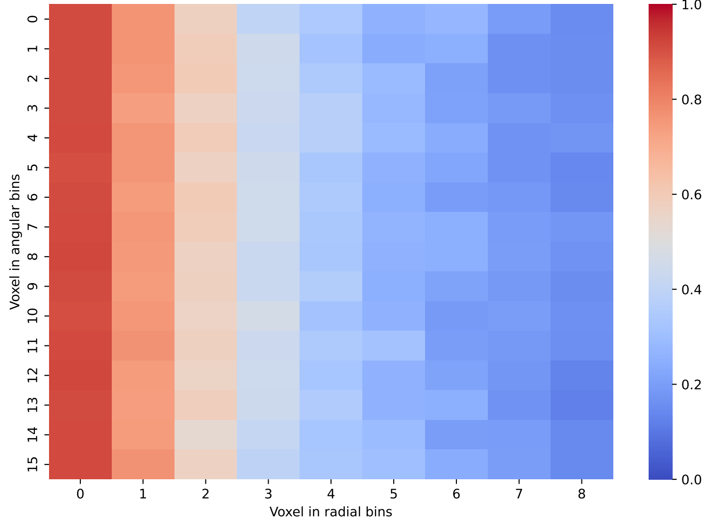
Geant4 Data: Layer 25 and 26
