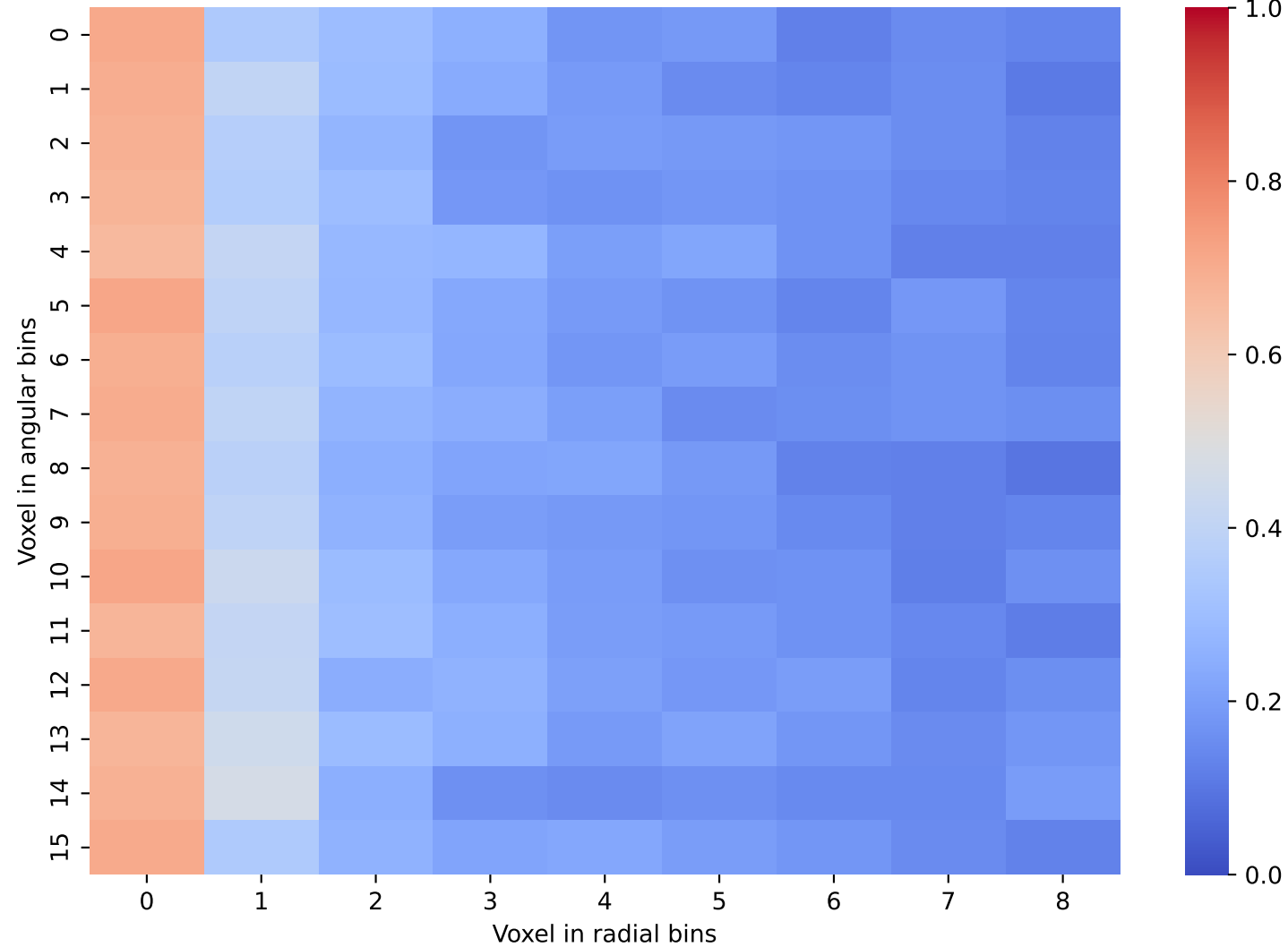
Geant4 Data: Layer 33 and 34
