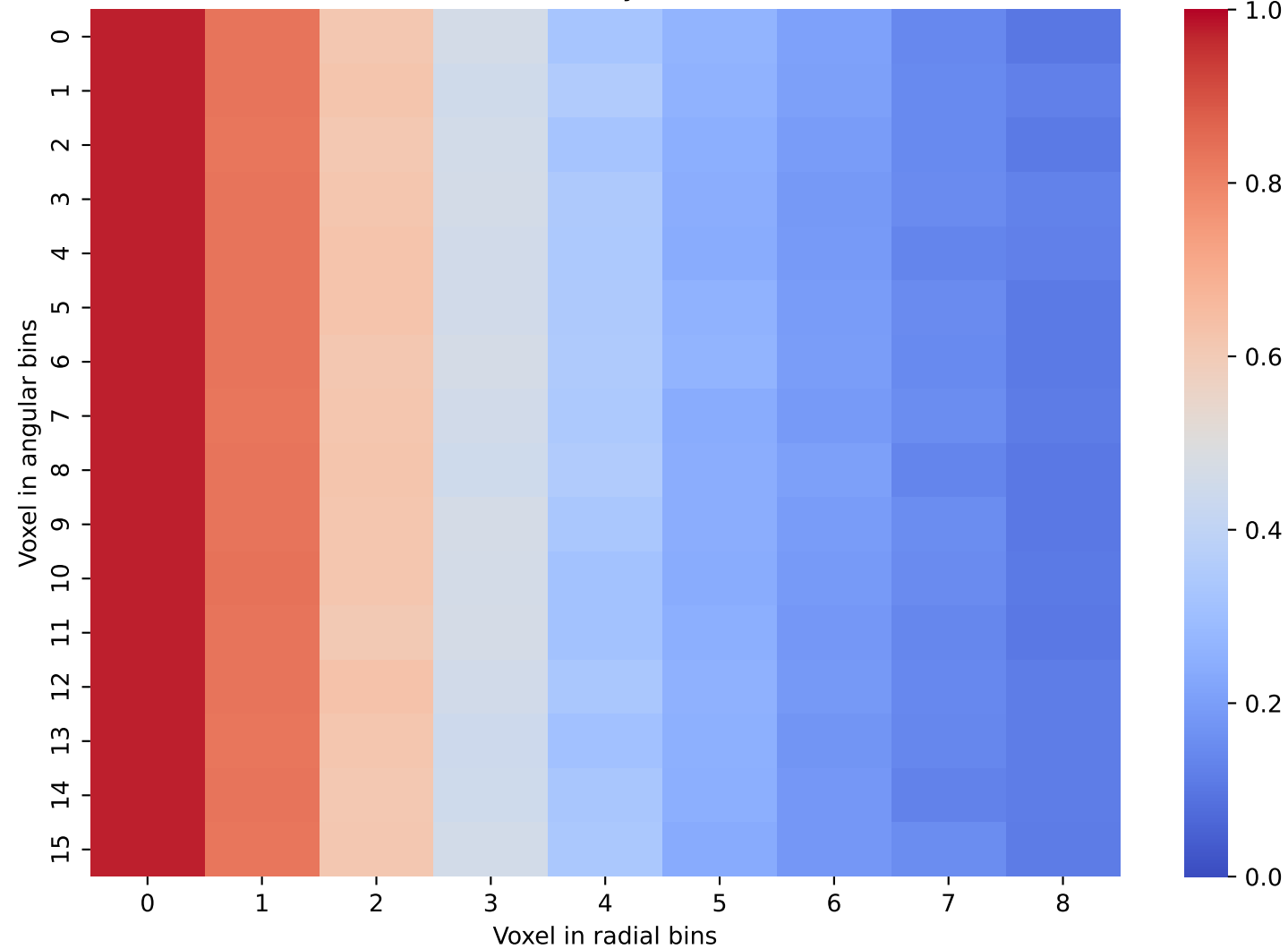
Geant4 Data: Layer 12 and 13
