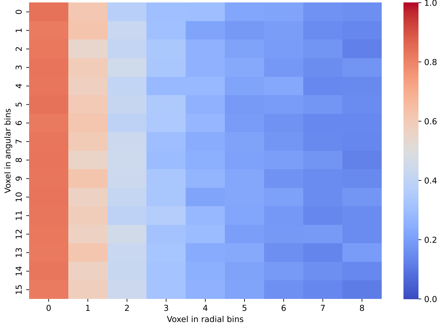
Geant4 Data: Layer 29 and 30
