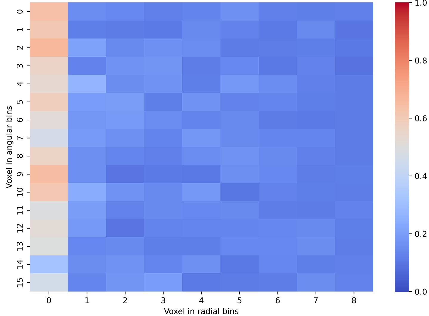
Geant4 Data: Layer 40 and 41
