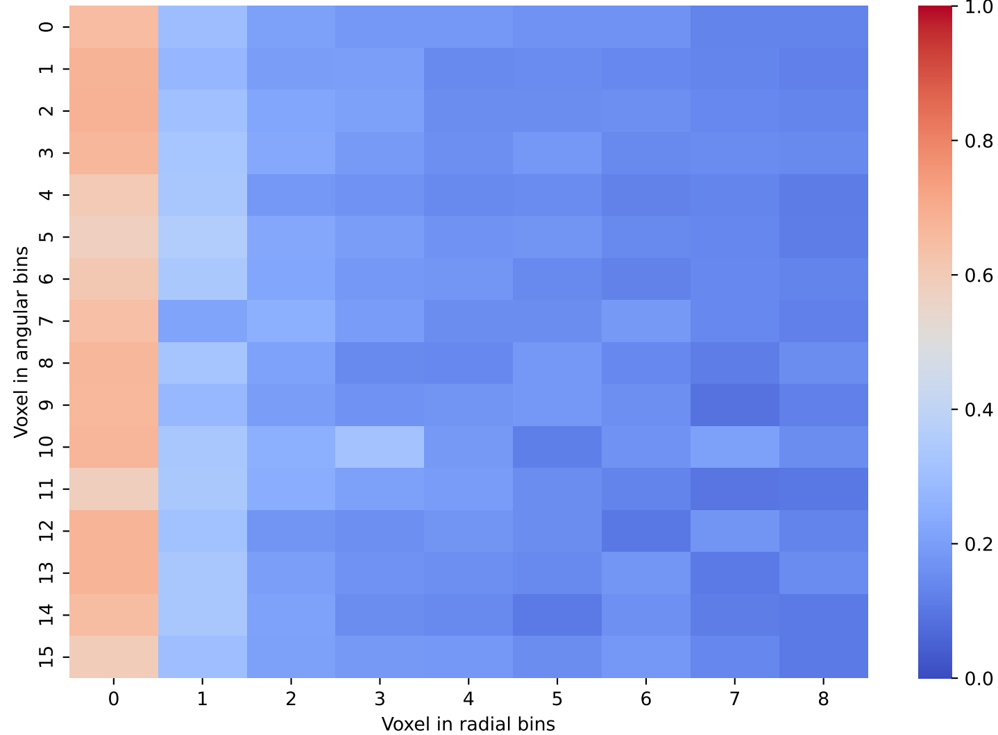
Geant4 Data: Layer 35 and 36
