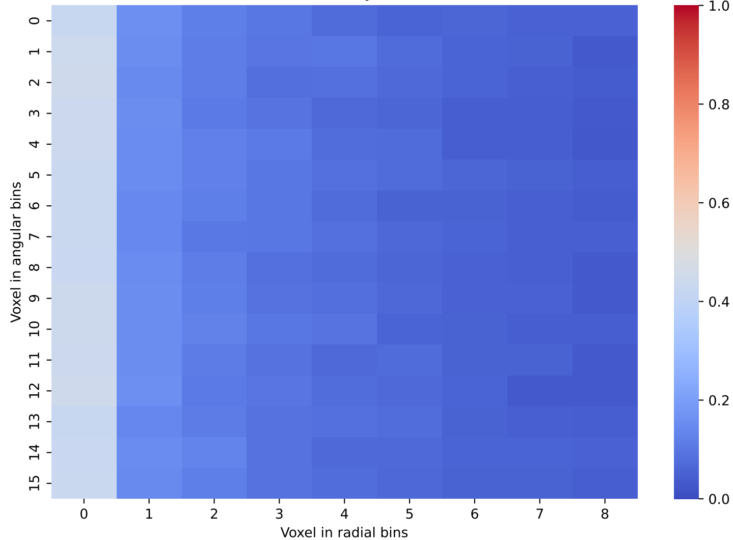
Geant4 Data: Layer 3 and 4
