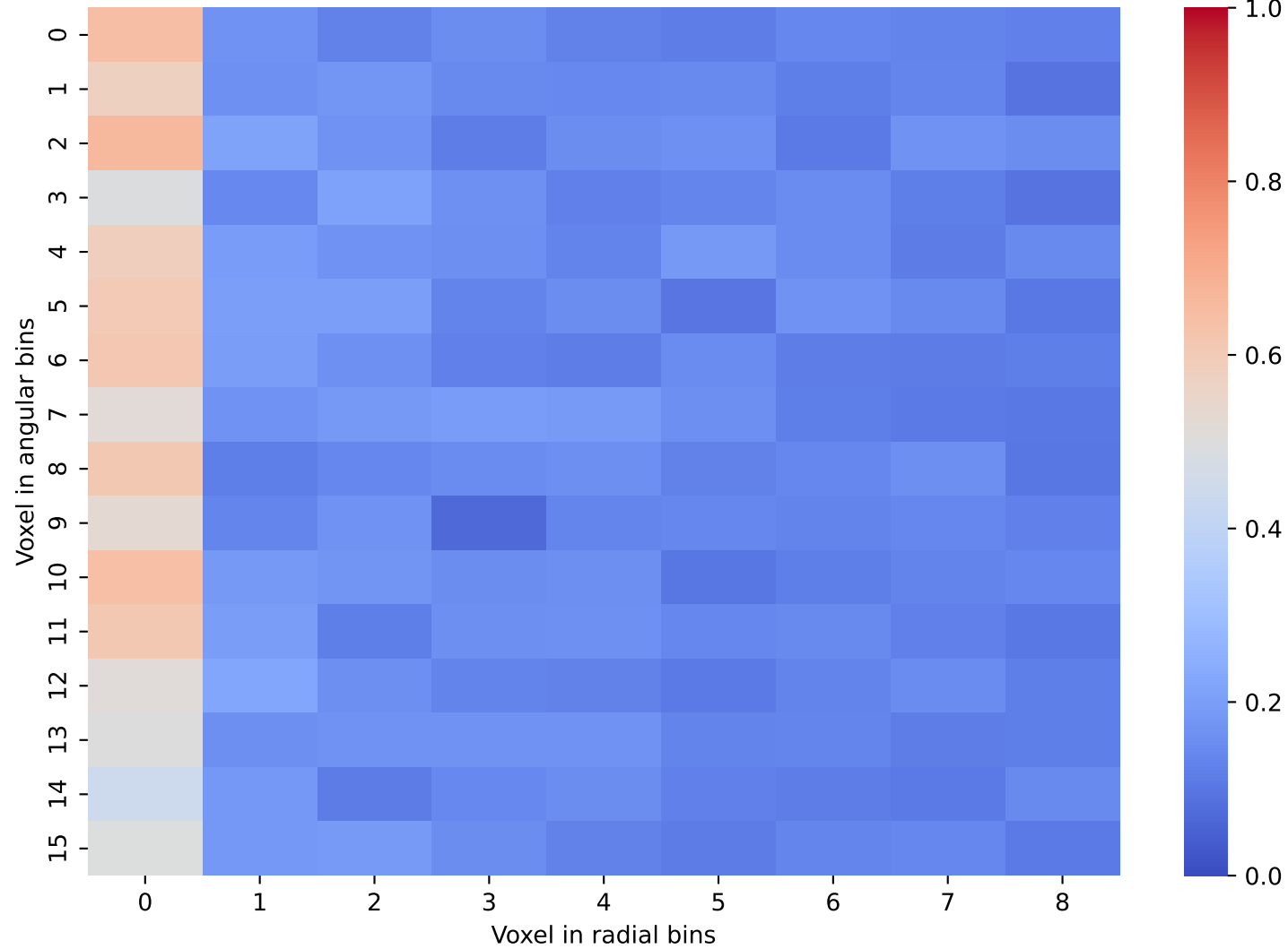
Geant4 Data: Layer 39 and 40
