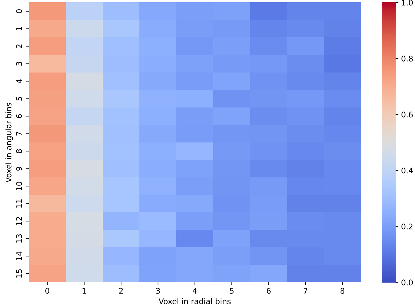
Geant4 Data: Layer 32 and 33
