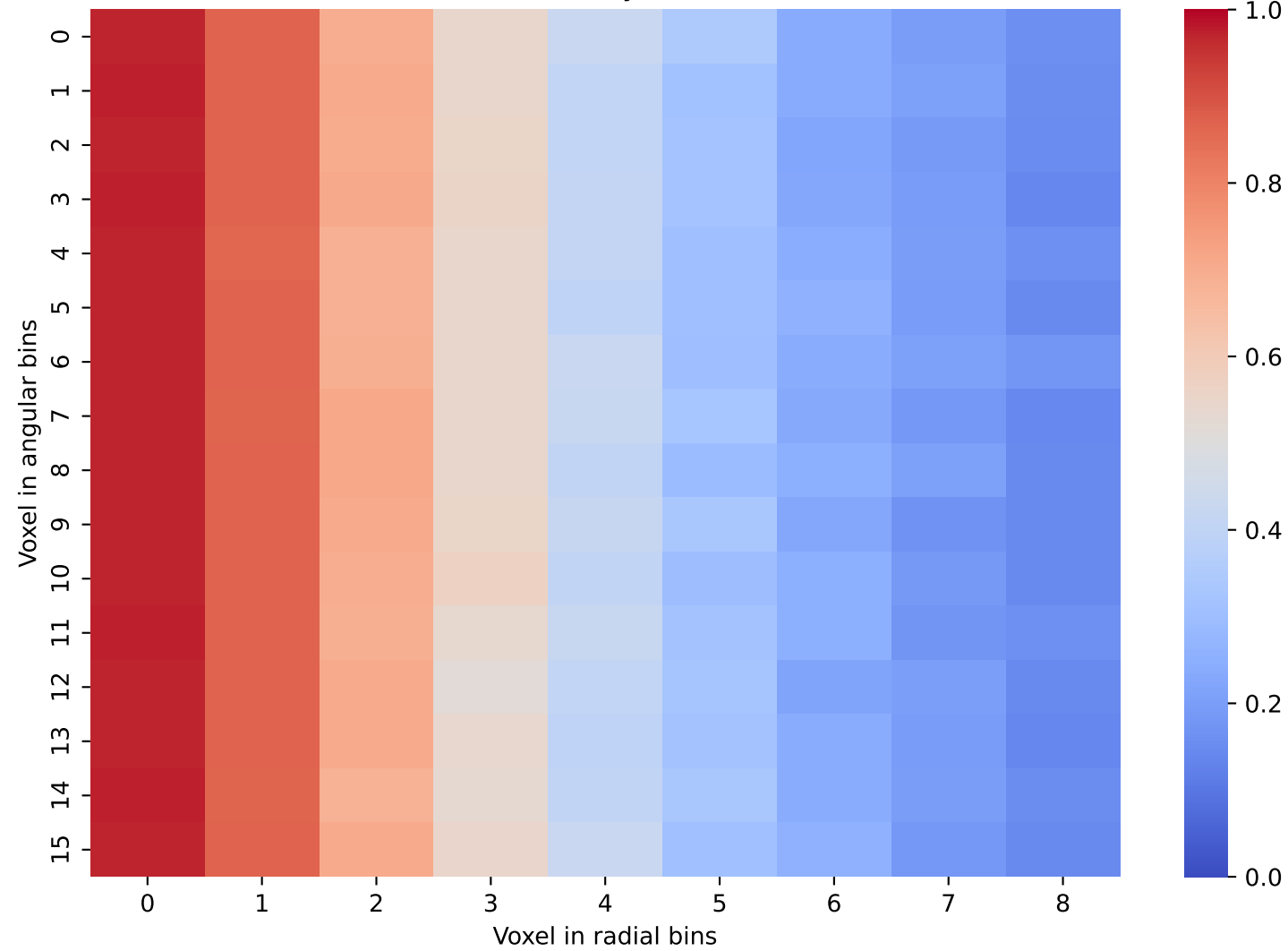
Geant4 Data: Layer 17 and 18
