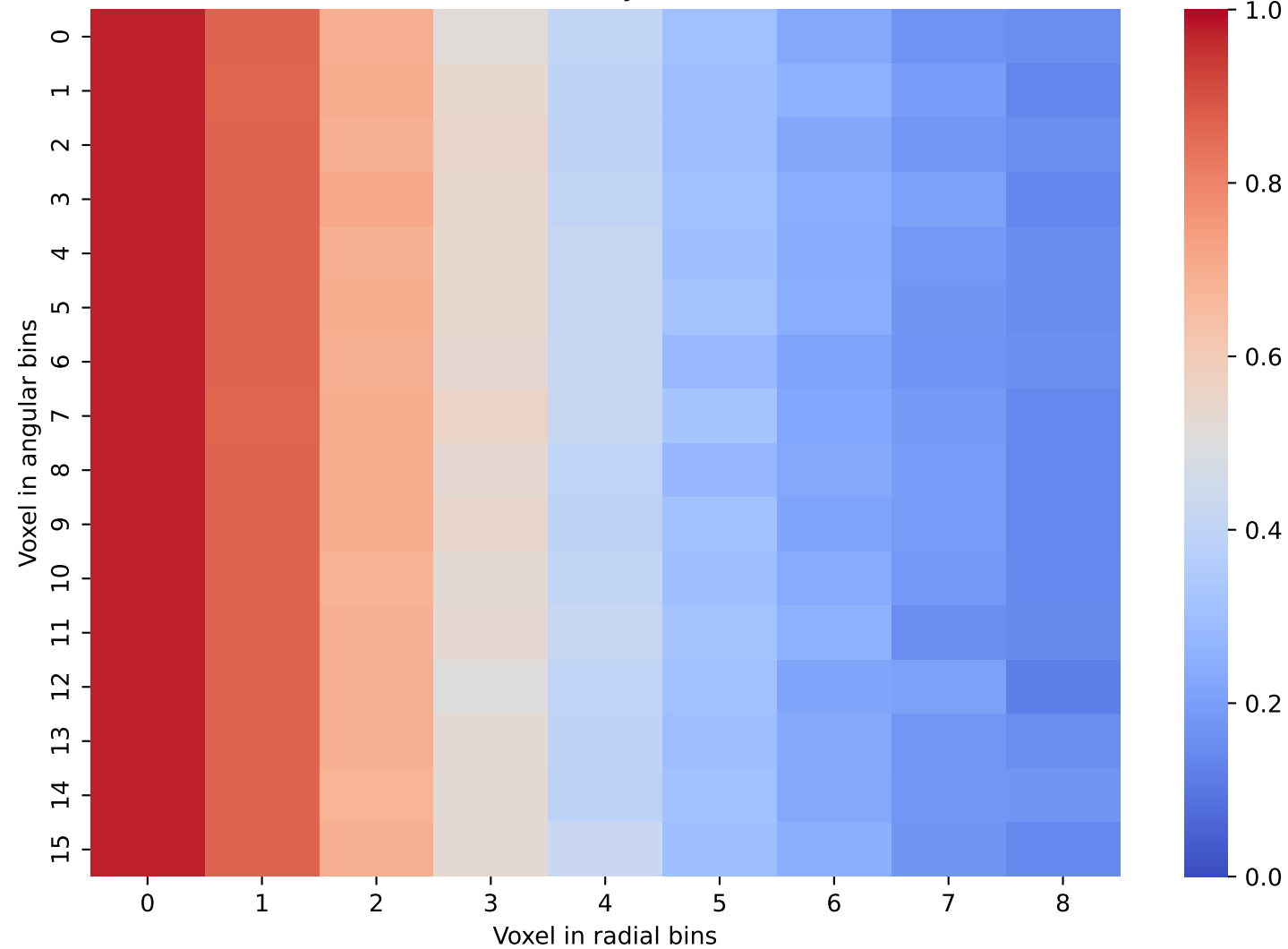
Geant4 Data: Layer 16 and 17
