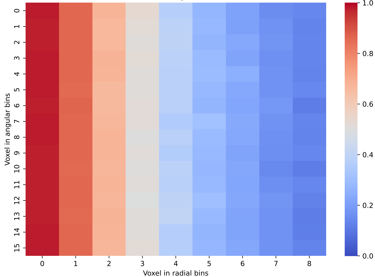
Geant4 Data: Layer 14 and 15
