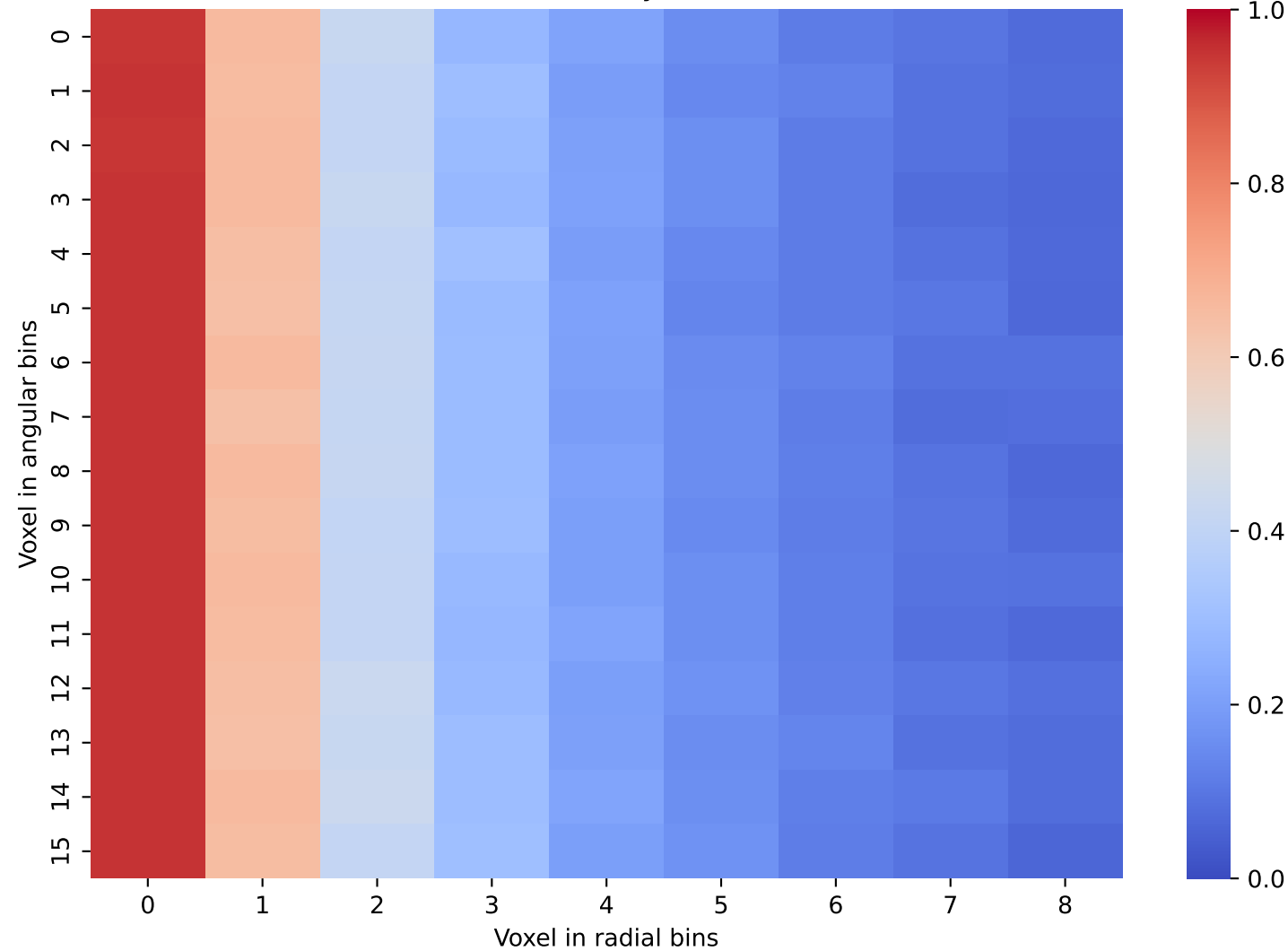
Geant4 Data: Layer 8 and 9
