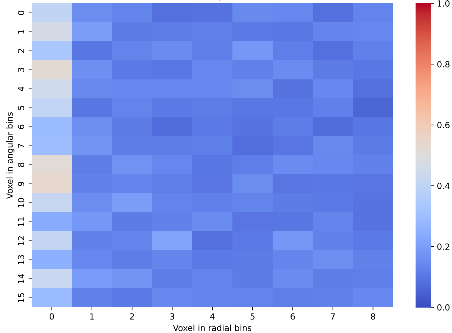
Geant4 Data: Layer 43 and 44
