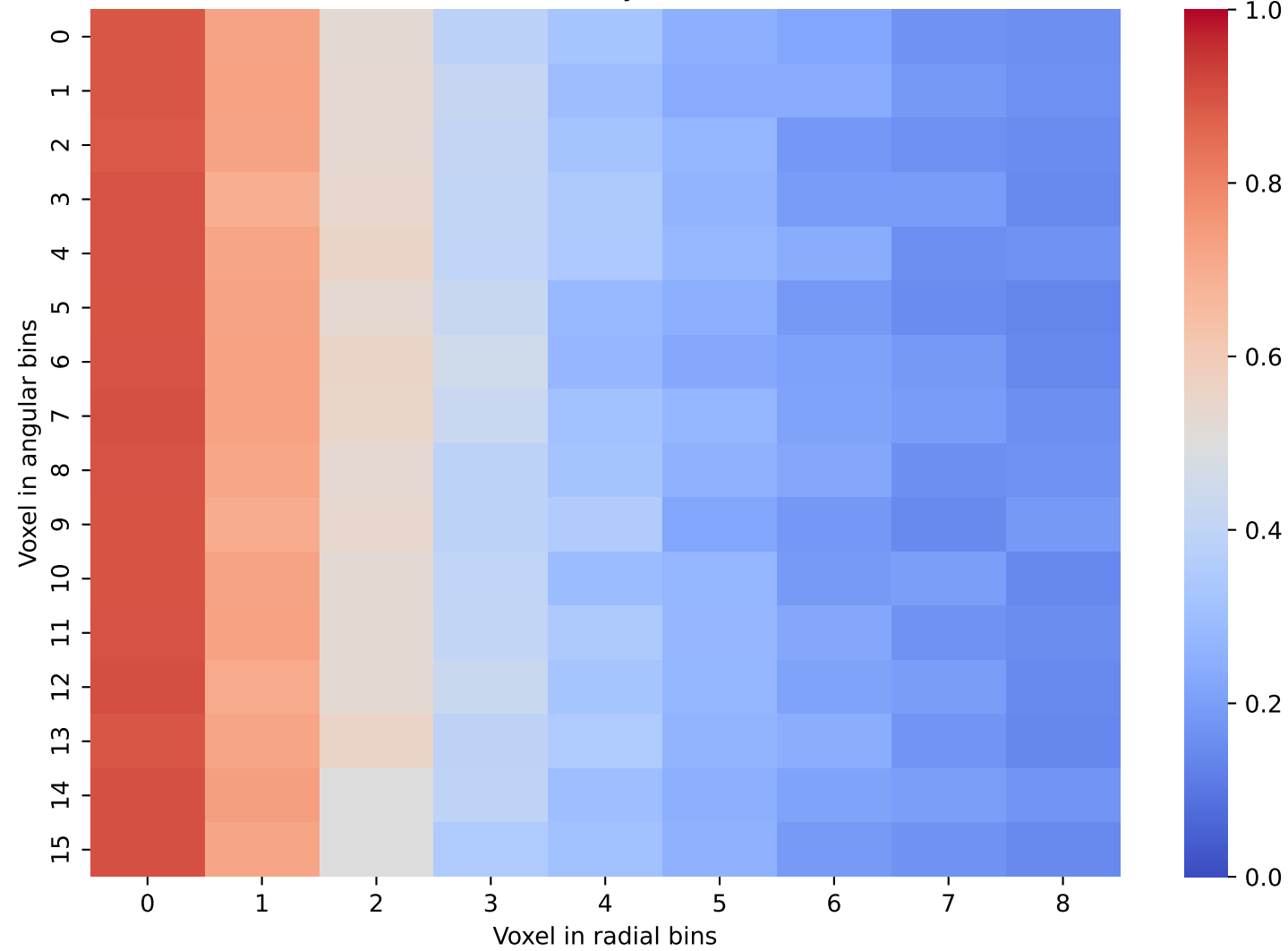
Geant4 Data: Layer 26 and 27
