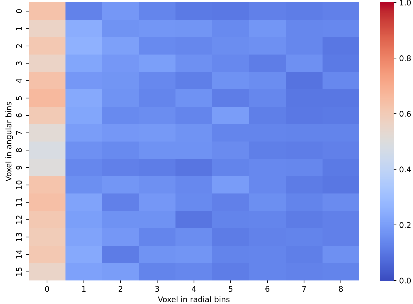
Geant4 Data: Layer 38 and 39
