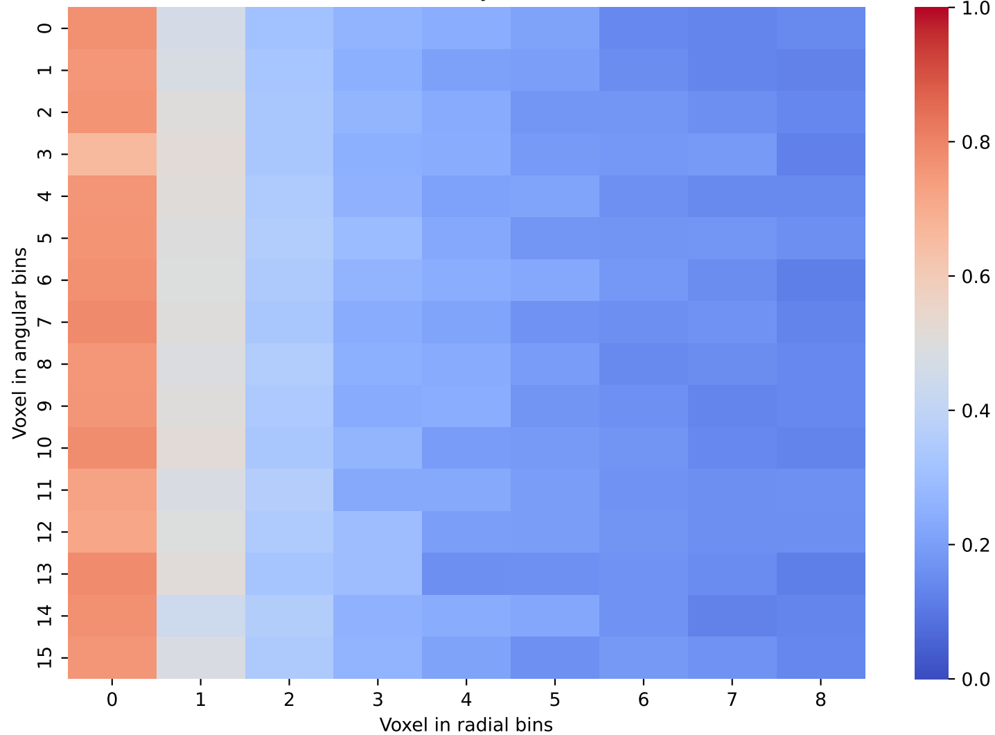
Geant4 Data: Layer 31 and 32
