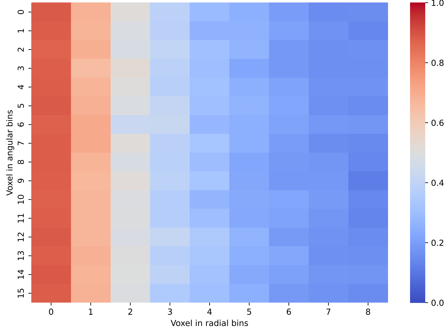
Geant4 Data: Layer 27 and 28
