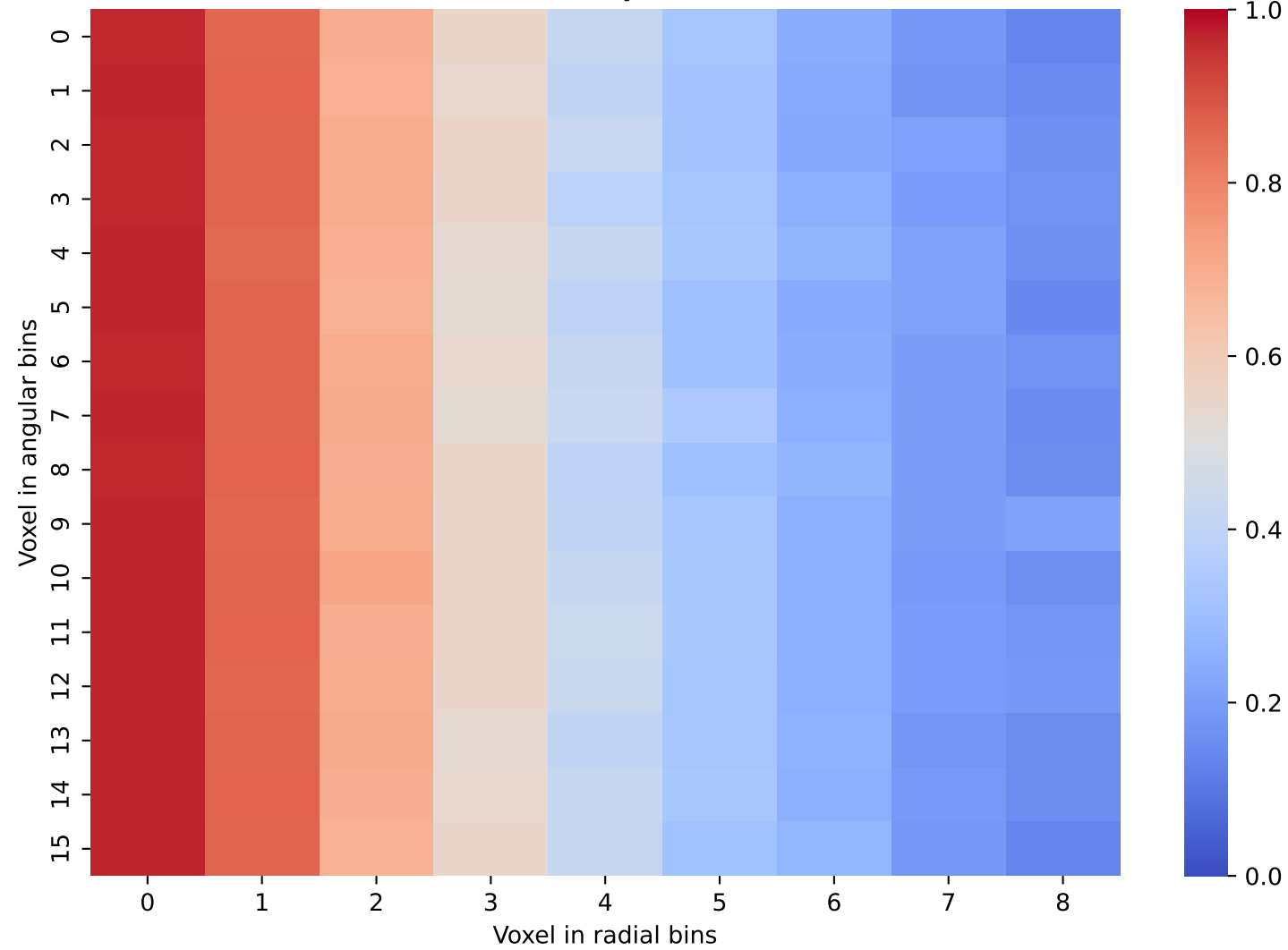
Geant4 Data: Layer 18 and 19
