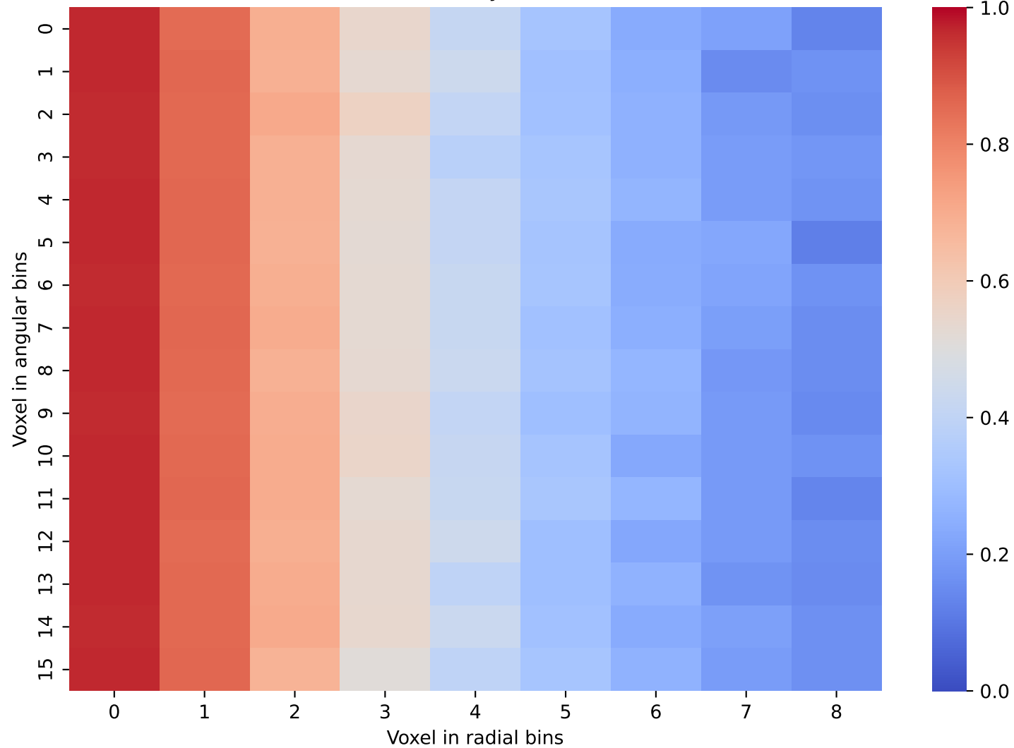
Geant4 Data: Layer 19 and 20
