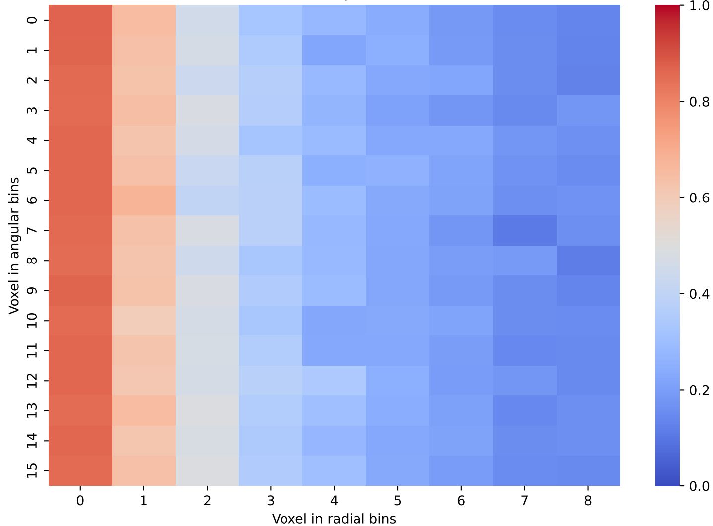
Geant4 Data: Layer 28 and 29
