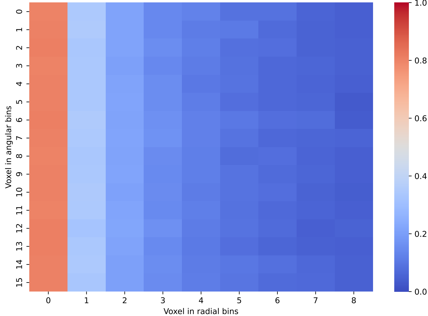
Geant4 Data: Layer 5 and 6
