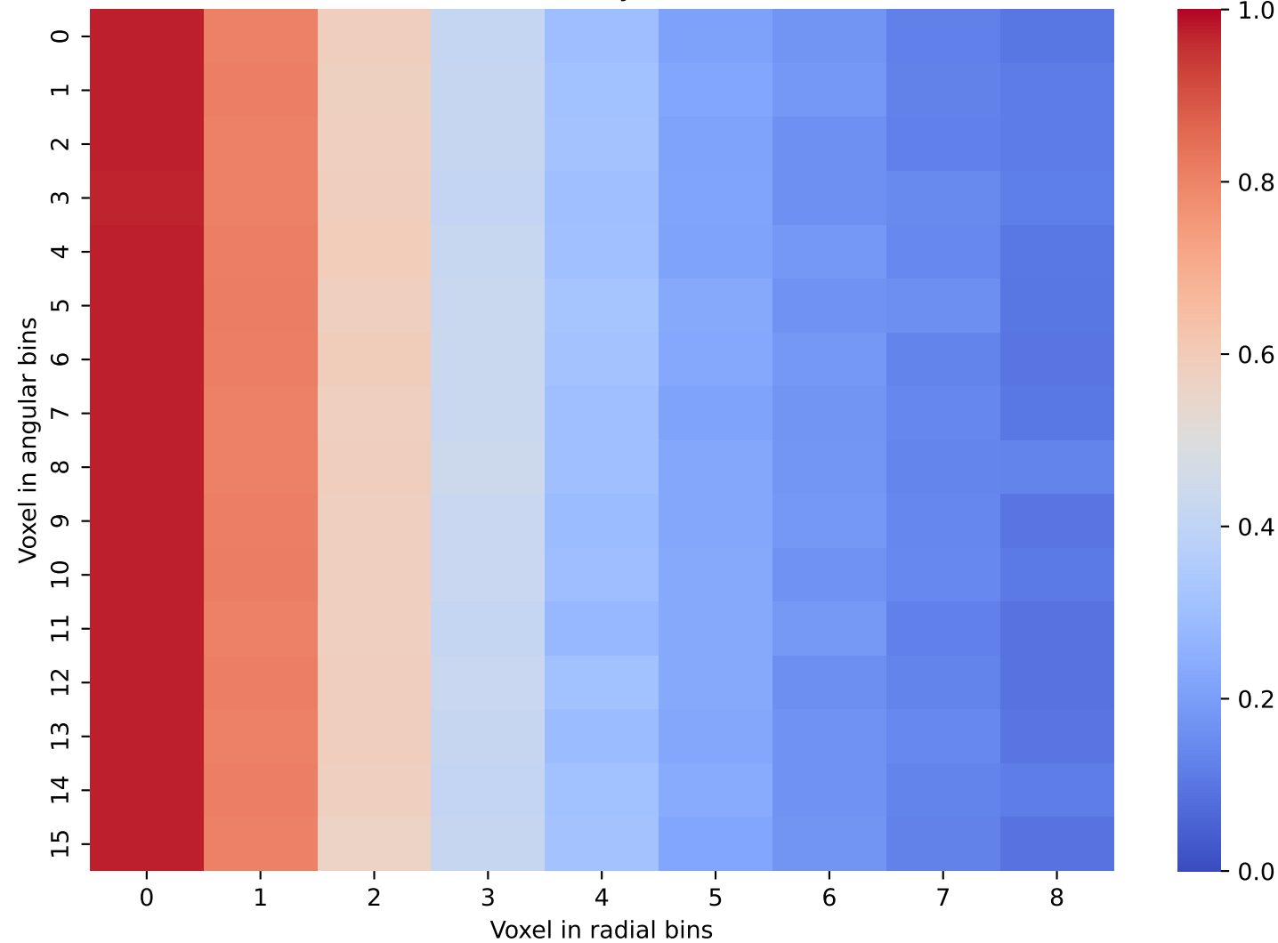
Geant4 Data: Layer 11 and 12
