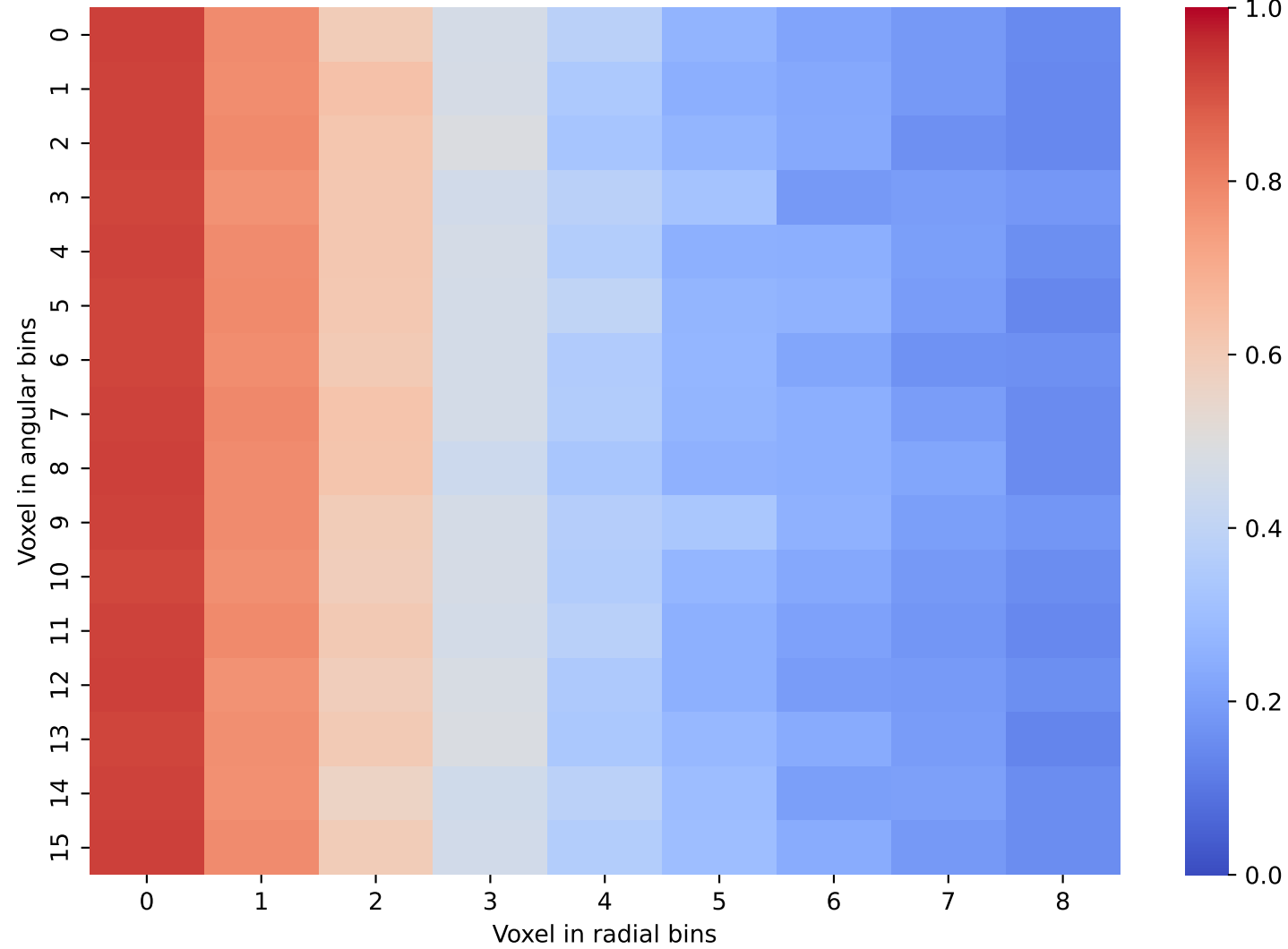
Geant4 Data: Layer 24 and 25
