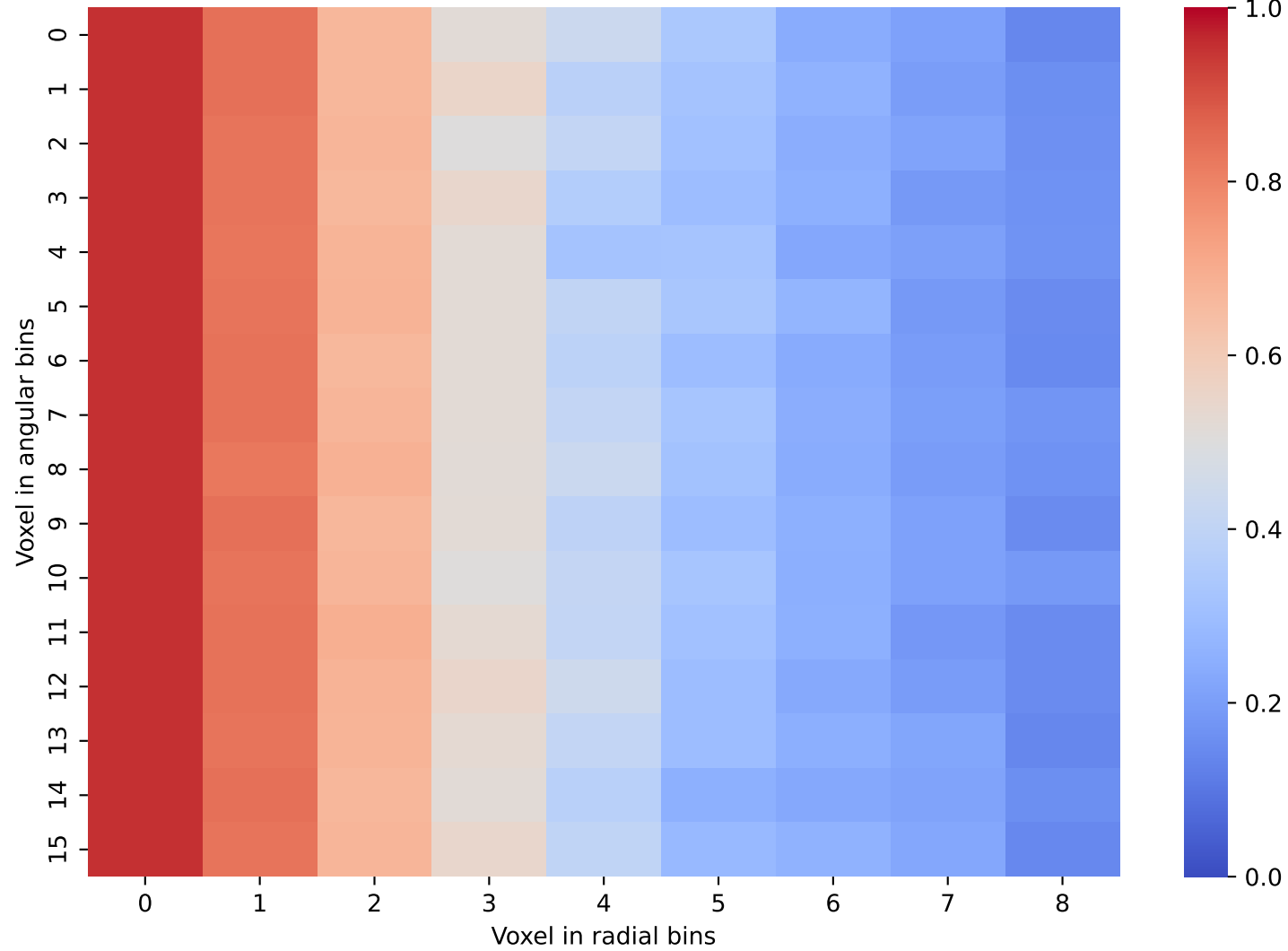
Geant4 Data: Layer 21 and 22
