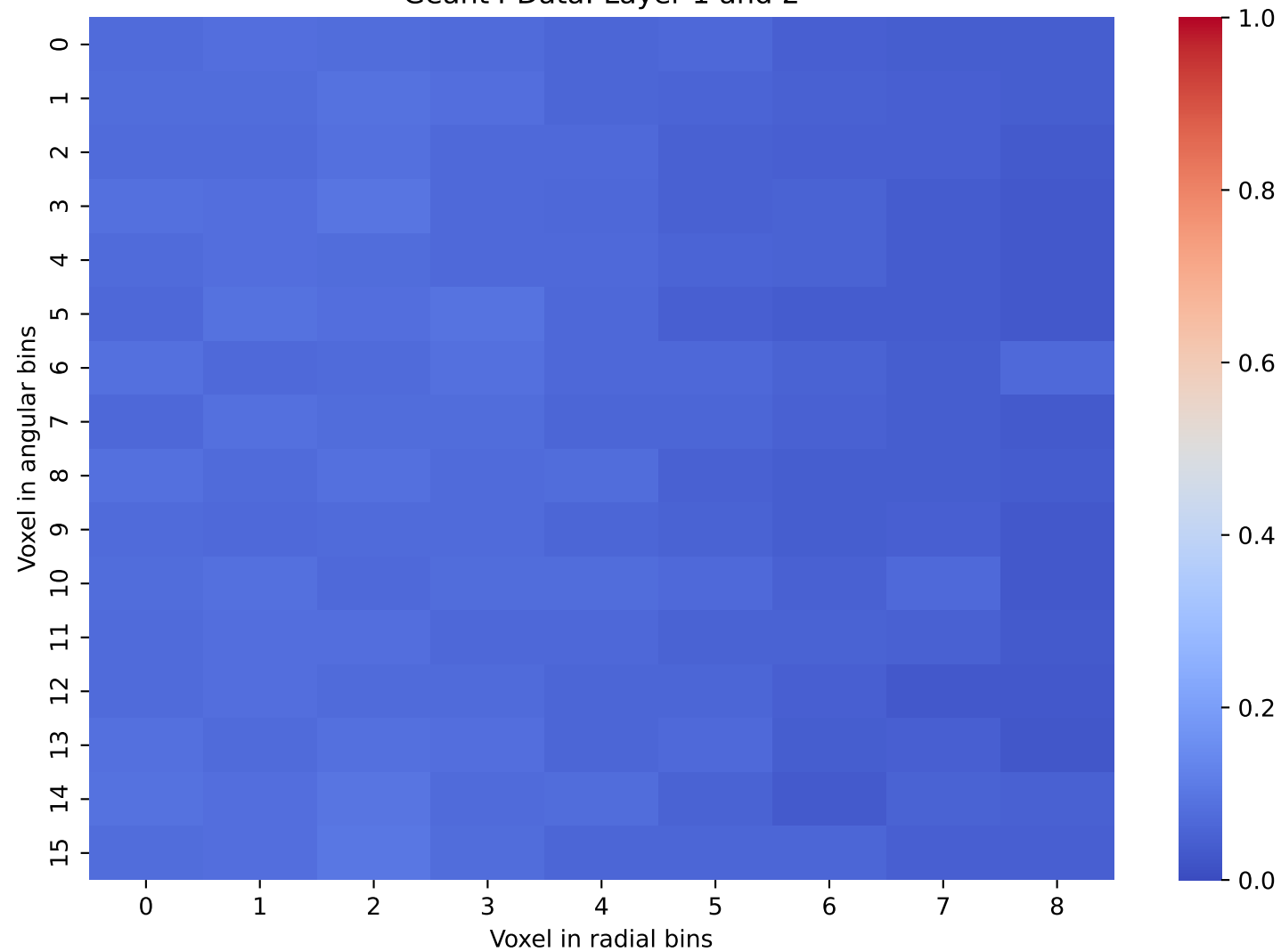
Geant4 Data: Layer 1 and 2
