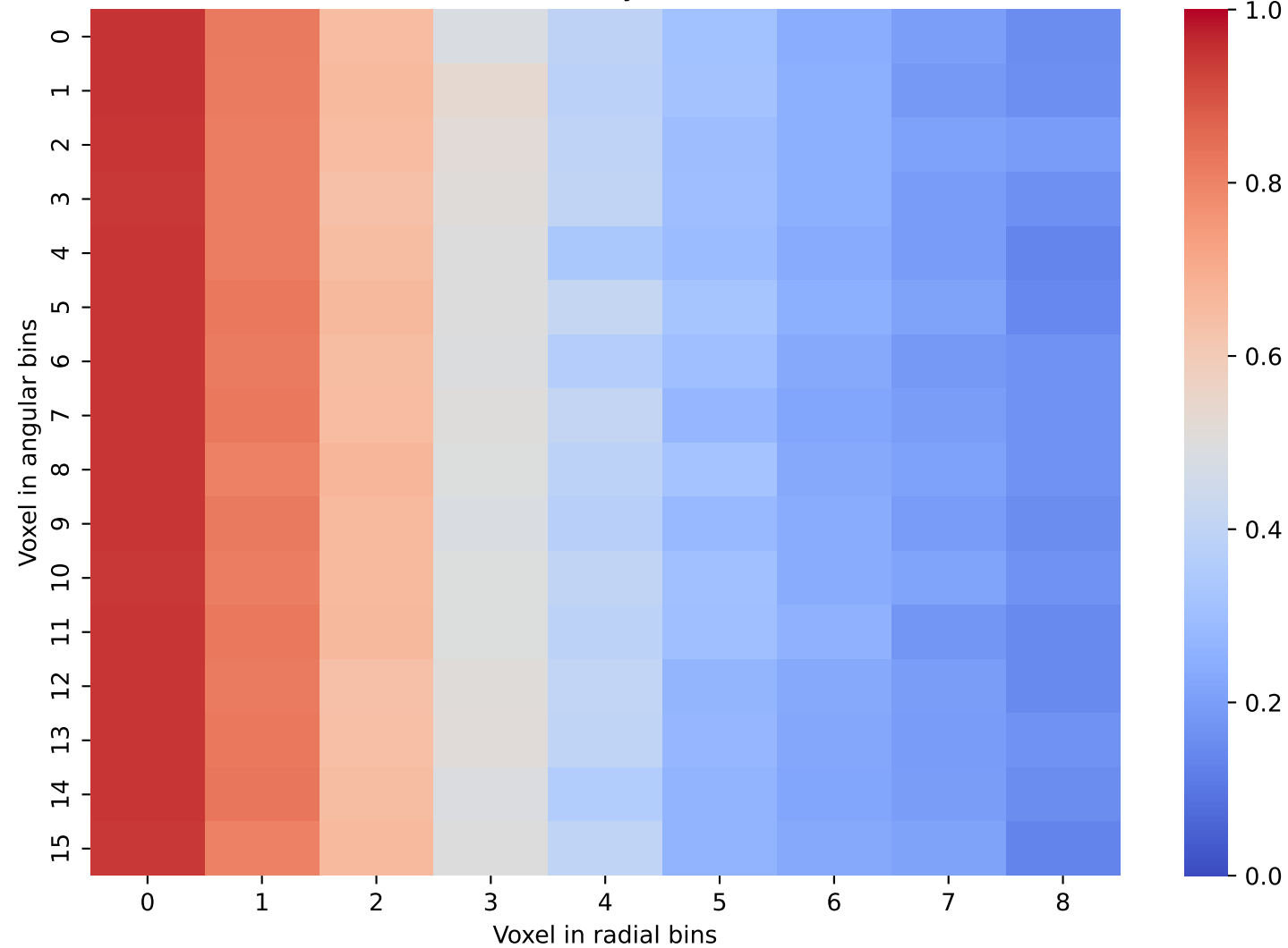
Geant4 Data: Layer 22 and 23
