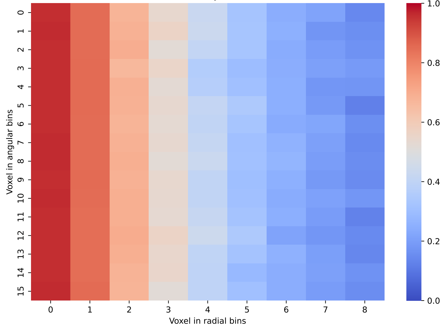
Geant4 Data: Layer 20 and 21
