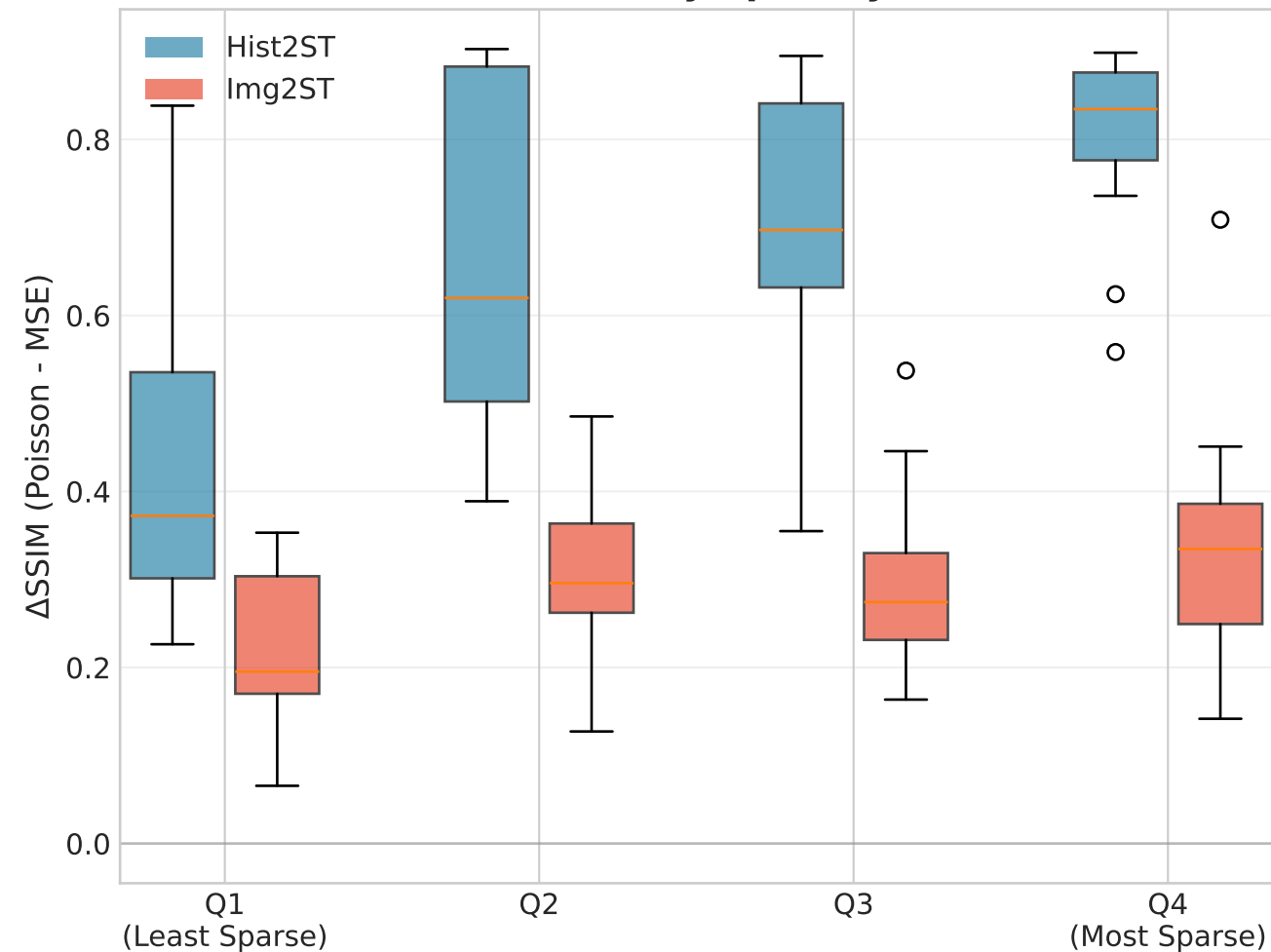
Poisson Benefit by Sparsity Quartile
