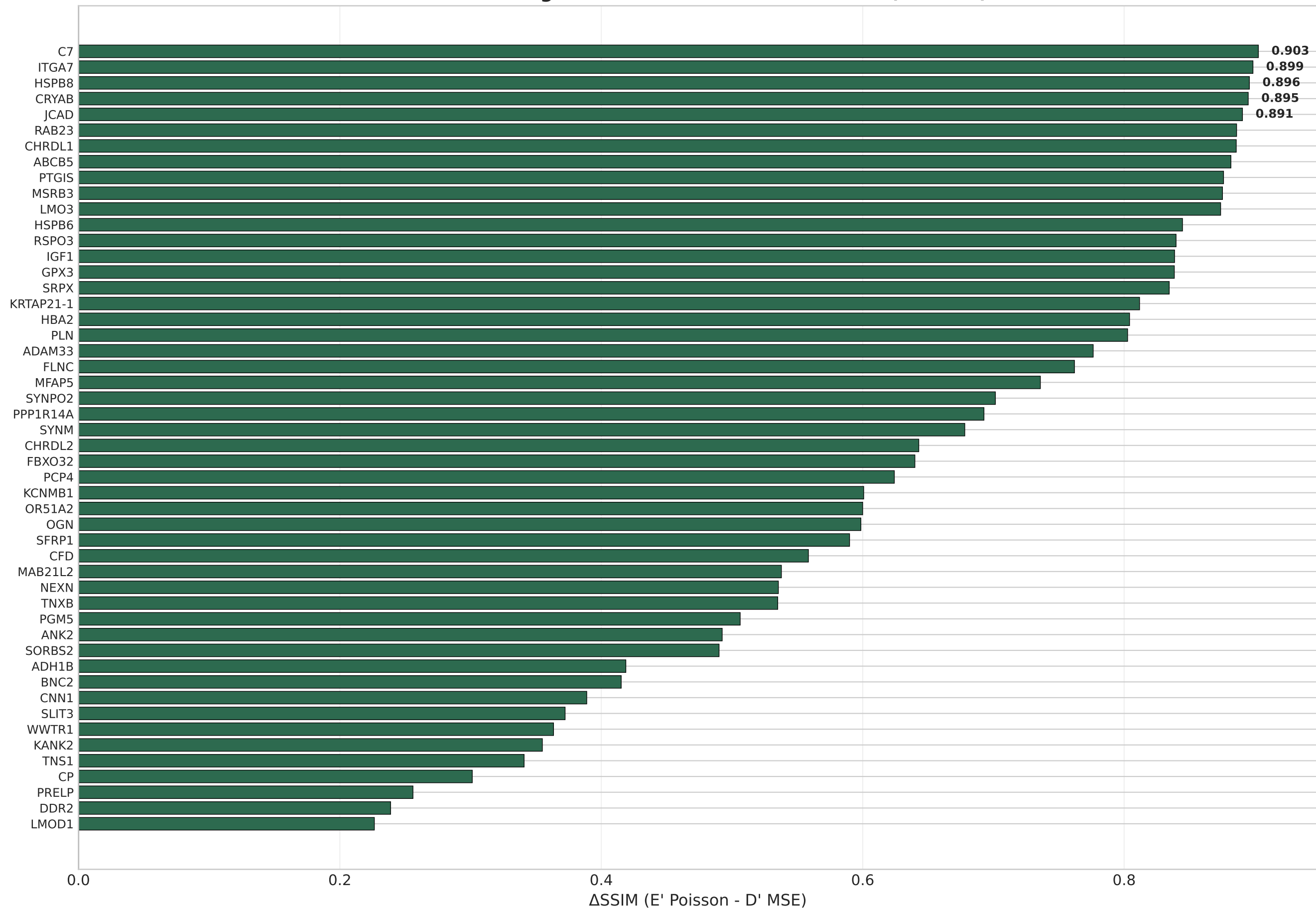
Gene Ranking: Poisson Benefit for Each Gene (Hist2ST)
