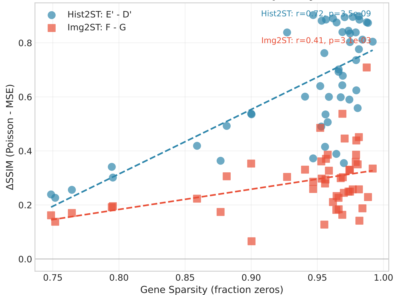
Poisson Benefit vs Gene Sparsity
