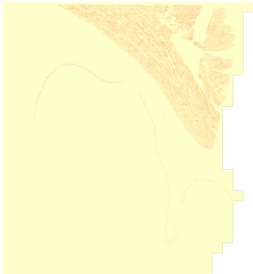
Ground Truth
