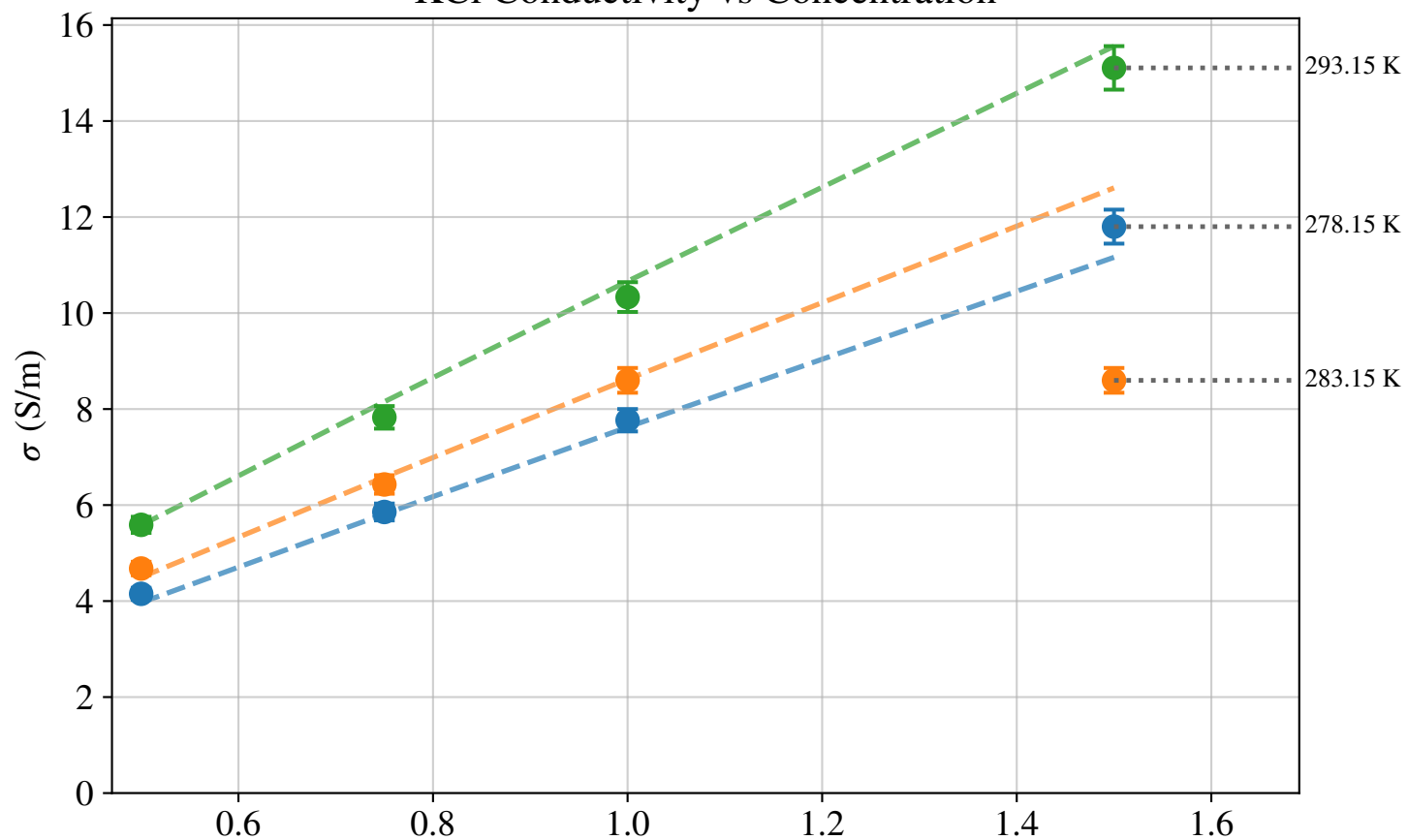
KCl Conductivity vs Concentration
