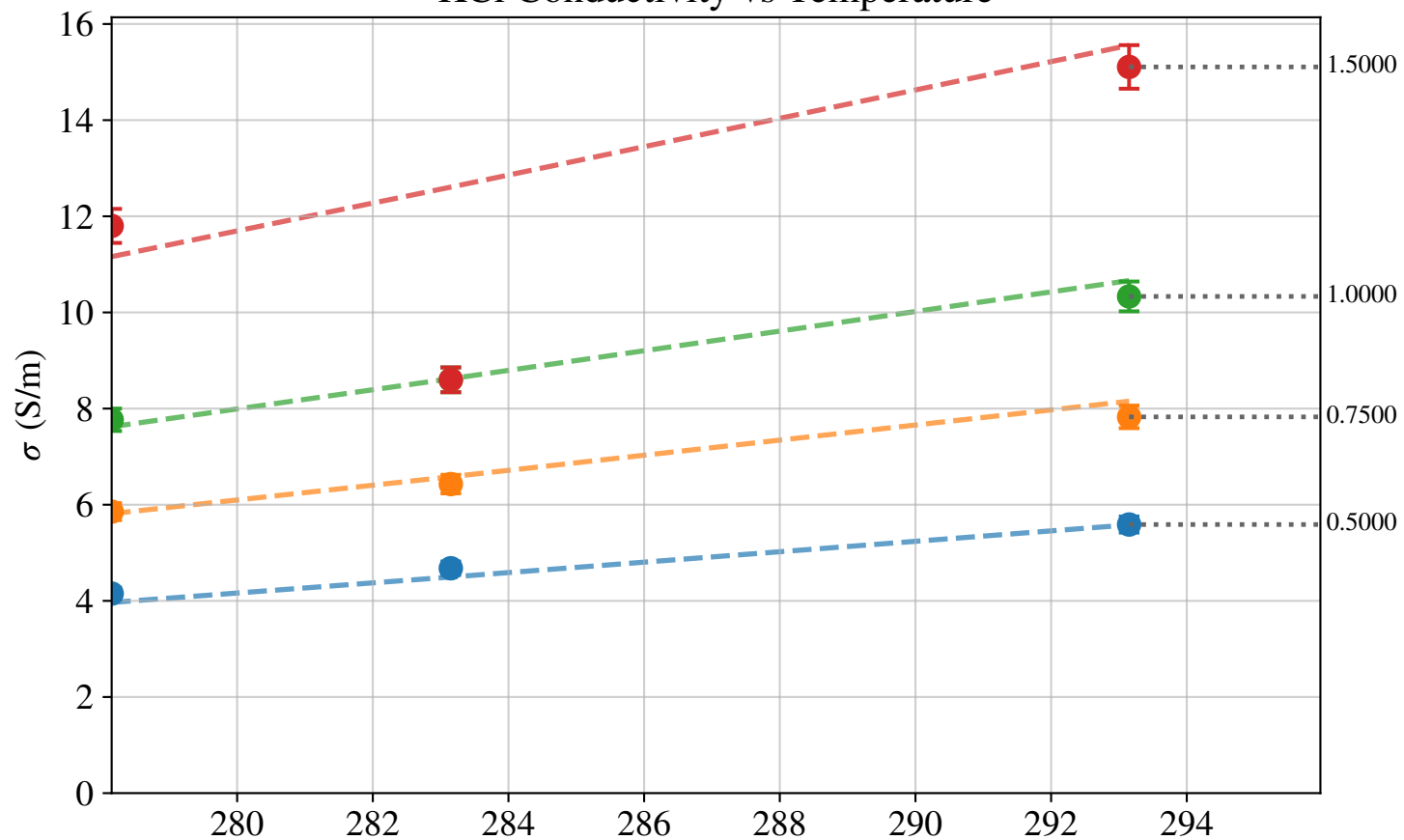
KCl Conductivity vs Temperature
