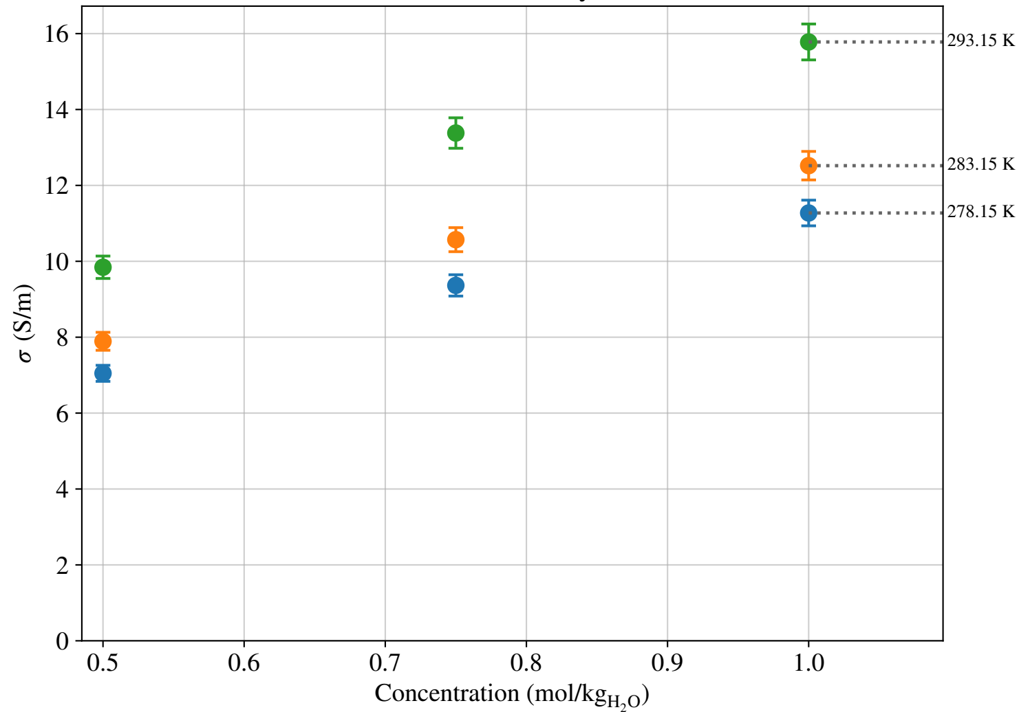
Na 2 SO 4 :KCl_1:1 Conductivity vs Concentration
