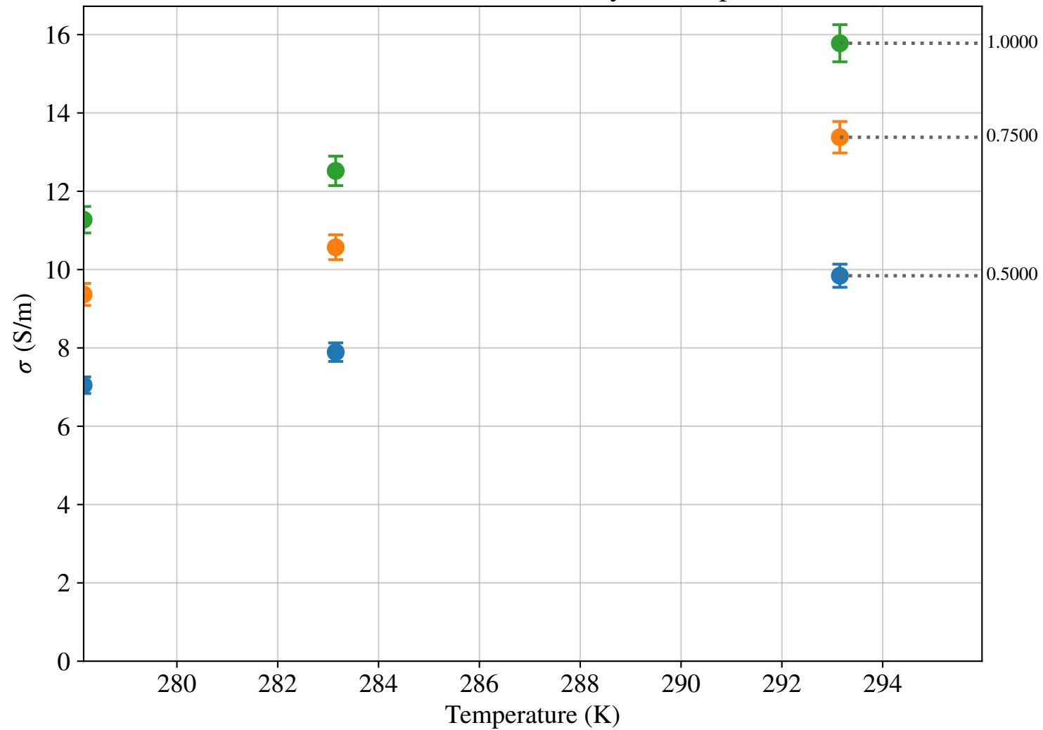
Na 2 SO 4 :KCl_1:1 Conductivity vs Temperature
