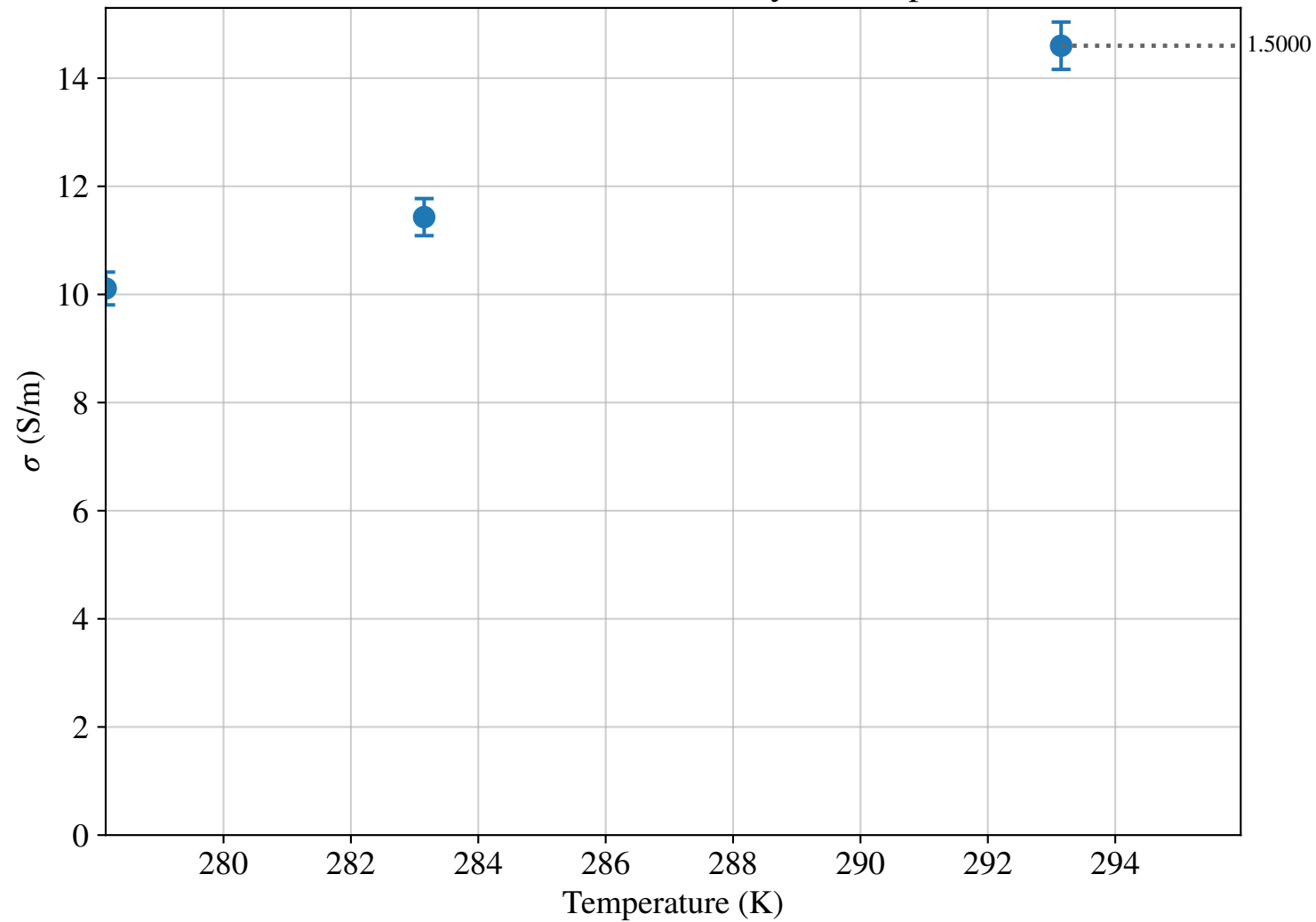
Na2SO4:KCl_2:1 Conductivity vs Temperature
