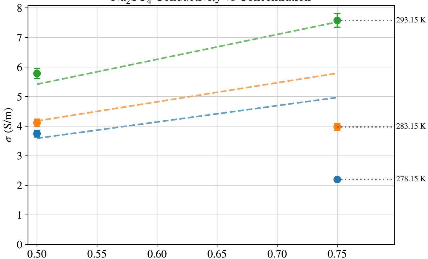
\text{Na}_2\text{SO}_4 Conductivity vs Concentration
