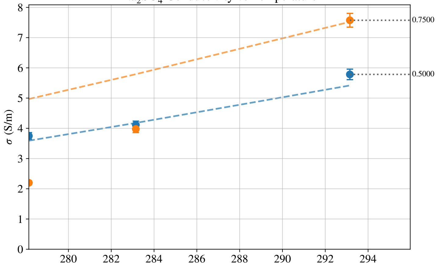
\text{Na}_2\text{SO}_4 Conductivity vs Temperature
