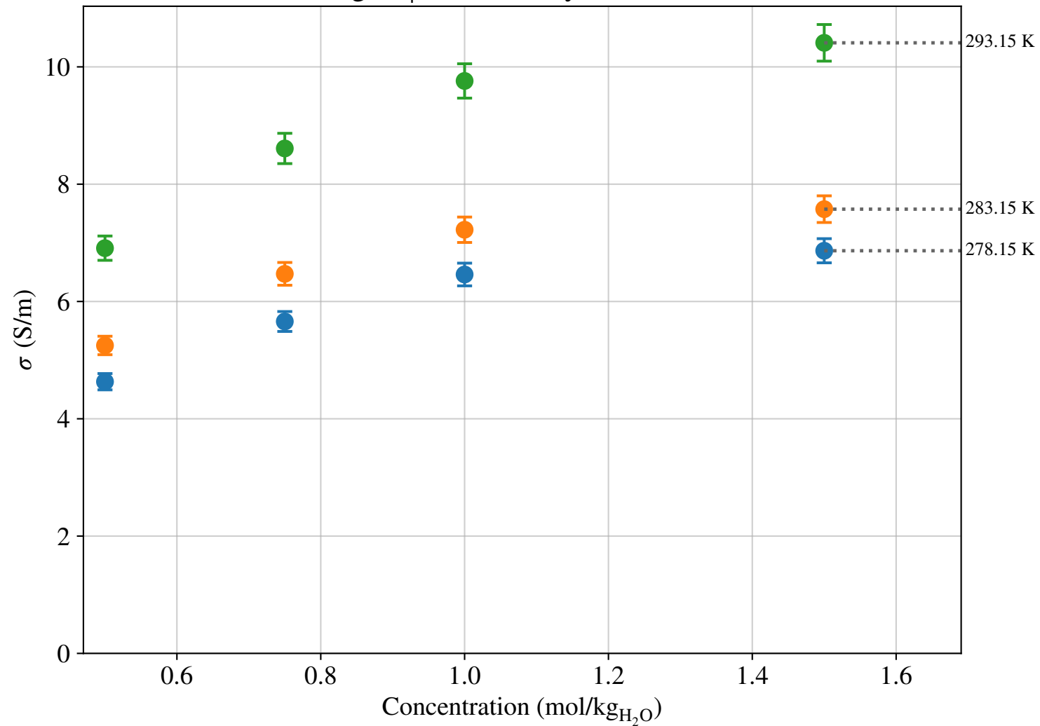
NaCl:MgSO 4 Conductivity vs Concentration
