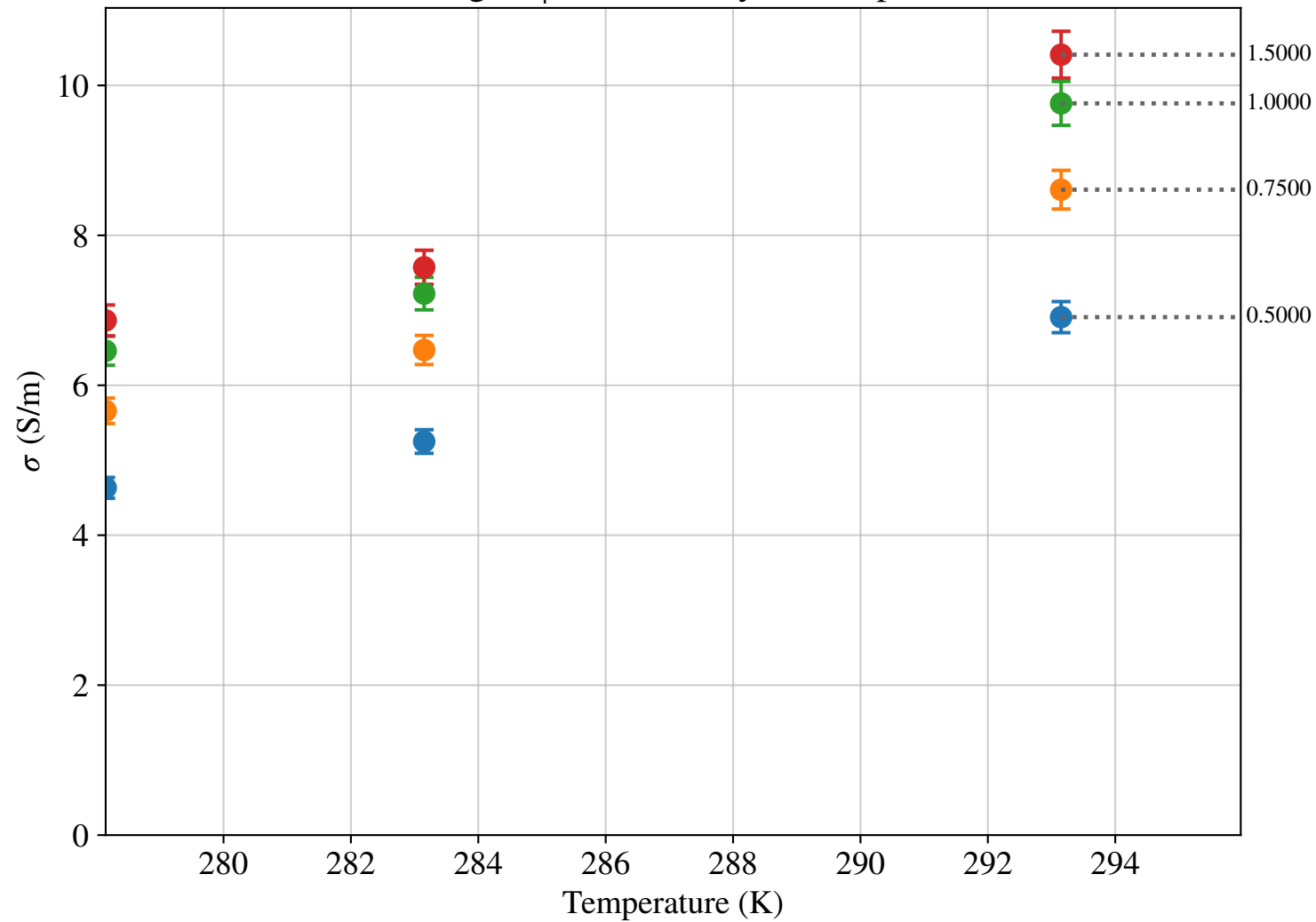
NaCl:MgSO 4 Conductivity vs Temperature
