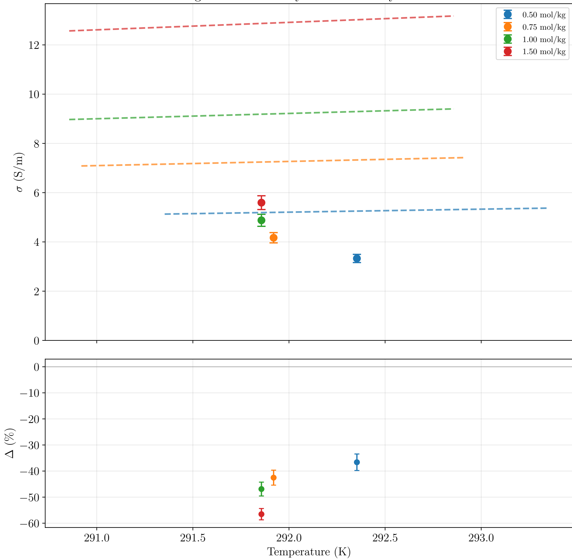
MgSO4 Conductivity with McCleskey Model
