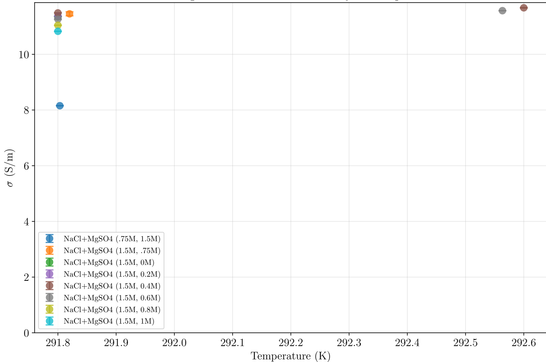
NaCl+MgSO4 Mixtures - Conductivity vs Temperature
