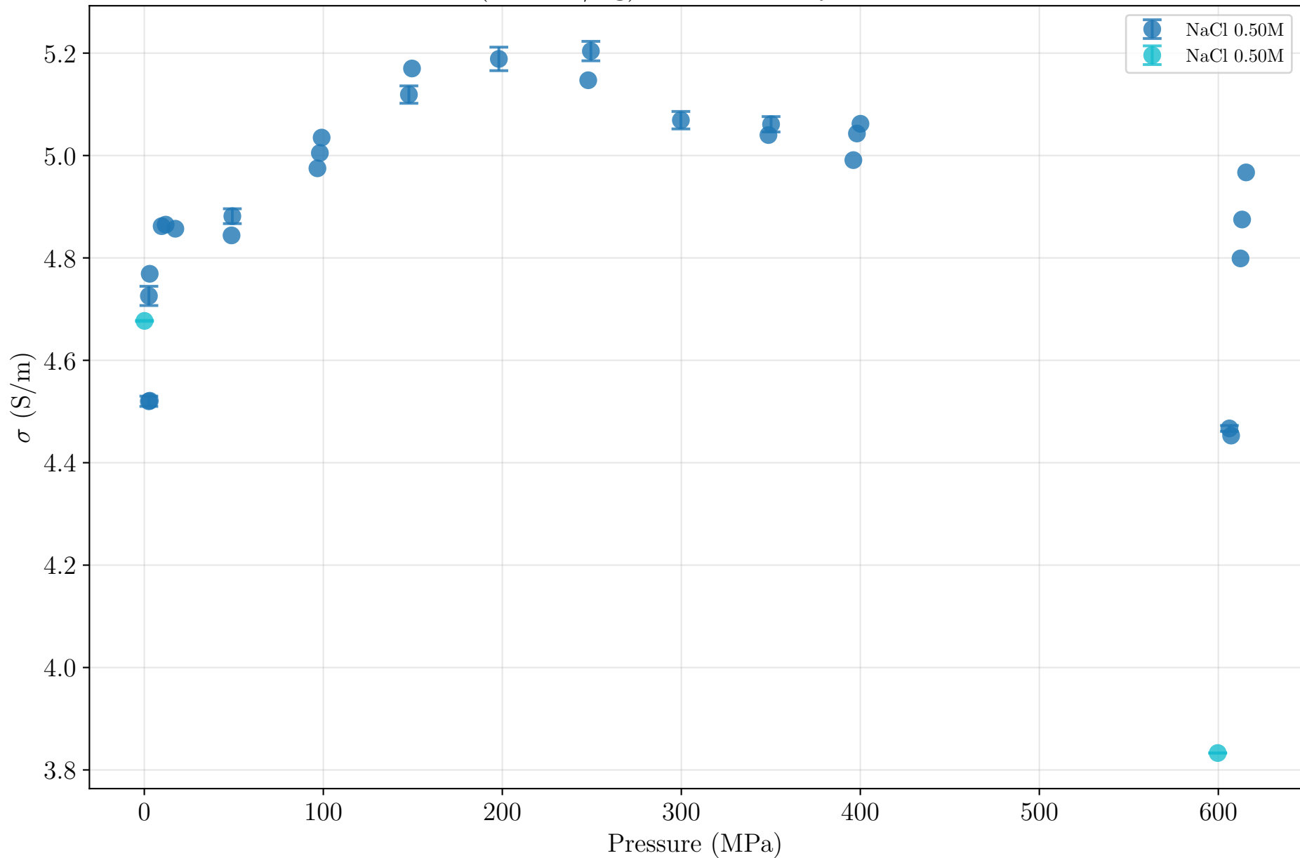
NaCl (0.5 mol/kg) - Conductivity vs Pressure
