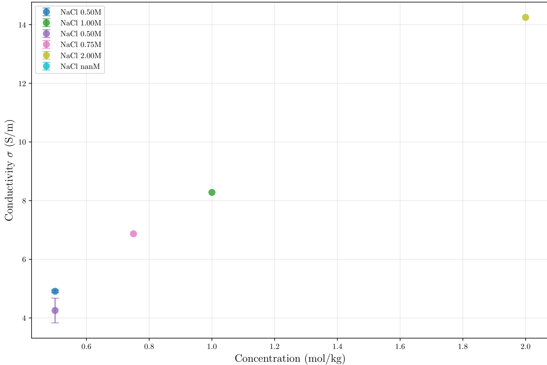
NaCl - Conductivity vs Concentration
