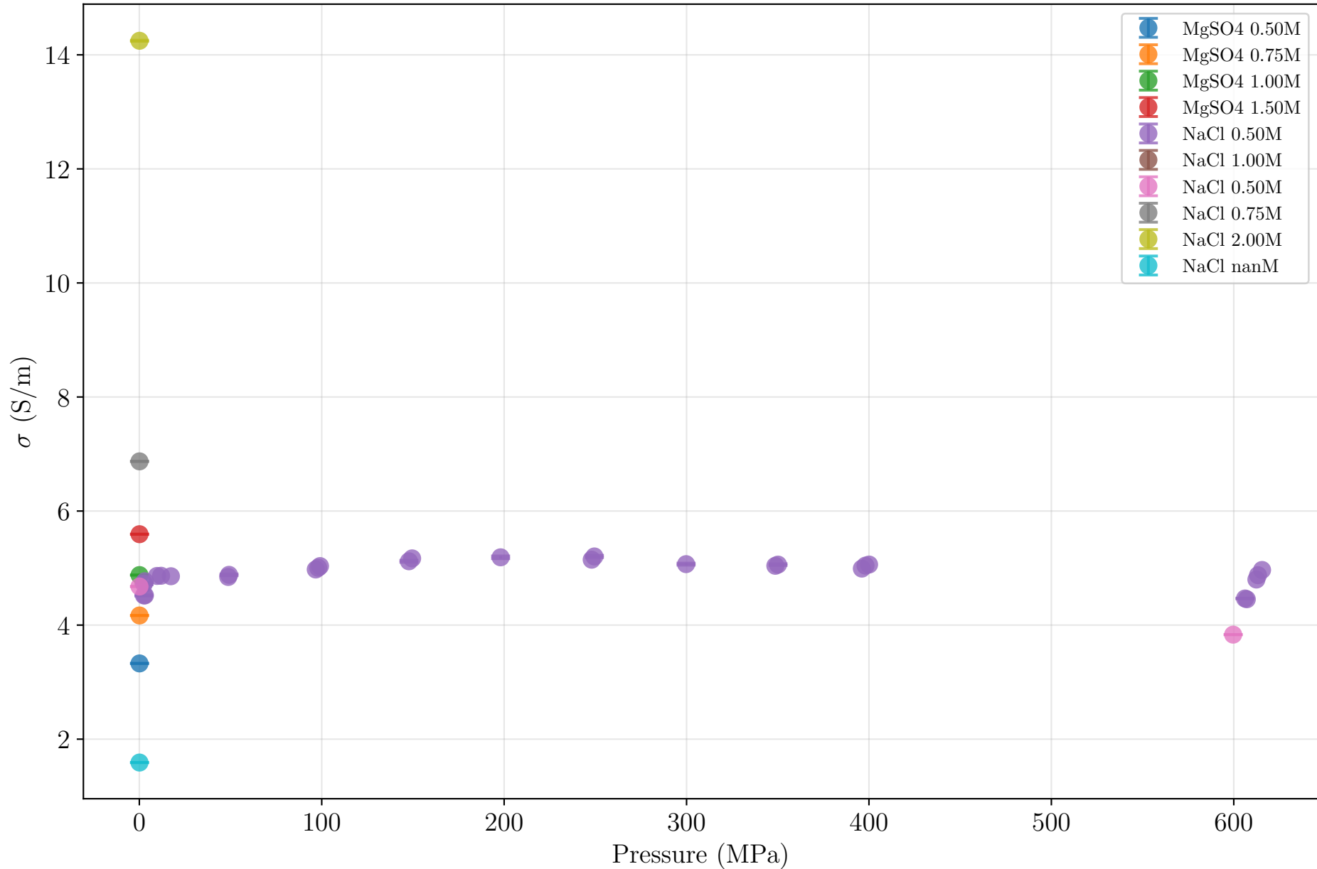
NaCl - Conductivity vs Pressure
