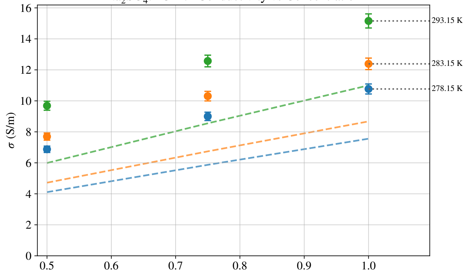
Na 2 SO 4 :KCl 1:1 Conductivity vs Concentration
