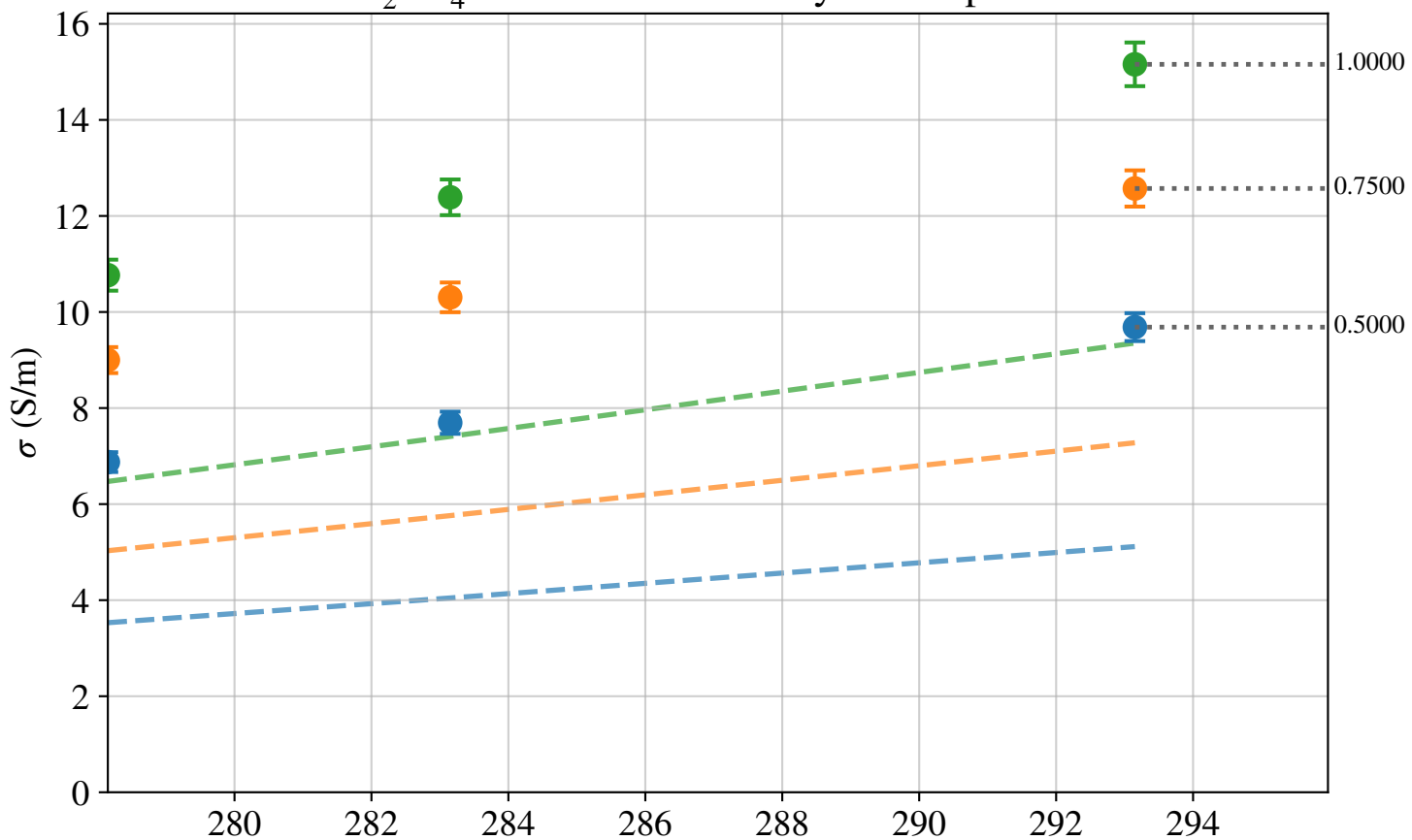
\text{Na}_2\text{SO}_4\text{:KCl} 1:1 Conductivity vs Temperature
