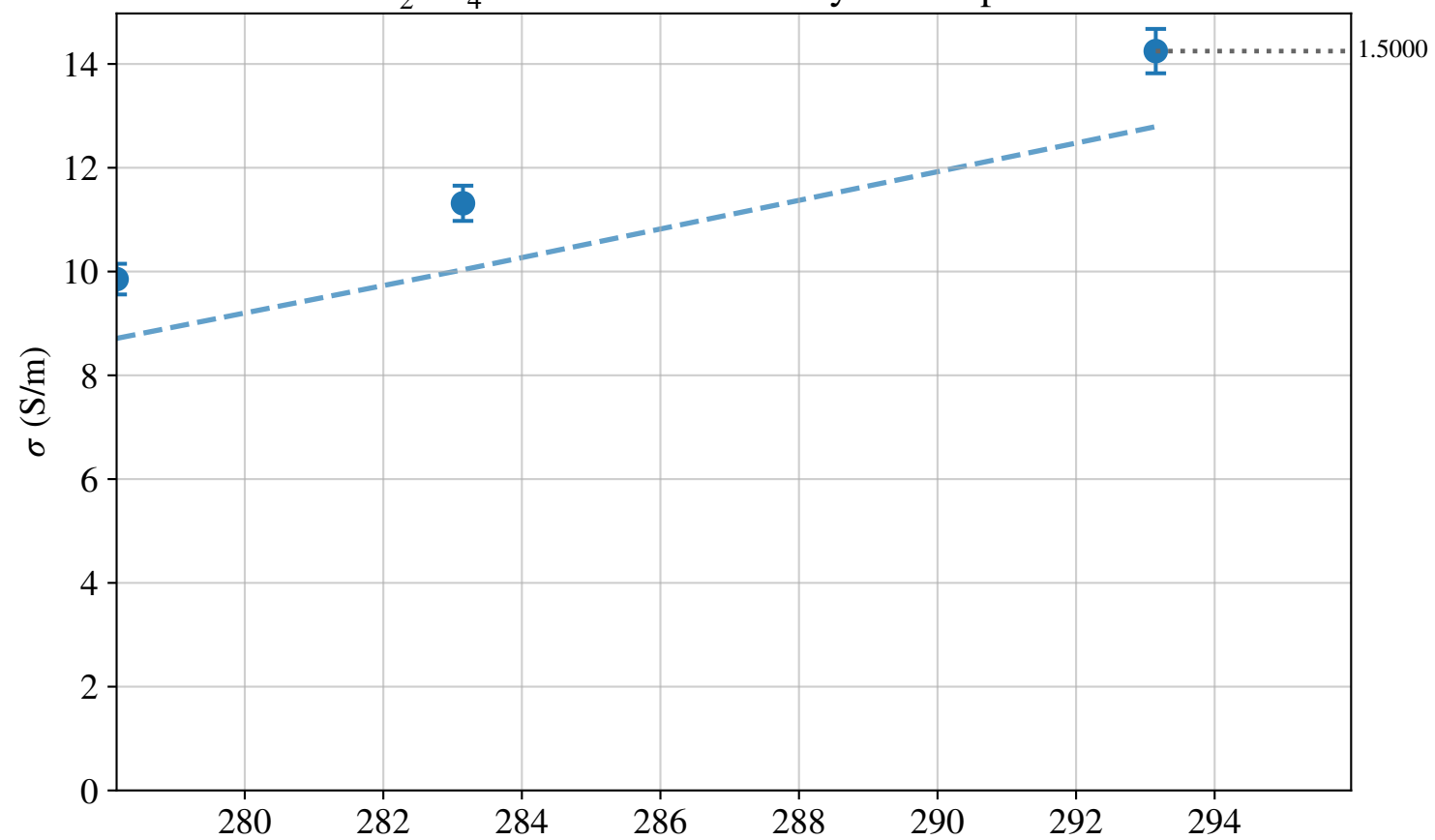
\text{Na}_2\text{SO}_4\text{:KCl} 2:1 Conductivity vs Temperature
