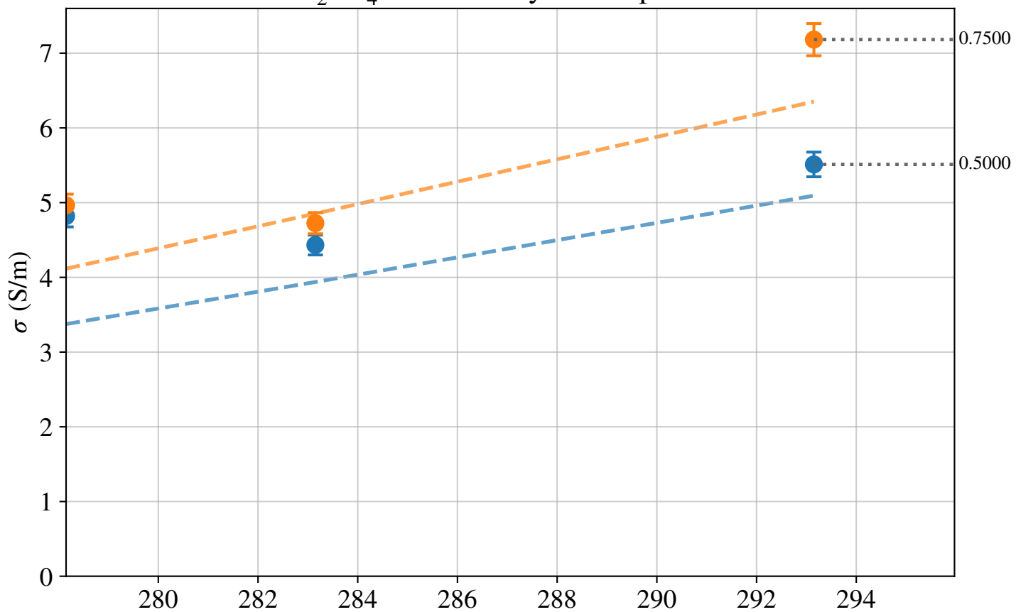
\text{Na}_2\text{SO}_4 Conductivity vs Temperature
