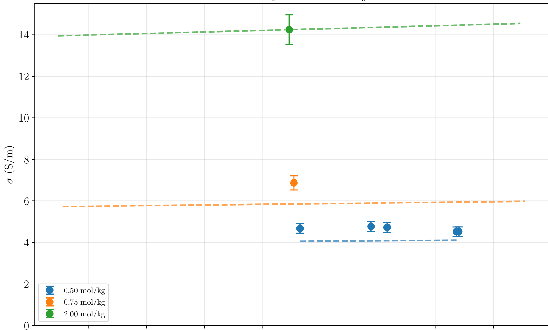
NaCl Conductivity with McCleskey Model
