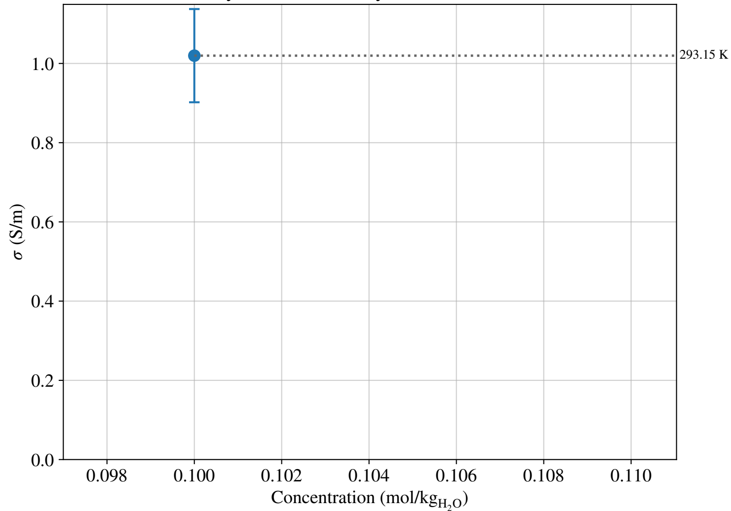
Glycine Conductivity vs Concentration
