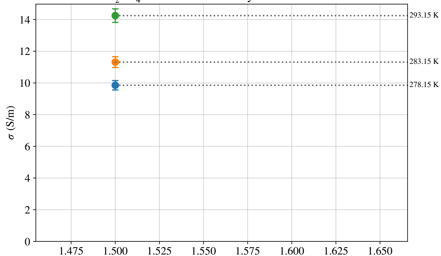
Na 2 SO 4 :KCl 2:1 Conductivity vs Concentration
