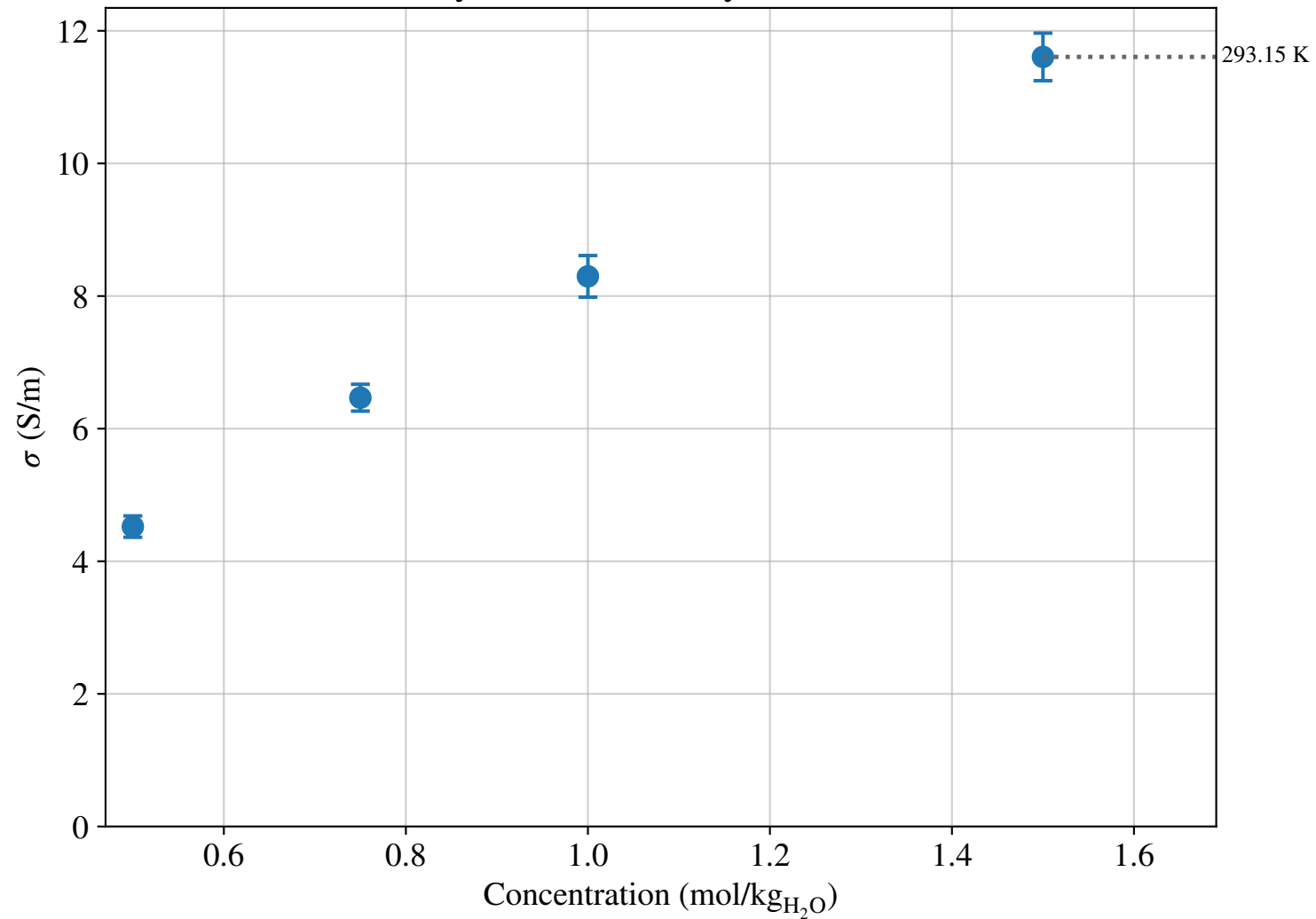
NaCl+Glycine Conductivity vs Concentration
