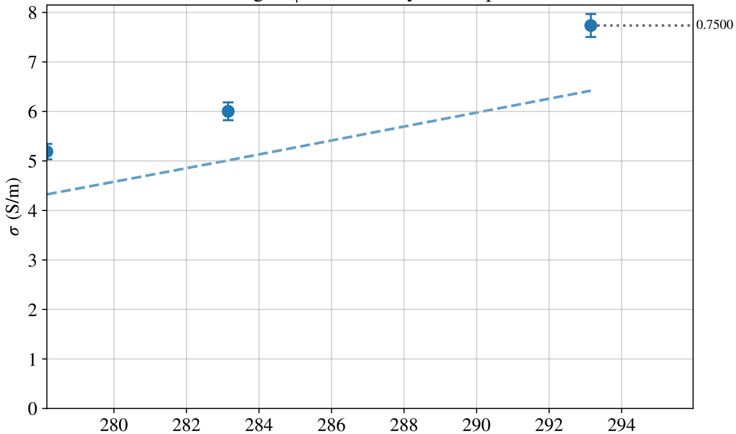
NaCl:MgSO 4 Conductivity vs Temperature
