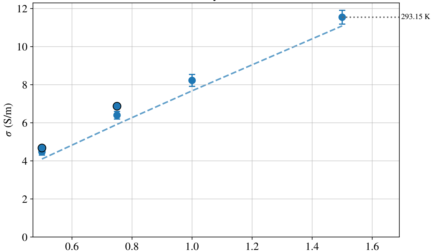
NaCl Conductivity vs Concentration
