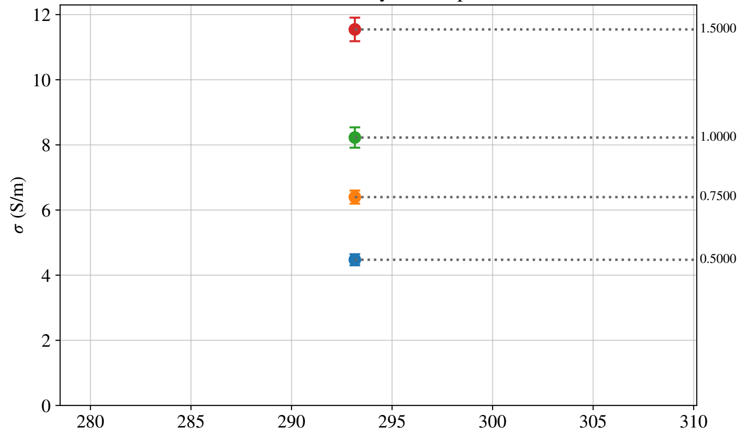
NaCl Conductivity vs Temperature
