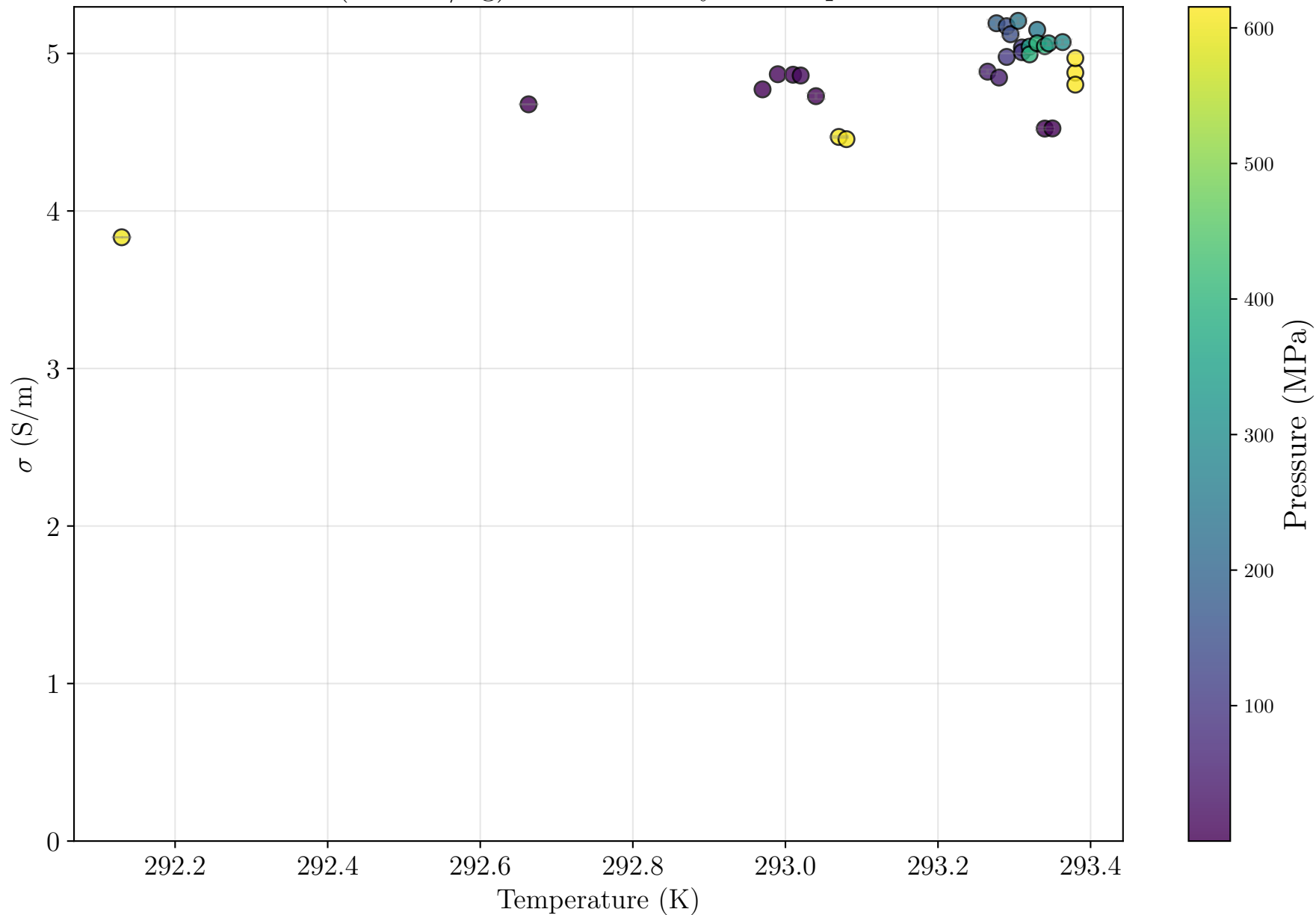
NaCl (0.5 mol/kg) - Conductivity vs Temperature
