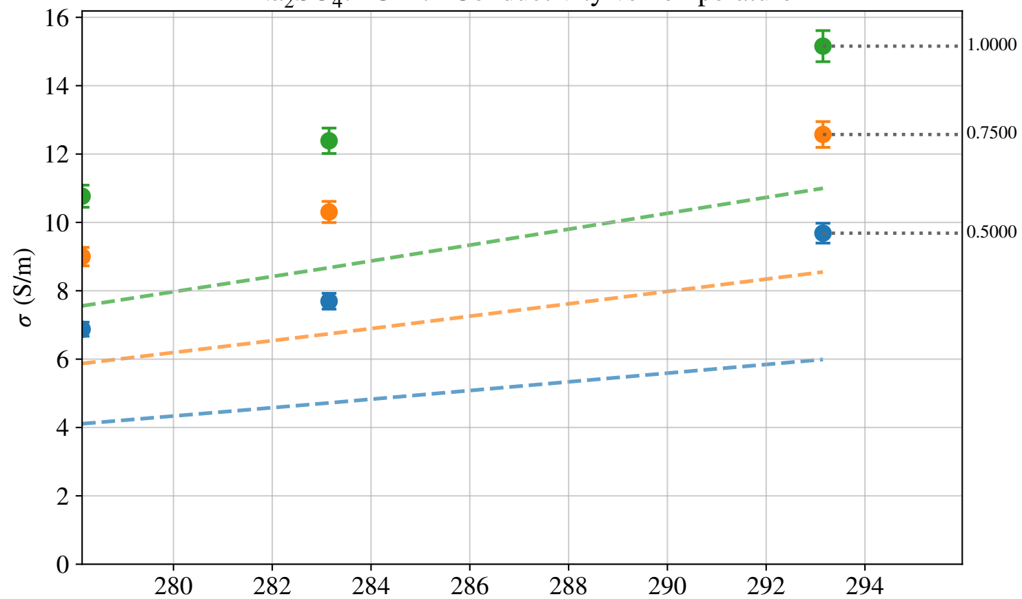
Na 2 SO 4 :KCl 1:1 Conductivity vs Temperature
