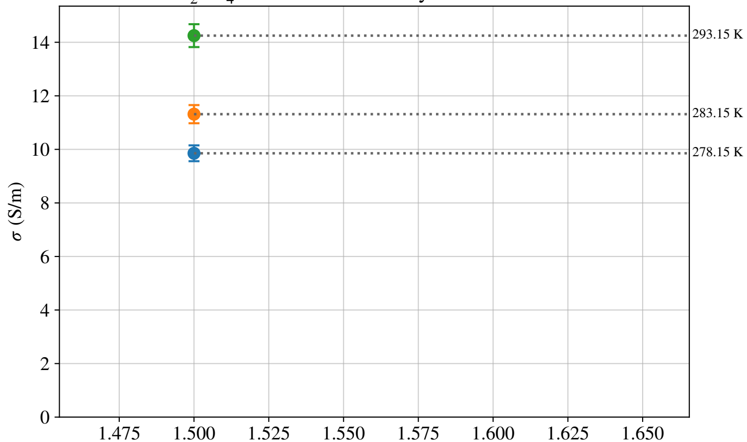
Na 2 SO 4 :KCl 2:1 Conductivity vs Concentration
