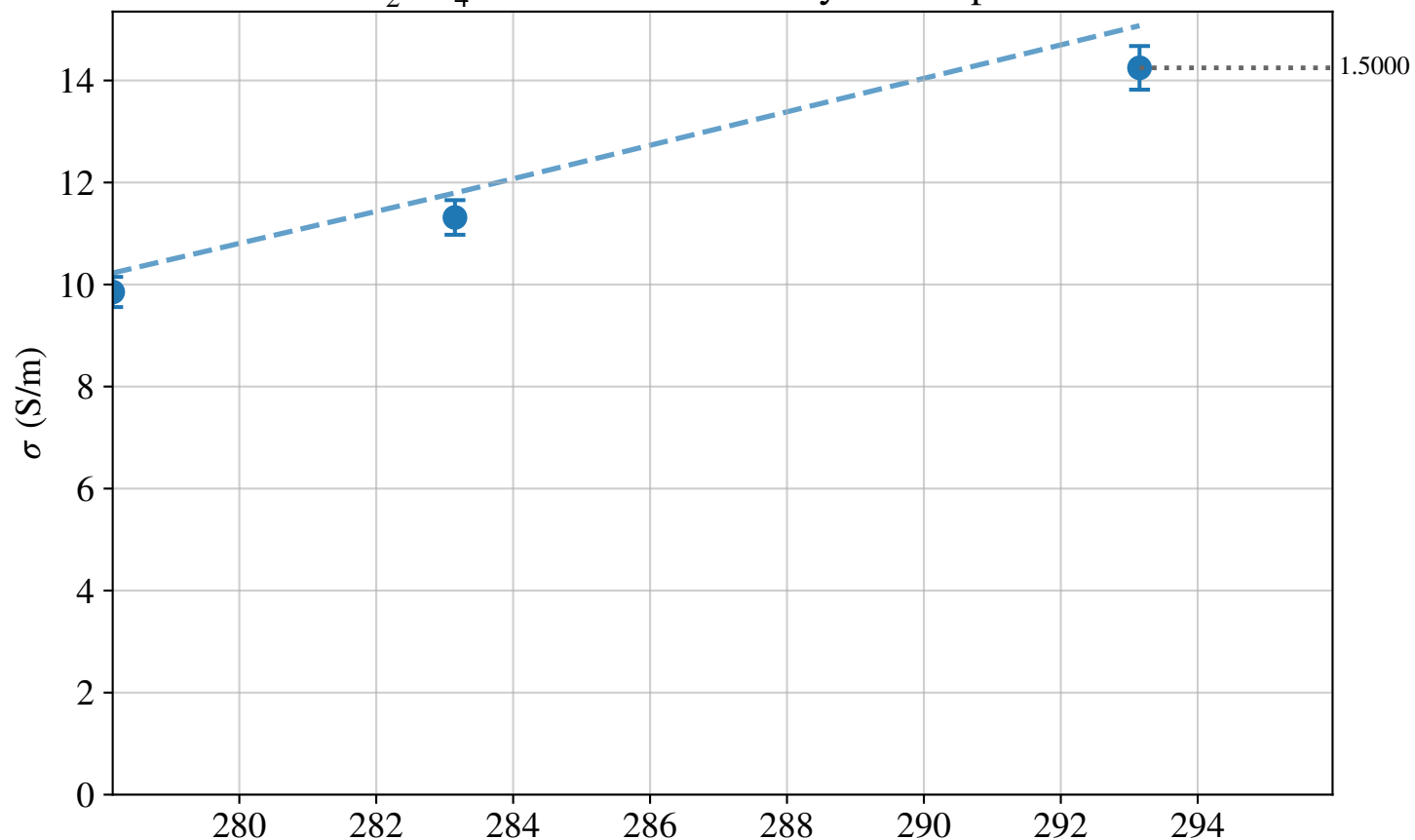
Na 2 SO 4 :KCl 2:1 Conductivity vs Temperature
