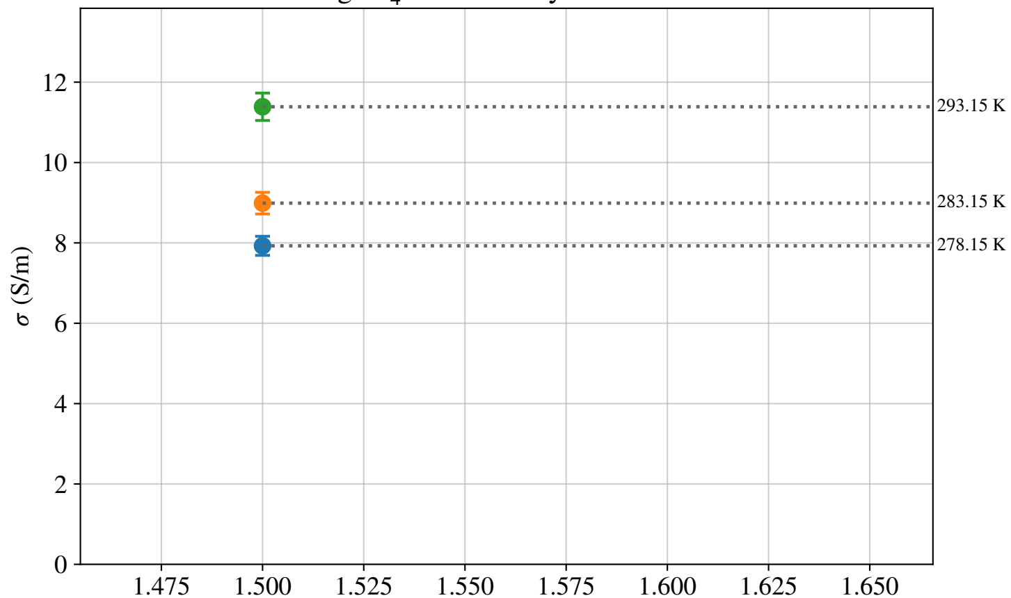
NaCl:MgSO 4 Conductivity vs Concentration
