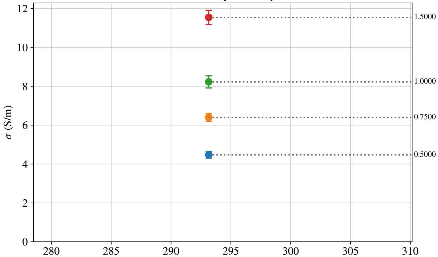
NaCl Conductivity vs Temperature
