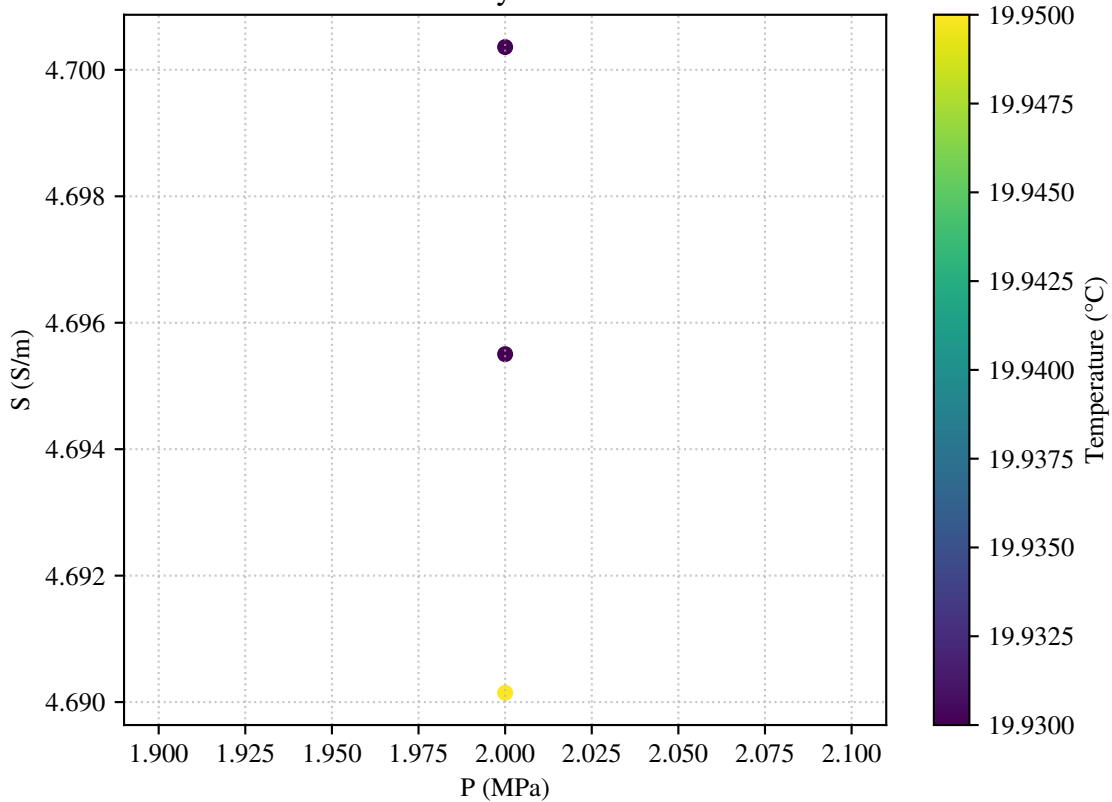
Conductivity vs Pressure
