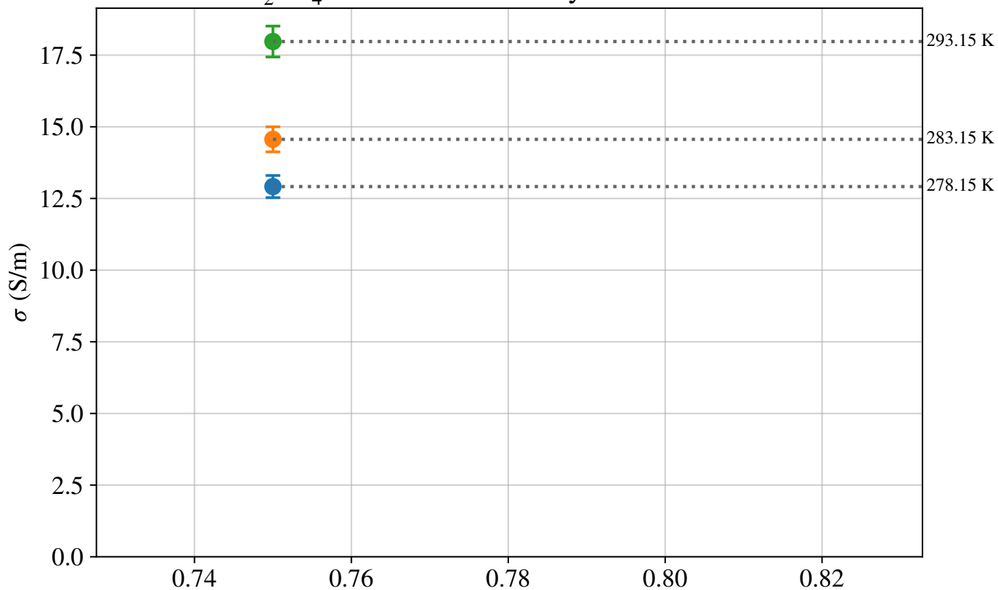
Na 2 SO 4 :KCl 1:2 Conductivity vs Concentration
