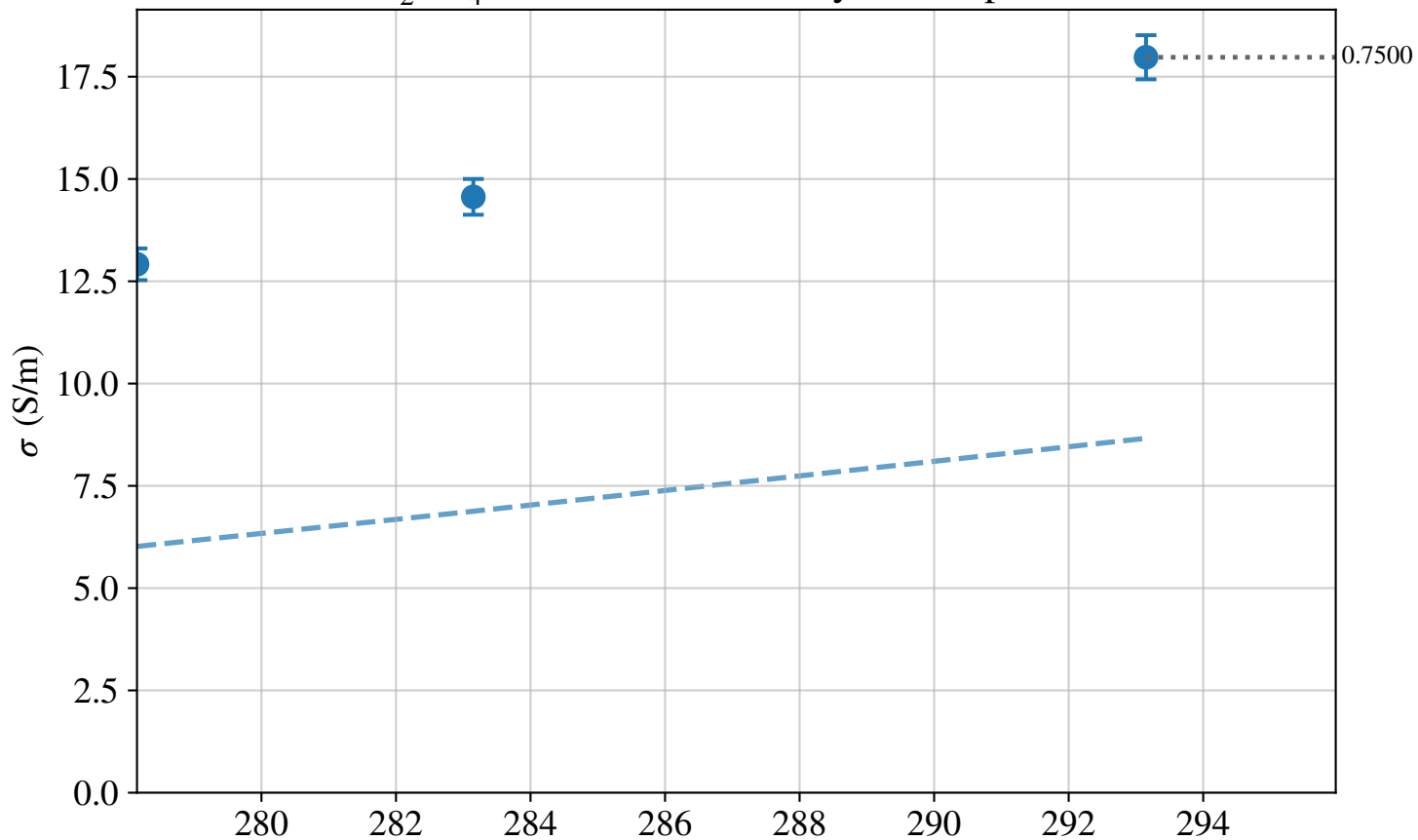
Na 2 SO 4 :KCl 1:2 Conductivity vs Temperature
