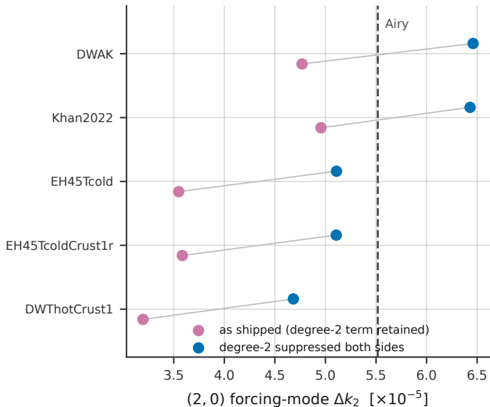
InSight-calibrated crustal models vs Airy
