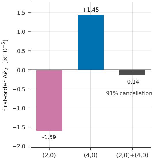
Two first-order zonal channels, opposite signs
