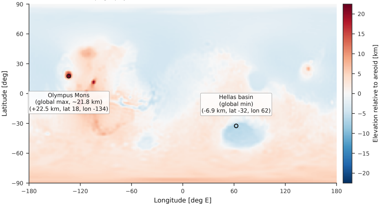
MOLA topography (relative to areoid), \ell_{\max} = 90 , C00+C20 removed
