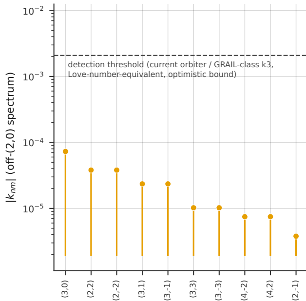
Off-(2,0) coupled spectrum (top 10 of 114)
