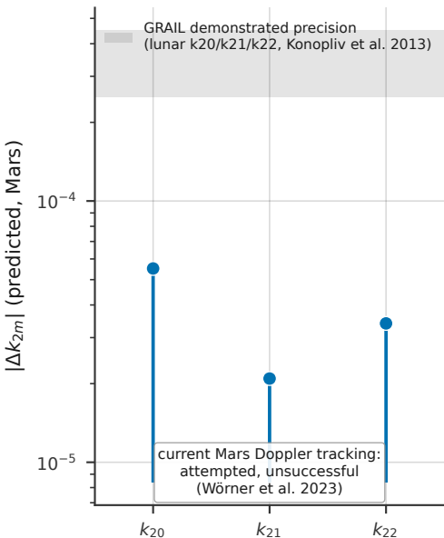
Diagonal k_{2m} order-splitting
